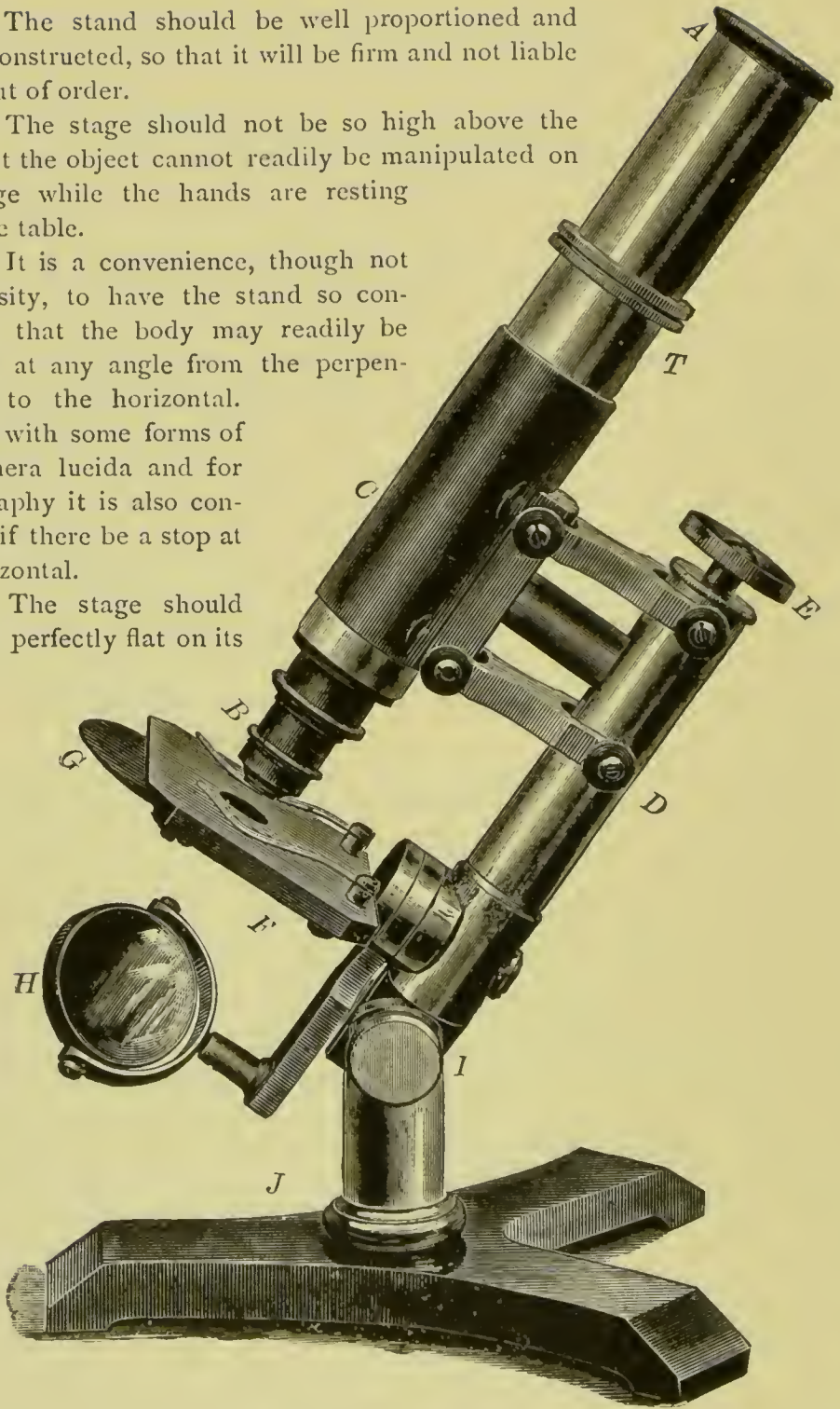
FIG. 460.— A , Eye-piece. B , The objective. C , The sleeve. D , Arm supporting the sleeve and tube. E , The "fine adjustment," operated by a screw, for obtaining the exact focus. F , The stage, with a pair of spring clips to hold the object or slide. G , A revolving diaphragm, with perforations of various sizes to regulate the amount of light admitted to the objective. H , A concave mirror on an axis, which permits illumination of any obliquity beneath the stage. It swings on an arm, by which it may be brought above the stage for the illumination of opaque objects. The instrument, complete without the objective, is called the "stand."
