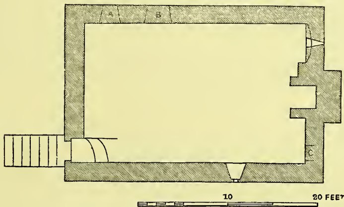
GROUND PLAN OF UPPER STORY IN THE NORTH HOUSE, CARSWELL.*
