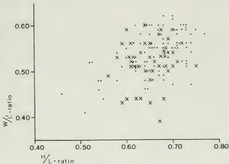
Text-fig. 2b. Diagram of ratios W/L' vs. H/L for Carbonita humilis from G. B. 25 Band. . specimens with rounded dorsum x specimens with straightened dorsum
