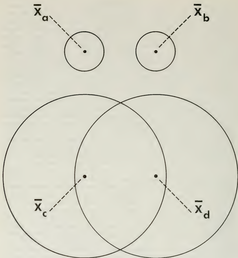
Text-figure 1. Diagrammatic representation of two studies of two populations each. Members of populations a and b with no overlap in morphologic characters are easily discriminated; members of populations c and d with a great deal of overlap are difficult to discriminate. Means of populations indicated by \bar{X} .
