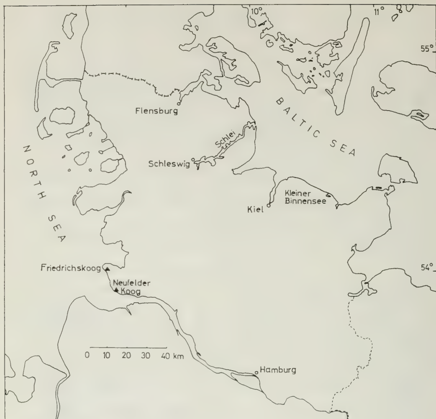
Text-figure 1. Study areas in Schleswig-Holstein.
