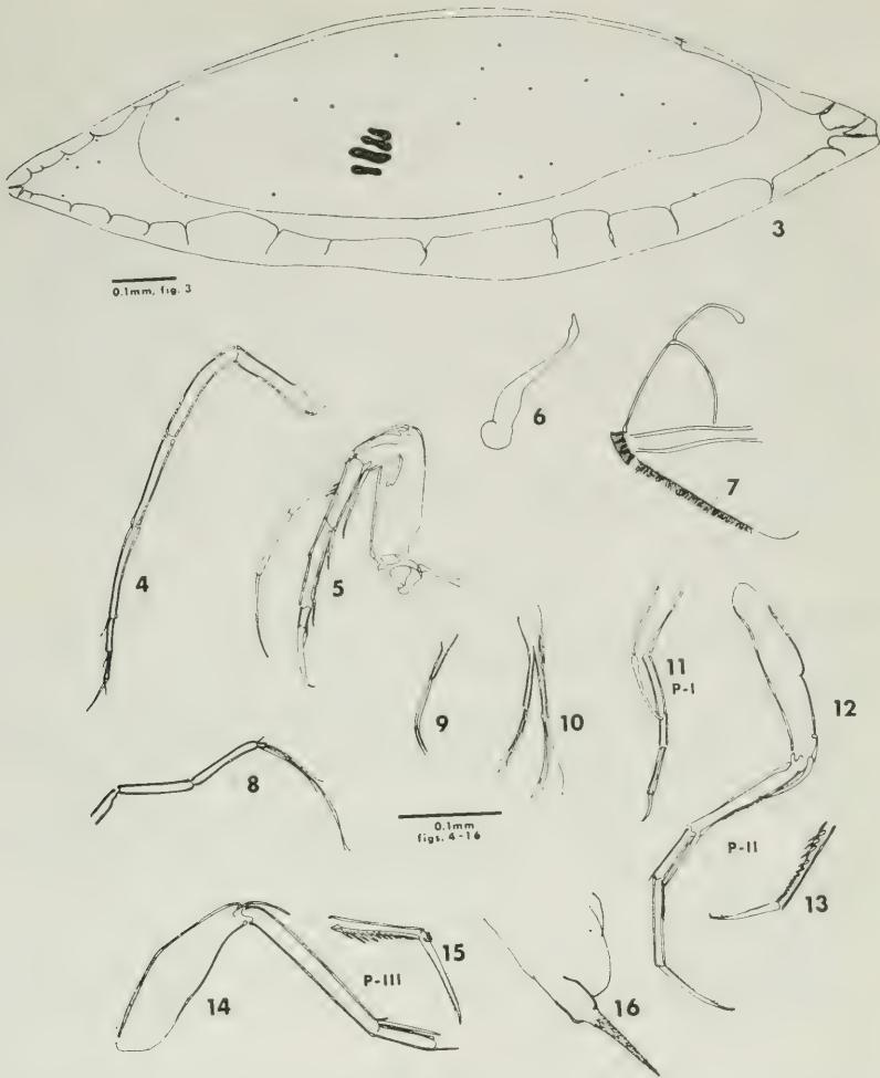
Text-figures 3-16.—Carapace of female. 4. Antennule. 5. Antennal endopod. 6. Antennal gland. 7. Oral cone. 8. Mandible palp. 9, 10. Maxillule palp. 11-15. Thoracic limbs. 16. Posterior portion of body.
