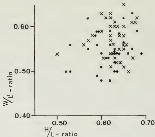
Text-fig. 5b. Diagram of ratios W/L' vs. H/L for Carbonita humilis from foveolata Band. . specimens with maximum width median x specimens with maximum width posterior
