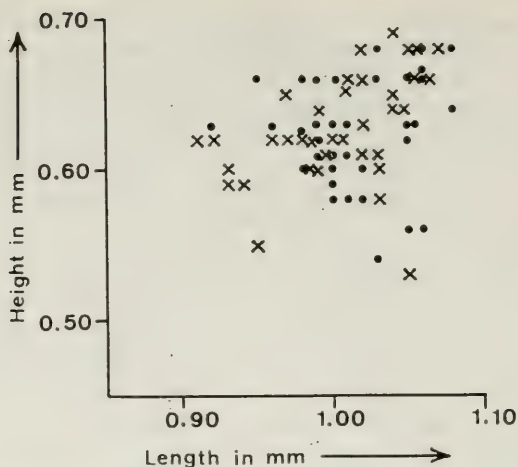
Text-fig. 5a. Height vs. length diagram for Carbonita humilis from foveolata Band. . specimens with maximum width median x specimens with maximum width posterior
