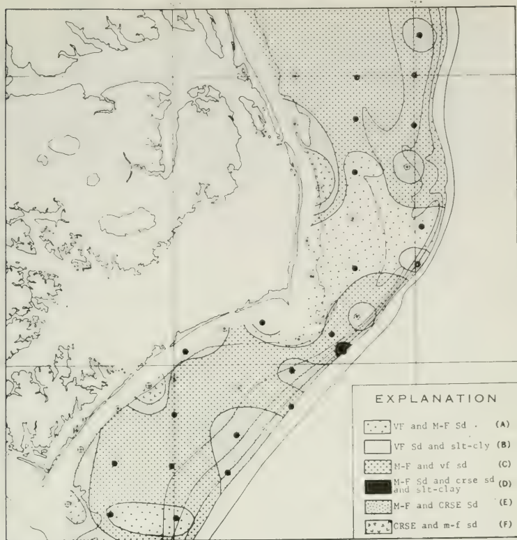
Text-figure 5.—Bottom-sediment facies map based on major clusters (A-F) of figure 4. The capital and lower case letters in the explanation indicate the dominant and subordinate grain size classes, respectively. A more detailed breakdown of sediment composition can be found in Hathaway (1971); see also Milliman (1972). Sample stations explained in figure 1.
