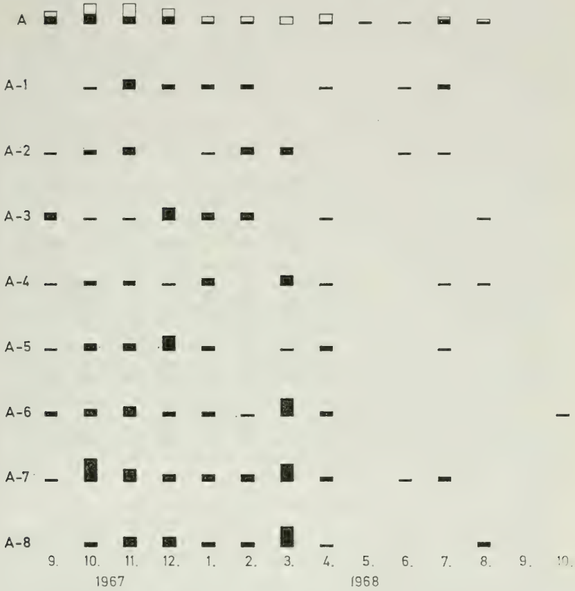
Text-figure 2. Cytherella sp. Seasonal distribution of instars, females, and males on the basis of 215 living specimens.
