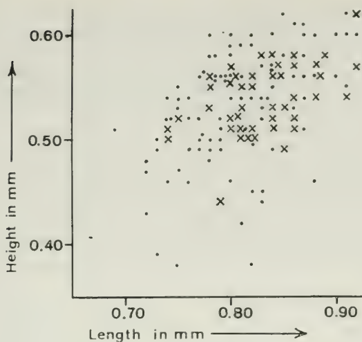
Text-fig. 2a. Height vs. length diagram for Carbonita humilis from G. B. 25 Band. . specimens with rounded dorsum x specimens with straightened dorsum
