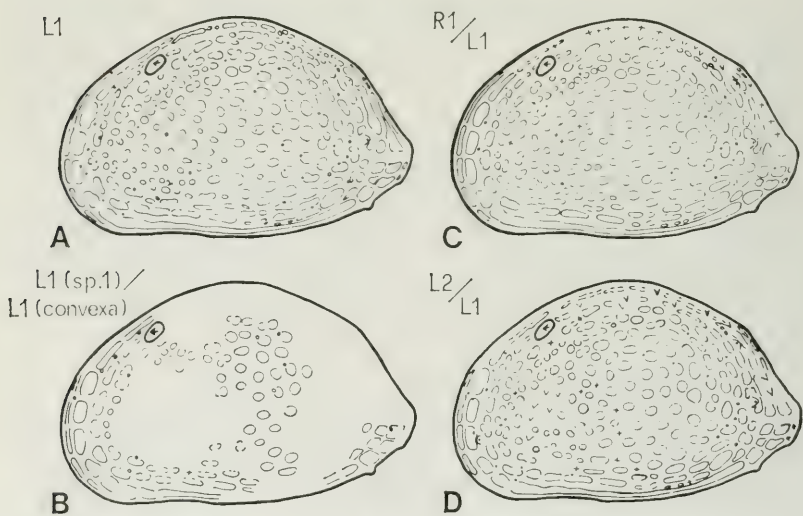
Text-fig. 4. Aurila convexa , Recent, Portuguese coast. Scale: Length of the L1 0.76 mm.
