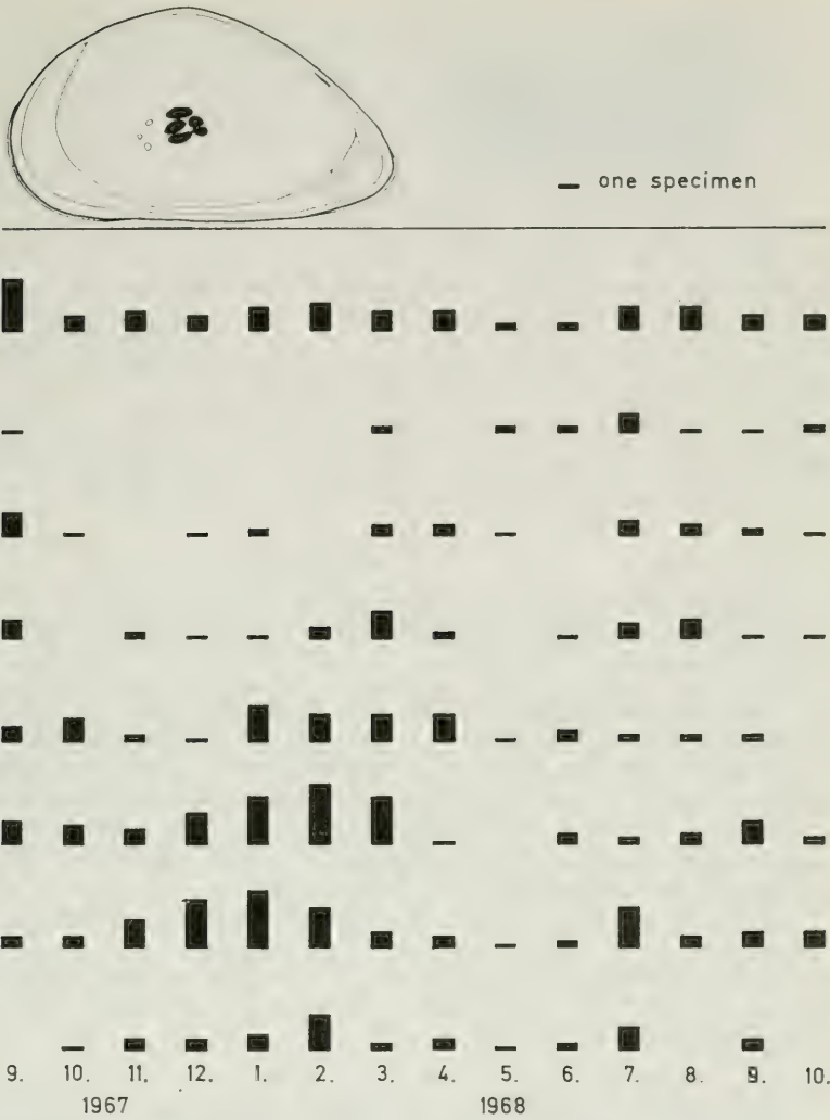
Text-figure 3. Proponocypris setosa (G. W. Müller, 1894). Seasonal distribution of instars on the basis of 398 living specimens.
