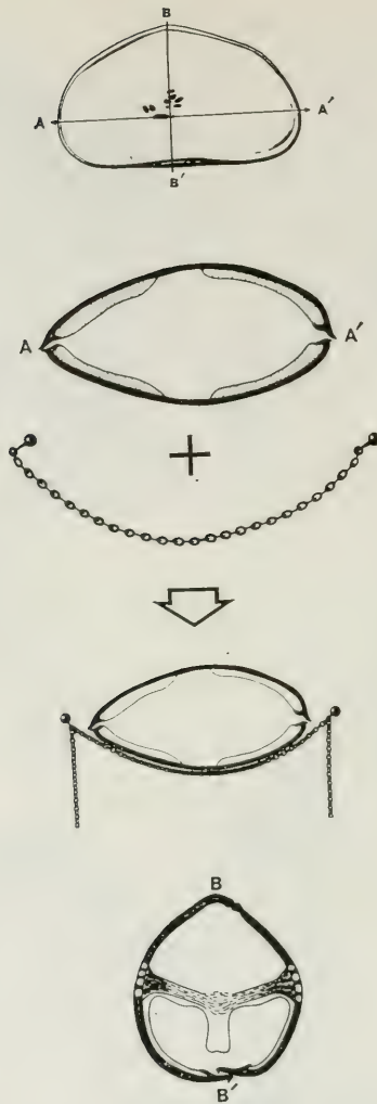
Text-figure 21. Longitudinal and saggital sections of Potamocypris? steueri Klie, 1935 (taken from Gauthier, 1939) showing a comparison between the catenary form of a spanning chain in tensional stress equilibrium (the equal and opposite of compressional span stress equilibrium) and the longitudinal shape of the carapace. The lower illustration of the chain and section together is an actual high contrast photograph of the experiment. The fit is better than 90 percent with the ends departing from the catenary form, presumably under the influence of local increased thickness to resist bending near the edge and the presence of the infold ( duplicature sensu lato ).
