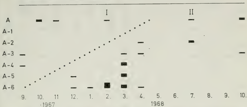
Text-figure 9. Cytheridea neapolitana Kollmann, 1960. Seasonal distribution of instars on the basis of 33 living specimens. The dotted line indicates the border between generation I and generation II.
