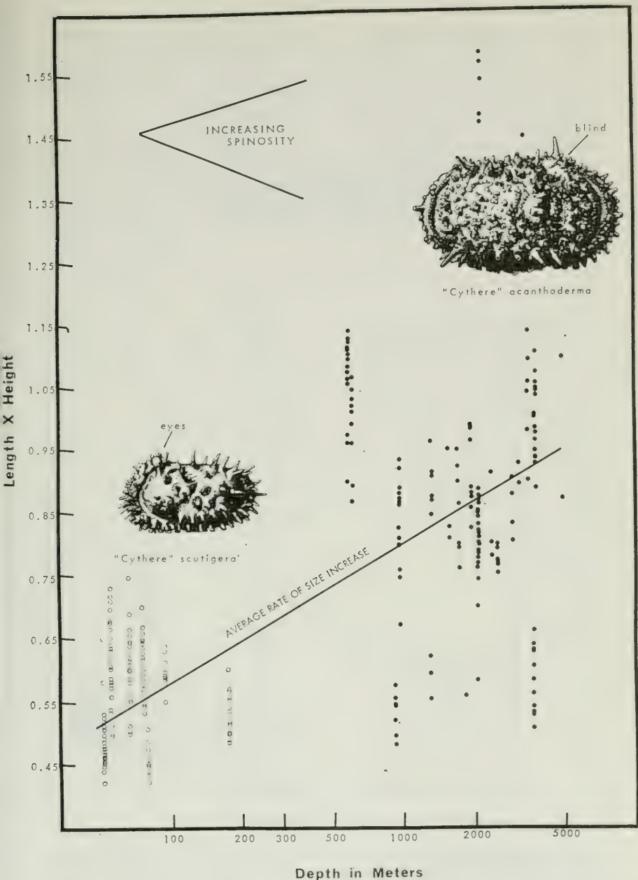
Text-figure 12. Increase in average size (in mm) and spinosity with depth of end members of a series of trachyleberid species including "Cythere" scutigera Brady, 1868, and "Cythere" acanthoderma Brady, 1880.
