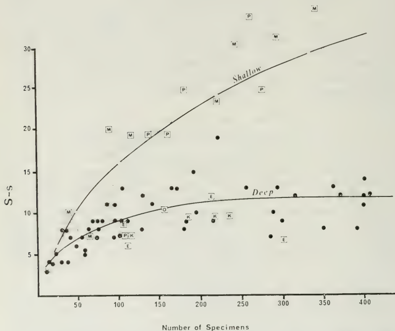
Text-figure 22. Relative species diversity among samples collected from the deep-sea (depths greater than 1000 meters; dots) and samples collected on the shelf (depths generally between 10 and 200 meters). Fossil samples of the same depths are also indicated (squares) with the ages shown (K, Cretaceous; E, Eocene; M, Miocene; P, Pliocene). The species diversity ( S-s is total species minus species with only one specimen found in a sample) of deep-sea psychrospheric faunas seems to have remained about half of that of temperate shelf faunas over the last 20 million years or perhaps longer.
