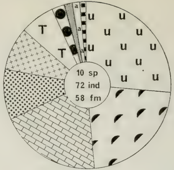
Spitzbergen Römer & Schaudinn Station 6 Adults Only
