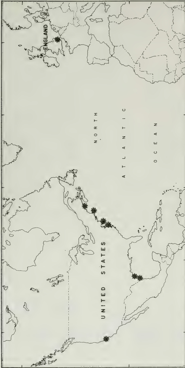
Text-figure 2. Map showing distribution of S. zostericola .
