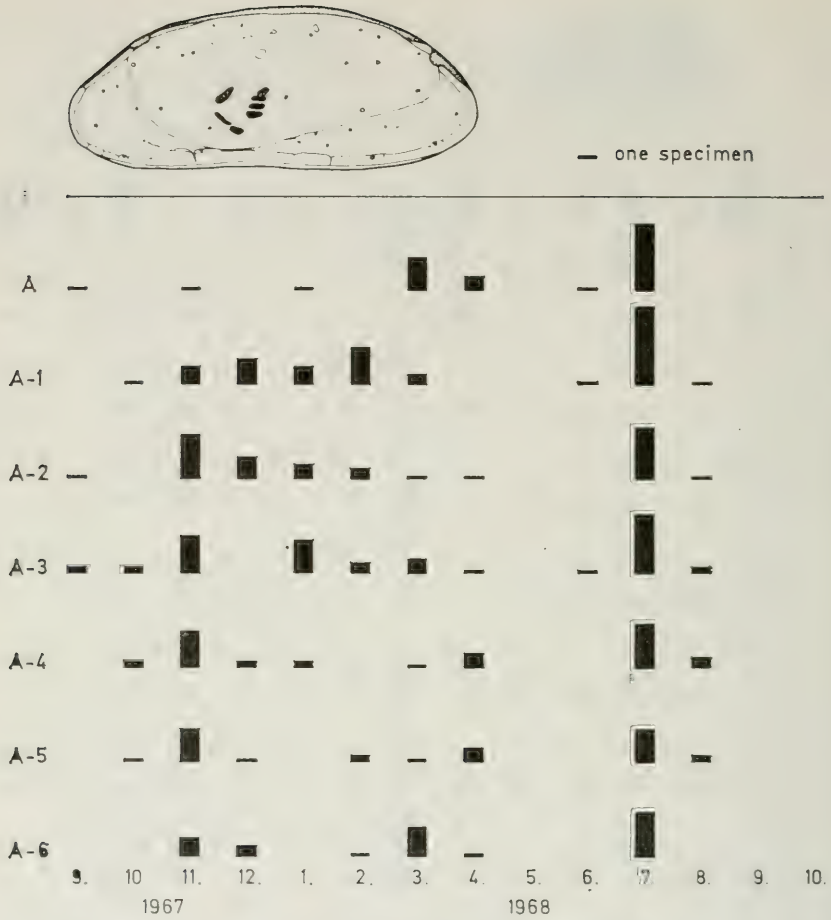
Text-figure 13. Cytheroidea aff. C. fischeri (Sars, 1866). Seasonal distribution of instars on the basis of 277 living specimens.
