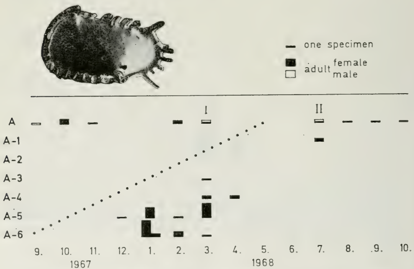
Text-figure 8. Pterygocythereis jonesii (Baird, 1850). Seasonal distribution of instars, females, and males on the basis of 52 living specimens. For dotted line see explanation Text-figure 7.
