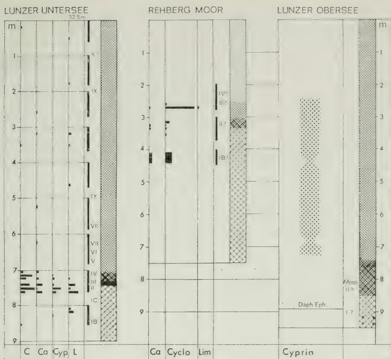
Text-fig. 1. — Distribution of ostracodes in cores from Lunzer Untersee, left, columns representing (left to right) Cytherissa , Candona candida , Cypria , and Limnocythere sanctipatricii . Breadth of each column: 20 shells. Black bars: actual cores taken. Symbols of sediments, presented right of the former, see Text-fig. 2. Rehberg Moor: Columns representing (left to right) Candona candida , Cyclocypris , Limnocythere sanctipatricii . Lunzer Obersee: schematic presentation of the distribution of Cypria , from 0-2.5 m not investigated but present.
