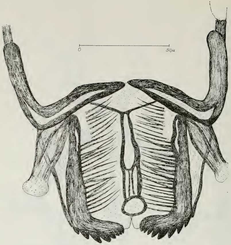
Text-figure 7. — Heterocypris salina (Brady), 1862) — Lower lip.
