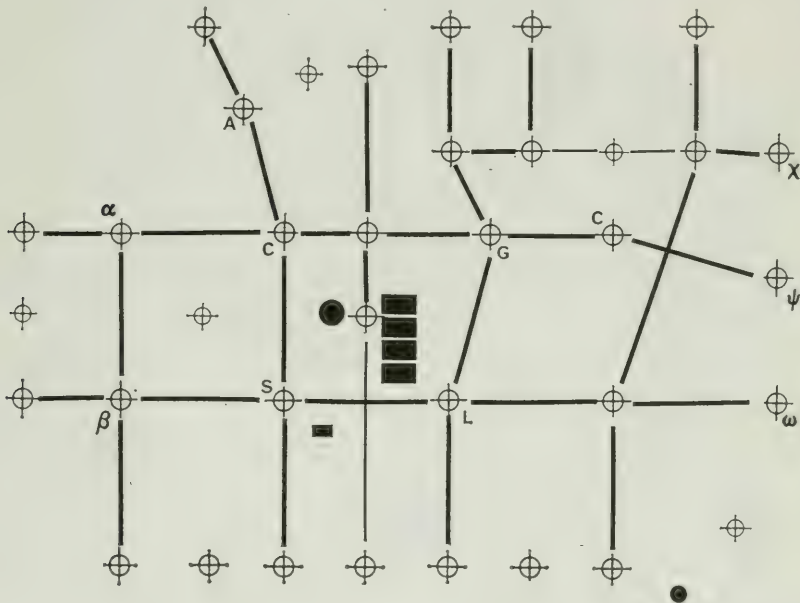
Text-figure 3. A schematic diagram or constellar map of the relative distribution of the normal pore canals and pore conuli which constitute a primary inertial system for reference in studying relative change in other aspects of the ostracode carapace sculpture (see text and Benson, 1972).
