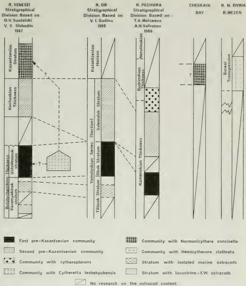
Text-figure 8. Development of late Tertiary/Quaternary ostracode faunas in northern Russia. (After Lev, 1969).
