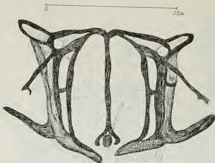
Text-figure 9. — Hirschmannia viridis (O. F. Müller, 1785) — Lower lip.
