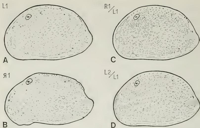
Text-fig. 3. Aurila sp. 1, Recent, Portuguese coast. — Scale: Length of the L1 0.76 mm.
