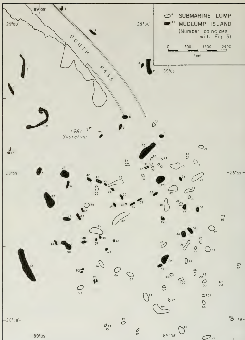
Text-figure 1. Mudlump distribution South Pass. Data from 123 maps dated between 1867-1961. (After Morgan, 1963, fig. 2.)
