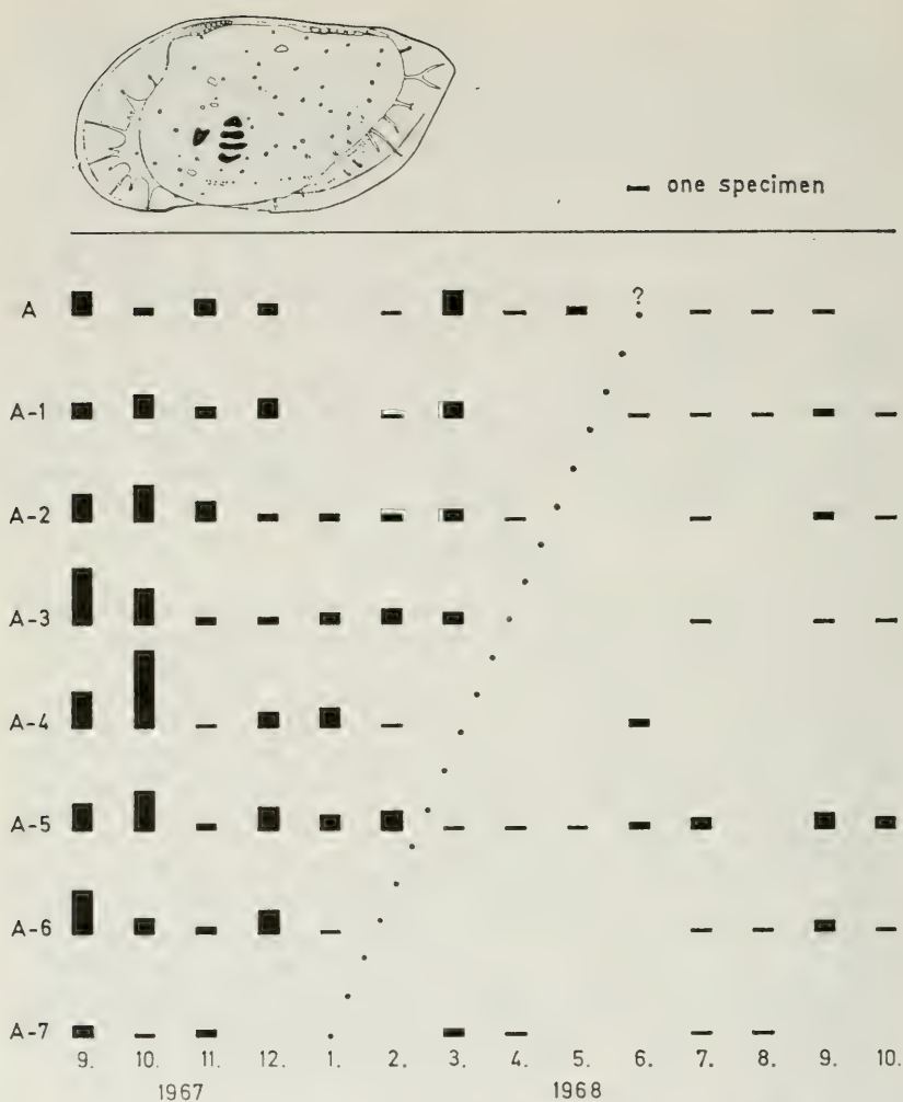
Text-figure 5. Cytheroapteron rotundatum G. W. Müller, 1894. Seasonal distribution of instars on the basis of 263 living specimens. The dotted line tentatively indicates the border between two generations and the general trend of the growth rate.
