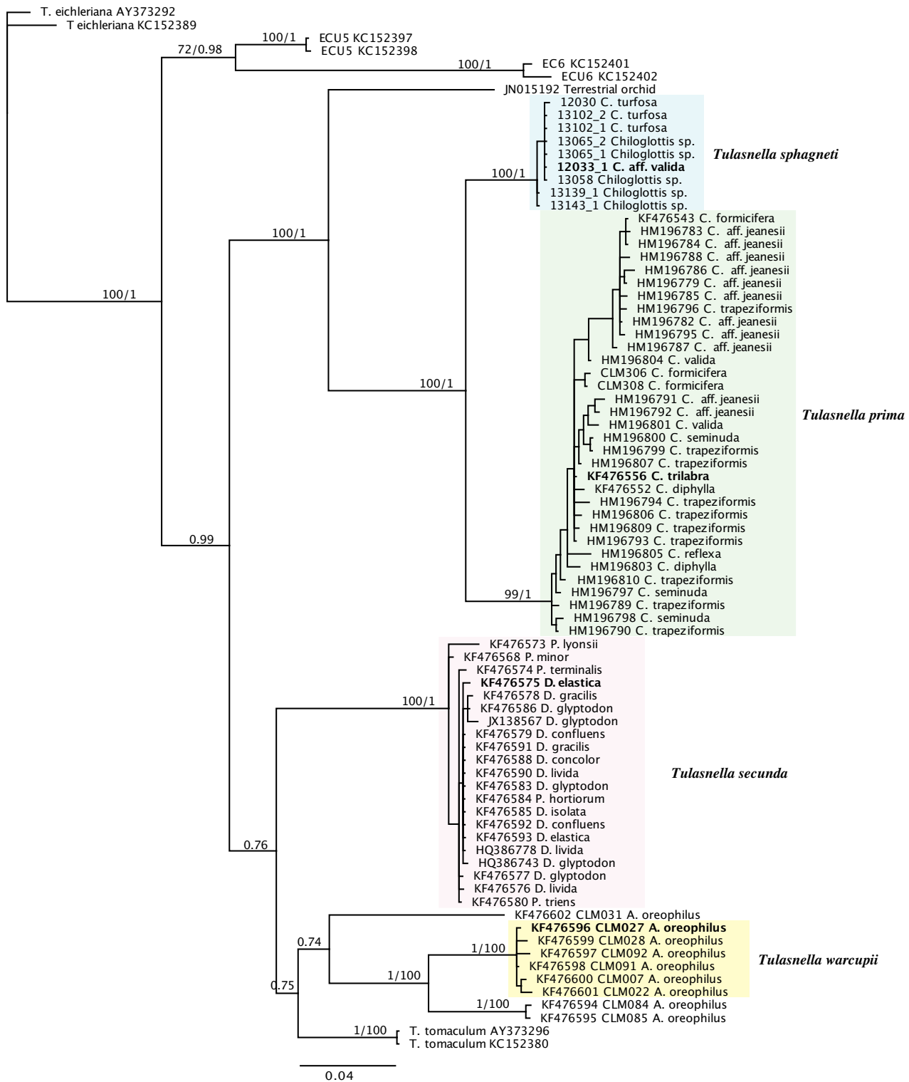
Fig. 1. Rooted MrBayes tree for Tulasnella obtained for ITS. The tree with the highest log likelihood is shown. The numbers above the branches are maximum likelihood bootstrap values/Bayesian posterior probabilities. Bootstrap values of \geq 70\% and Bayesian posterior probabilities of \geq 0.70 are shown. The branch length is proportional to the inferred divergence level. Host from which the Tulasnella isolate was collected from is indicated after the isolate number or GenBank number. Sequences from the holotype of each species is indicated in bold.
