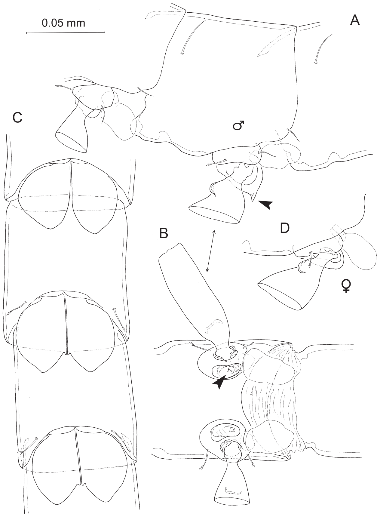
Fig. 6. Ingolfiella moluccensis sp. nov. (A–C, male paratype 1.39 mm; D, female holotype). A, detail of proximal portion of left pereiopods VI–V showing pointed process on coxa V, lateral; B, fifth pereonite with fifth pereiopods attached, ventral; C, pleonites I–III with corresponding pleopods, ventral; D, proximal portion of female left fifth pereiopod, lateral. Arrowheads point to pointed process on male coxa V.
