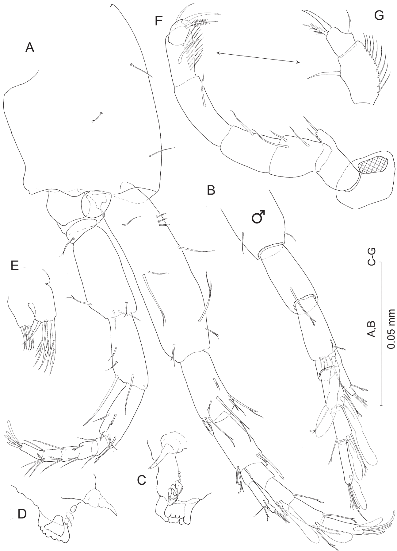
Fig. 3. Ingolfiella moluccensis sp. nov. (A, C–E: female holotype; B: male paratype 1.39 mm). A, head with right antennule and antenna, lateral; B, distal portion of male left antennule, lateral; C, left mandible; D, right mandible; E, right maxilla, posterior [= ventral]; F, right maxilliped, posterior; G, inset of distal segments of maxillipedal endopod.
