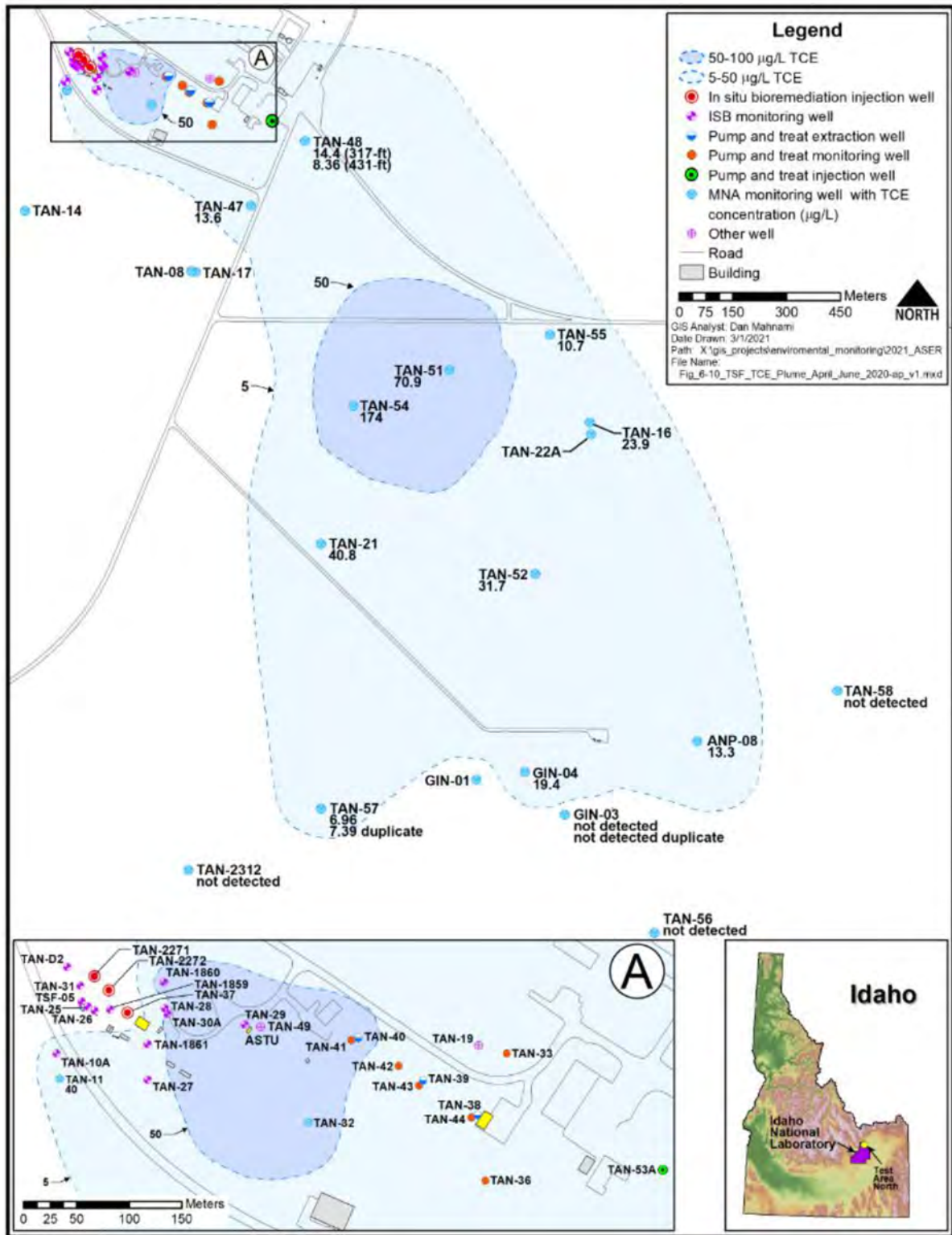
Figure 6-10. Distribution of TCE in the Snake River Plain Aquifer from April–June 2020.
