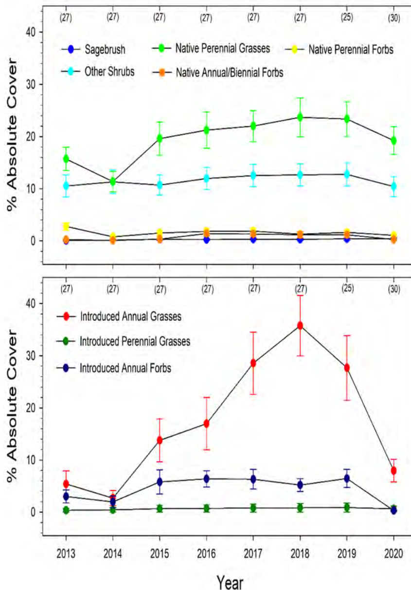
Figure 10-3. Mean Cover from Functional Groups in Non-sagebrush Plots for Native and Introduced Species on the Idaho National Laboratory Site from 2013 through 2020.
