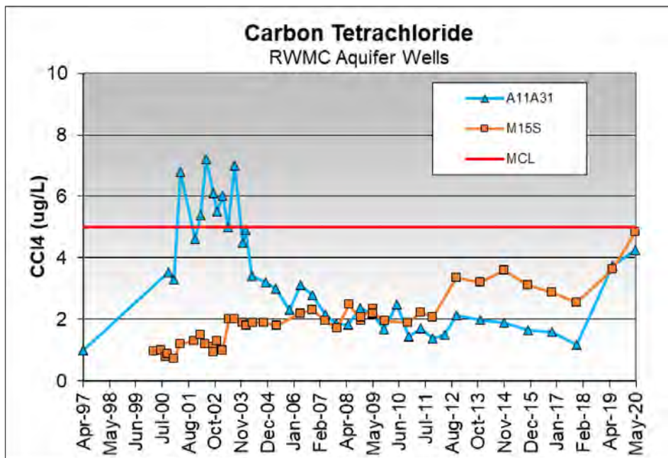
Figure 6-16. Carbon Tetrachloride (CCl4) Concentration Trends in Wells with Increasing Concentrations.
