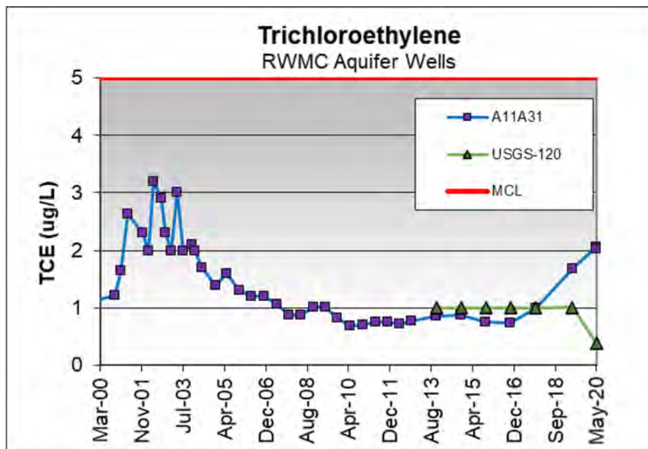
Figure 6-18. Concentration History of TCE in Aquifer Wells Downgradient of the RWMC.
