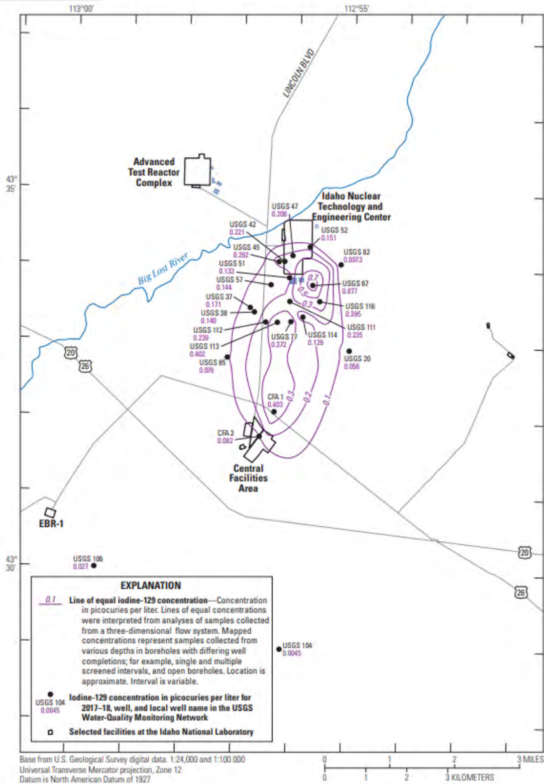
Figure 6-8. Distribution of ^{129}\text{I} in the Eastern Snake River Plain Aquifer on the INL Site in 2017–2018 (from Maimer and Bartholomay 2019).
