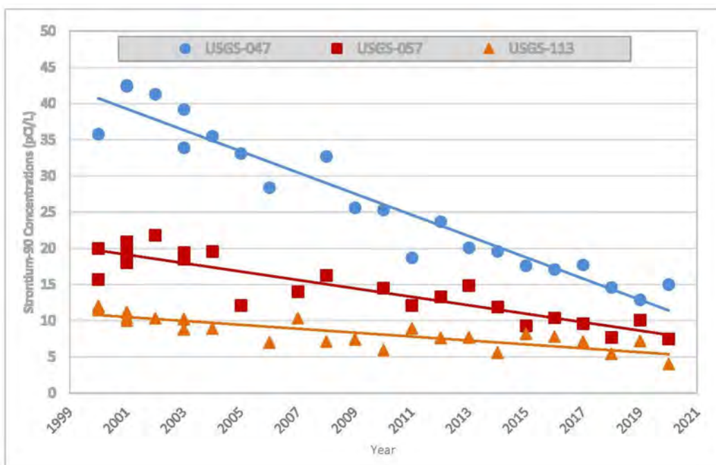
Figure 6-7. Long-term Trend of ^{90}\text{Sr} in Wells USGS-047, -057, and -113 (2000–2020).
