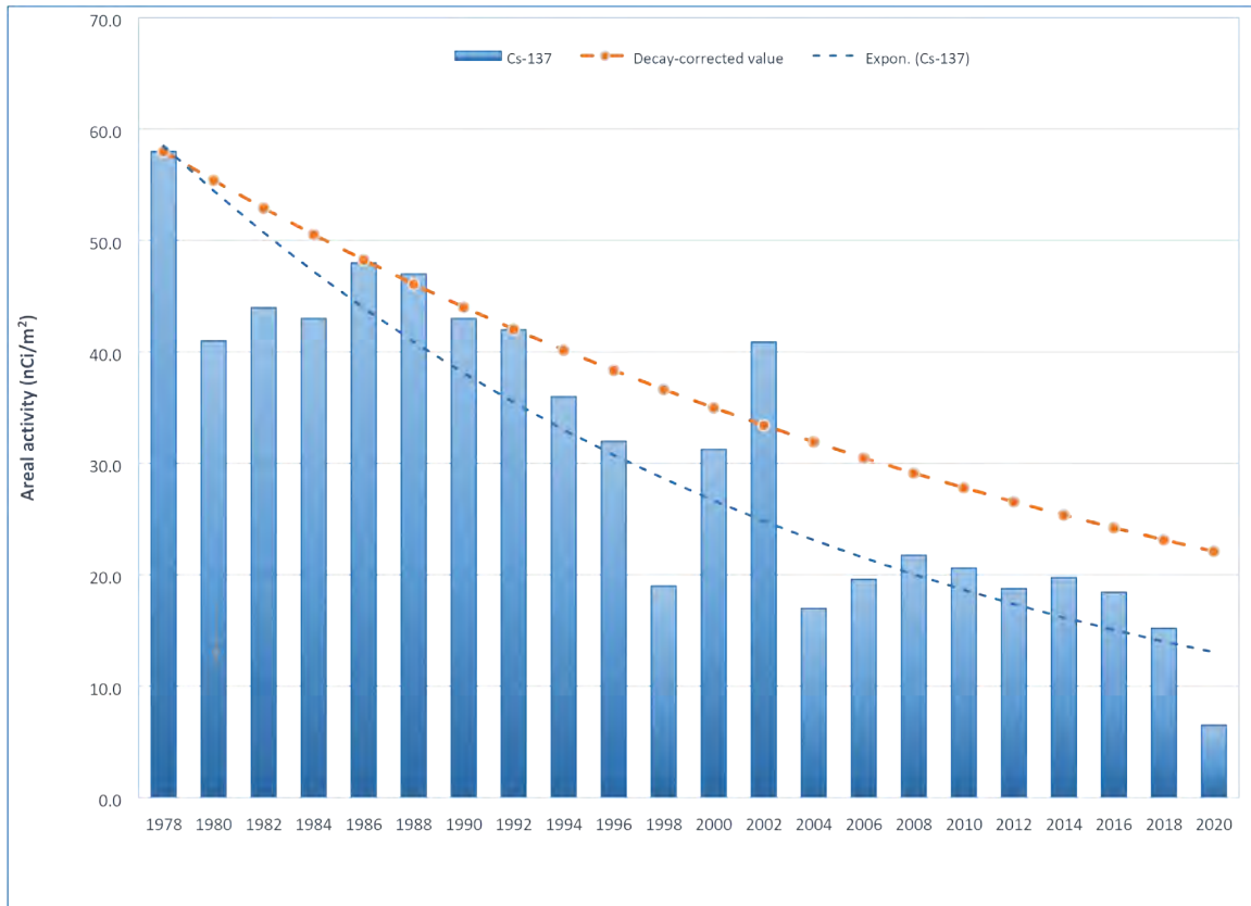
Figure 7-4. Mean (Geometric) Areal Activities of 137 Cs in Surface (0–5 cm [0–2.5 in.]) Soils off the INL Site (1978–2020). Decay-corrected values assume an initial mean areal activity measured in 1978 and a half-life of 30.17 years. The decreasing trend in the mean activity in soil samples was determined to be exponential ( r^2=0.81 ).
