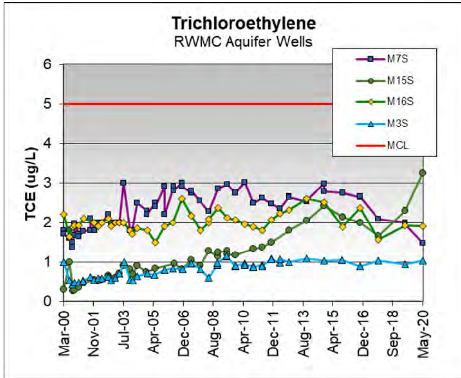
Figure 6-17. Concentration History of TCE in Aquifer Wells near the RWMC.
