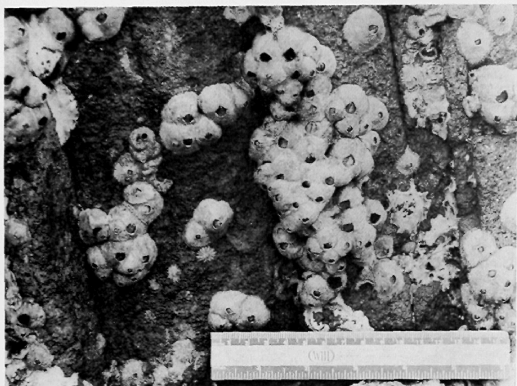
FIG. 1. Type-locality at Naos Island, Panamá (2 April 1968). The vertical rock face is dominated by clusters of both living and dead Tetraclita squamosa panamensis . The substratum is fine grained, igneous rock (dacite).
