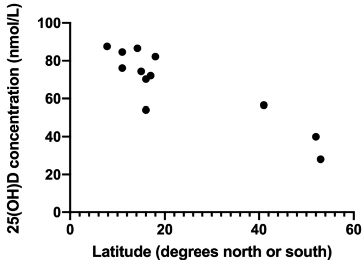
Figure: Relationship between vitamin D concentration [25(OH)D] and latitude in the African Caribbean population. Note: Mean 25(OH)D concentration of 12 papers included in the meta-analysis. Latitude reported by author or estimated. Note additional unpublished data was provided by some authors.
