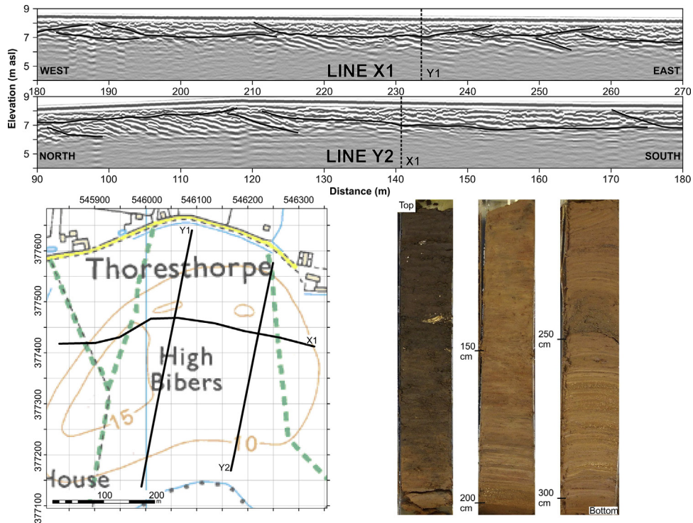
Fig. 6. Results of GPR surveys across Thoresthorpe (High Bibers), with migrated results for three transects and interpretive stratigraphic boundaries annotated on the print-outs, and details of the borehole that was recovered and sampled for OSL dating.
