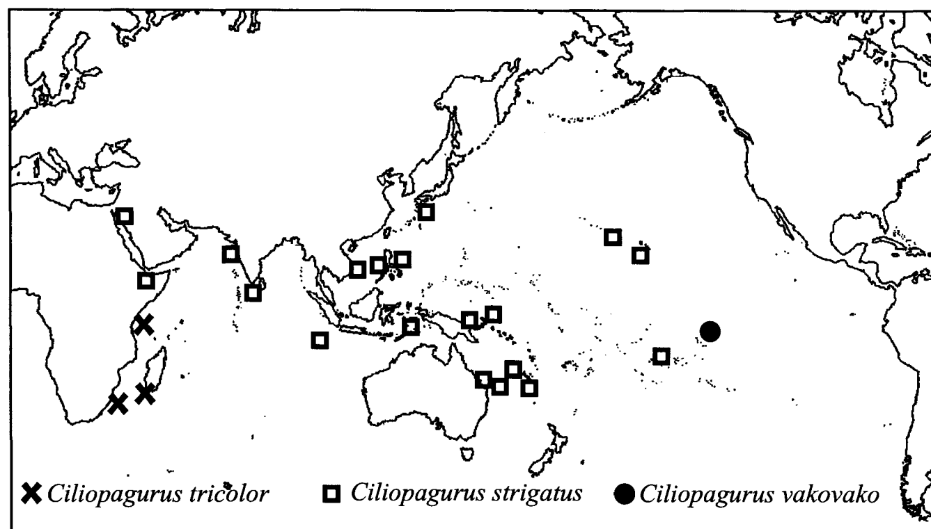
Fig. 4. Indo-West Pacific distribution for the intertidal Ciliopagurus species: C. tricolor Forest, 1995; C. strigatus (Herbst, 1804); C. vakovako , new species (adapted from Forest, 1995: Fig. 29).
