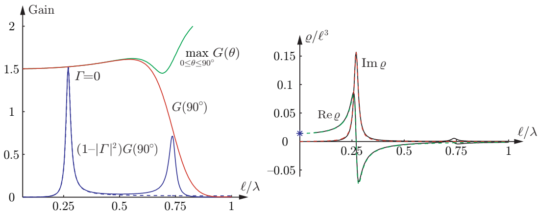
Figure 4: The maximal gain, the partial gain at \theta = 90^\circ , and the partial realized gain at \theta = 90^\circ (left figure), and the extinction volume q (right figure) for the monopole antenna. The different curves in the right figure correspond to a MoM solution (solid curves) and Q-factor approximation (dashed curves). The low frequency estimates of the monopole antenna with wire ground plane is indicated by the cross.
