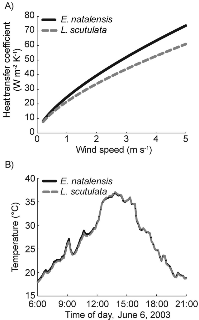
Figure 8. (A) Calculated heat transfer coefficients for similarly sized Echinolittorina natalensis (black line) and Littorina scutulata (gray line). Higher values increase the convective heat exchange with the surrounding air. Values are calculated for 25 °C air temperature and shells sitting with the aperture against the substratum. (B) Predicted body temperatures for a representative hot day, for brown snails of each species modeled with the foot withdrawn and shell resting on the substratum. The sculptured shell of E. natalensis was 0.2 °C cooler on average than the smooth shell of L. scutulata under identical weather conditions. The wind speed on this day was 1.2 \pm 0.6 \text{ m s}^{-1} (mean \pm 1 SD).
