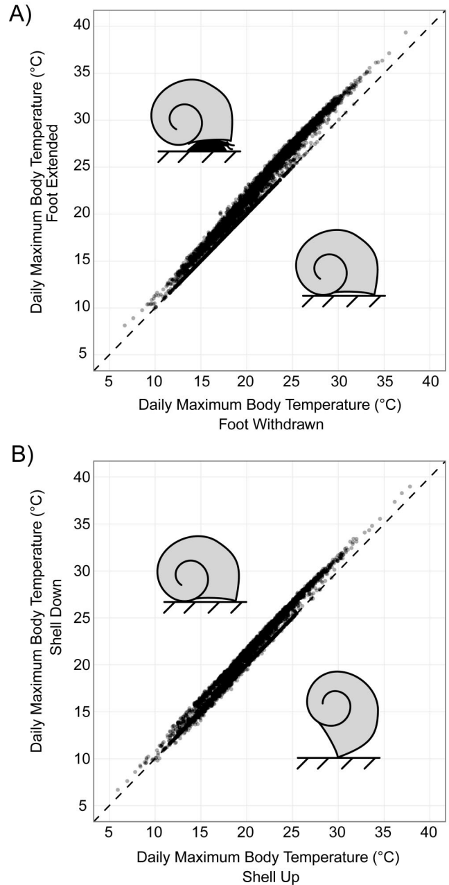
Figure 4. (A) Predicted daily maximum body temperatures for a black individual of Littorina keenae modeled with the foot out in contact with the substratum at all times or withdrawn into the shell during low tide. (B) Predicted daily maximum body temperatures for the same individual with the foot withdrawn and the shell sitting down on the substratum or with the shell tipped up on the edge of the aperture lip. Temperatures were predicted using environmental data for HMS from 1999 to 2009 ( n = 3652 days). The snail was modeled on horizontal substratum at 2.0 m above mean lower low water. A line of unity is plotted in both panels.
