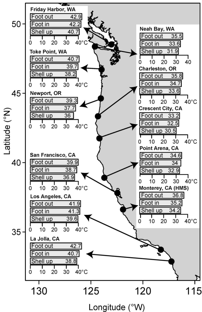
Figure 5. Maximum predicted body temperatures for a black individual of Littorina scutulata at 11 sites along the west coast of North America, using environmental data from 1 August 2007 through 1 August 2009. Temperatures are given for the same snail in three positions: with the foot out on the rock at all times, with the foot withdrawn into the shell at low tide, and with the shell tipped up on edge during low tide. All models were run with the snail sitting on a horizontal surface at the height of the maximum still tide level for each site.
