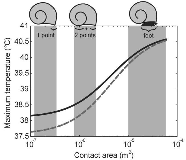
Figure 6. Maximum predicted body temperatures for a black snail (solid line) and white snail (dashed line) modeled with a range of contact areas on the substratum, using environmental data from HMS for 1999–2009. The shaded areas represent the typical range of contact areas for littorinid snails with only the lip of the shell glued to the substratum (1 point), resting on the lip and main whorl of the shell (2 points), or attached by the foot. As contact area increases, conductive heat flux reduces the effect of shell color differences on body temperature.
