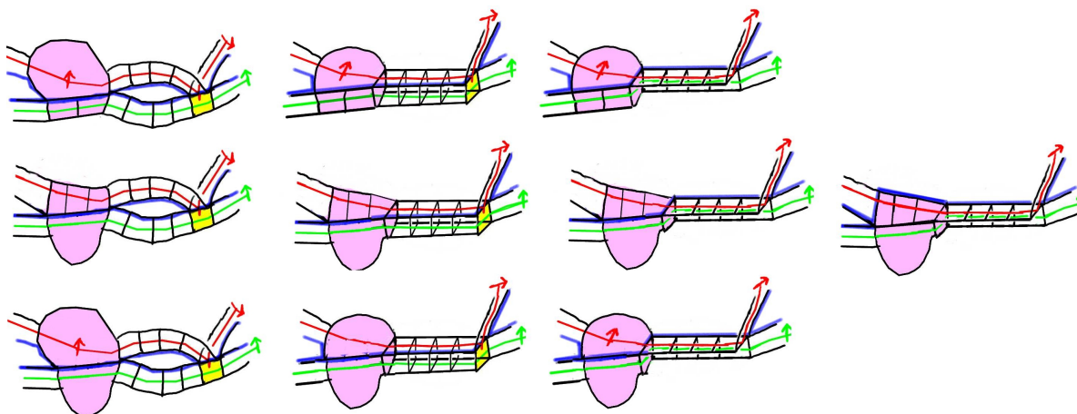
FIGURE 128. If a square bounce is consecutive with a cone absorption event, then we slide it over to bounce on the cone. The 2nd and 3rd cases lead to a decrease in the L_1, L_2 complexity and thus do not arise.
