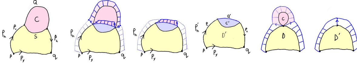
FIGURE 77. The four diagrams on the left illustrate how a hyperplane can be pushed across a cone-cell whose outerpath is not a real wall-piece. The right two figures illustrate the situation when the innerpath is trivial.
