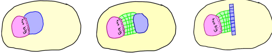
FIGURE 26. Too large to be real pieces. The left case is similar to the classical small-cancellation theory. It is a degenerate version of the middle case, which is itself covered by the rightmost case.
