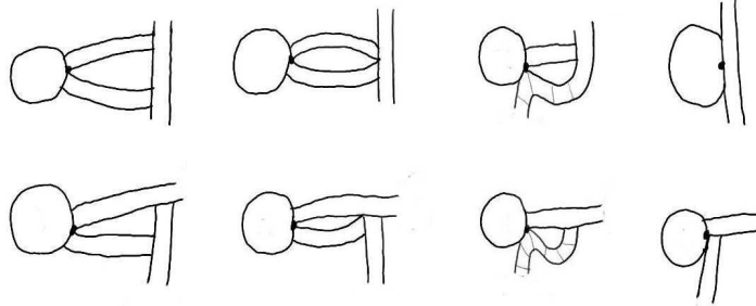
FIGURE 37. Rectangles (implicitly) parallel to the same admitted rectangle have \pi angle at the cone-cell corner.
