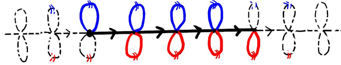
FIGURE 172. The subcomplex Y^1 \subset \widehat{X} for the word \bar{W}' = at^3bt^{-2}at^3bt^{-4} is illustrated in bold. The reader should check that the base lift of \bar{W}' at the basepoint only passes through two b edges and two a edges, but we include their intermediate \mathbb{Z} -translates.
