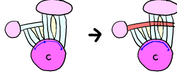
FIGURE 53. An explicit rectangle piece extends to include a cone piece.
