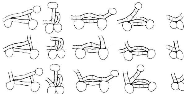
FIGURE 49. Some cases requiring a -\frac{\pi}{2} angle . These figures should only be viewed by readers who are 18 years or older.
