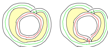
FIGURE 130. One or two (alternate) square bounces cannot be all, for otherwise a carrier would be 1-sided.
