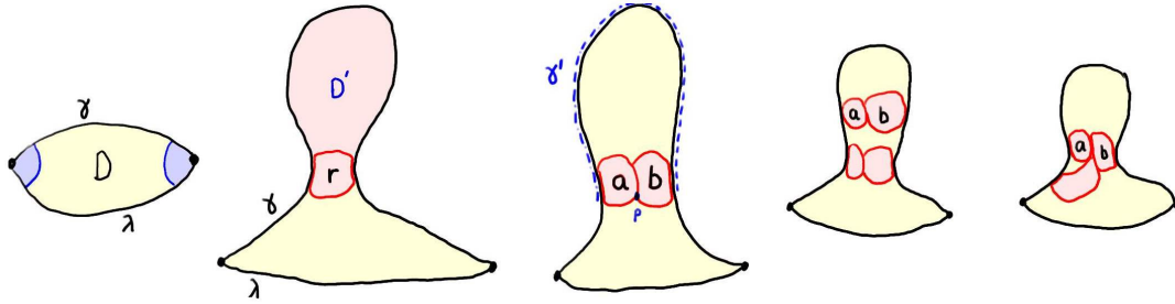
FIGURE 173. Pac-Man: The first figure shows the only two places where an extreme cell could lie, the second figure shows the subdiagram D' subtended by r , the third figure illustrates a bridge, and the fourth and fifth figures illustrate bridges that are not outermost.
