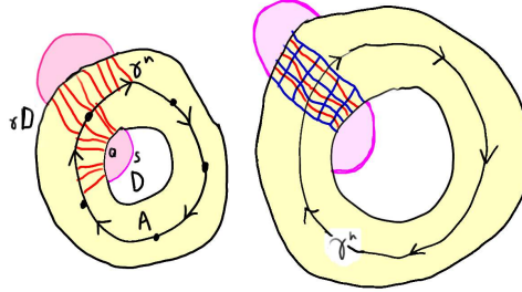
FIGURE 72. Torsion in cones in higher dimensions
