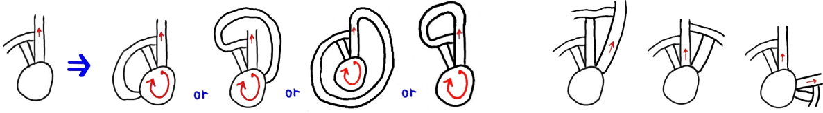
FIGURE 55. Limiting consecutive wall-pieces around internal cone-cell.
