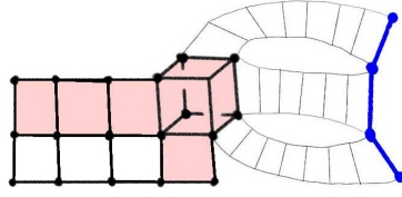
FIGURE 16. The above example illustrate a length 3 bold interval U whose wall projection onto a bold complex V is the shaded subcomplex of V . The ambient complex is not simply-connected.
