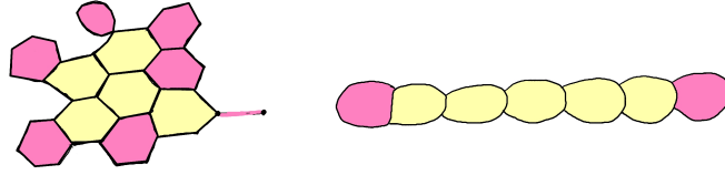
FIGURE 14. On the left in clockwise order we have a: 2-shell, 3-shell, spur, 3-shell, 1-shell, 1-shell, and 0-shell. On the right is a ladder.
