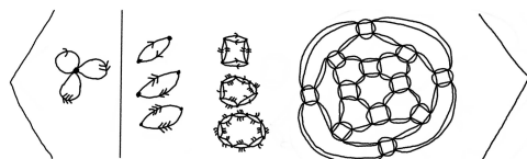
FIGURE 68. The 2-3-4 triangle group: A Coxeter group yields a graded presentation. Its generators are the usual generators. Its grade i relators are Cayley graphs of the i -generator Coxeter subgroups. For a relator Y of grade \geq 3 , the induced cubical presentation Y^* is already simply-connected so |Y^*| = \infty .
