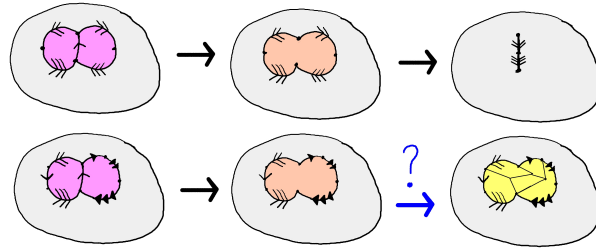
FIGURE 22. A pair of cone-cells can sometimes be combined and then possibly replaced by a square diagram.
