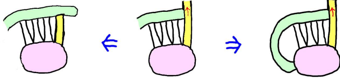
FIGURE 56. Using the argument of Lemma 3.28, if the middle diagram existed, then the hyperplane would be forced to also emerge from the cone as on the right. However, in applications, this is impossible by Scheme 3.24, so all the rectangles end explicitly on the same rectangle.
