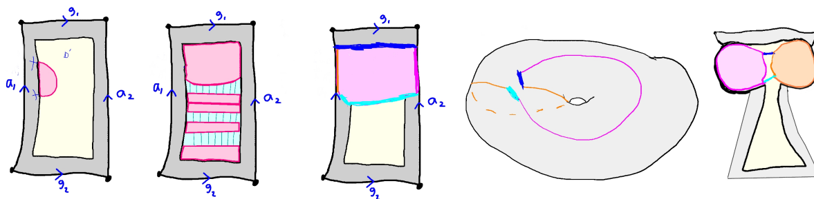
FIGURE 167. Peripherally Separating Hyperplanes:
