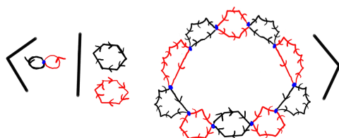
FIGURE 67. Haglund's group acting properly and cocompactly on a (6, 10) Gromov polyhedron.
