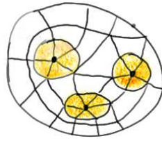
FIGURE 21. Cone-cells in D \rightarrow X^*
