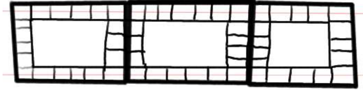
FIGURE 108. There is a ladder containing three cone-cells in the complex above such that the first and last cone-cells are connected by a pair of hyperplanes without a square diagram between them.
