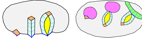
FIGURE 17. Generalized Corners of Squares: The boundary of the diagram on the left has three illustrated corners of generalized squares. The first is a genuine square with a corner on the boundary. The second is a remote square which could obviously be pushed to the boundary. The third is typical as the two rectangles from the square to the boundary bound a nontrivial square subdiagram. The diagram on the right illustrates corners of generalized squares on cone-cells and on a rectangle.
