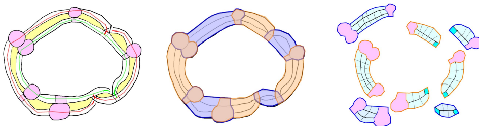
FIGURE 126. Each subdiagram of B starting and ending at an event (after absorptions) is either a single cone-cell, a ladder with exactly two cone-cells, a corner of generalized square on a cone-cell, or a bigonal square diagram.
