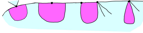
FIGURE 62. Singular doubly-external, doubly-external, singly-external, and nil-external corners.
