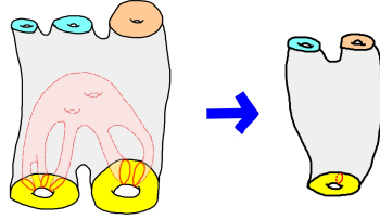
FIGURE 171. The wall W_H is indicated within the torus P_0 at the bottom on the right. Its “absorbing wall” extension is indicated in the covering space on the left.
