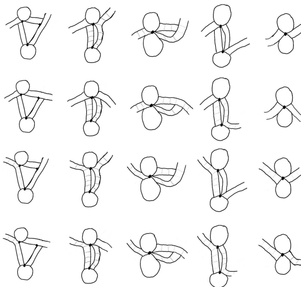
FIGURE 50. Some more cases requiring a 0 or -\frac{\pi}{2} angle
