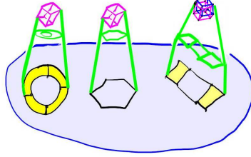
FIGURE 152. Cubical cone points:
