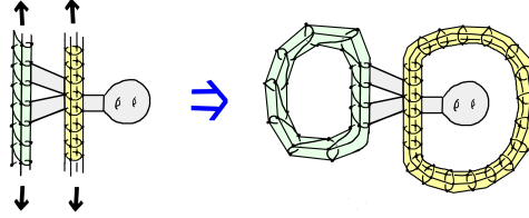
FIGURE 166. Closing up two infinite cylinders in base space.
