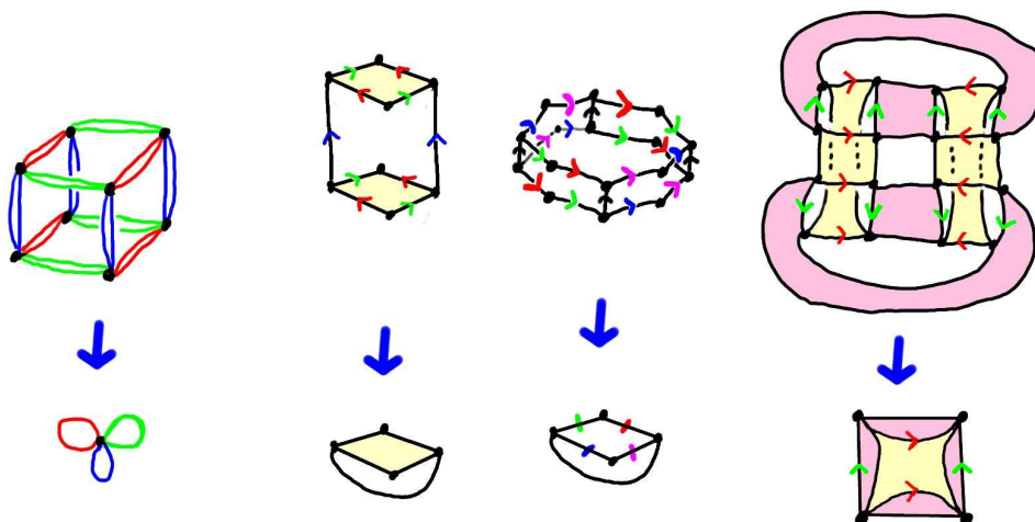
FIGURE 144. The preimages in \check{Y} \rightarrow Y of hyperplanes in Y are walls in \check{Y} . We have indicated some walls with corresponding labelled edges. The most interesting case is on the right, where \#_W \neq H_1(-; \mathbb{Z}_2) .
