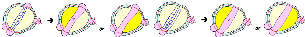
FIGURE 85. If there is a cancellable pair of cone-cells as on the first diagram, then there is a smaller complexity counterexample as shaded in the second or third. The second diagram is the case where the two walls in the cancellable pair are distinct, and the third where the two walls are the same. The fourth diagram indicates a fake wall-piece, which is absorbed analogously in the fifth and sixth diagrams.
