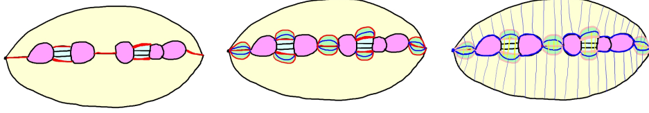
FIGURE 163. \tilde{X}_o^* has thin bigons, for large girth hyperbolic fillings.
