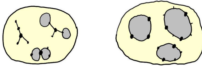
FIGURE 30. Nontrivial singular diagrams of D - E “inflate” to the shard 2-cells of \bar{D} .
