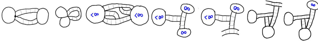
FIGURE 34. More impossible configurations of admitted rectangles and cone-cells. The first diagram is missing some admitted rectangles. The second diagram is impossible assuming that the bounded region is a shard and has minimal area.
