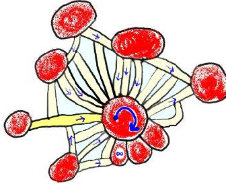
FIGURE 57. Clockwise from the yellow rectangle edge we have:
