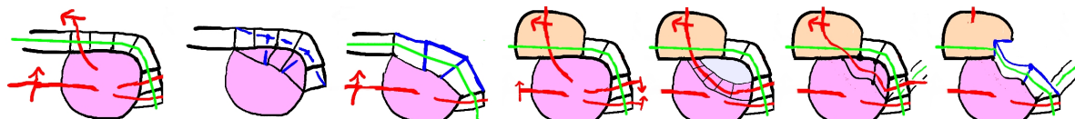
FIGURE 124. Replacing the ladder L along C with a shorter square ladder L' .
