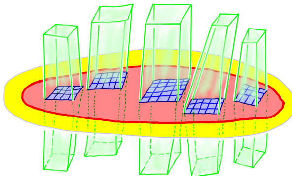
FIGURE 142. Heuristic picture of a cosparse cubulation.
