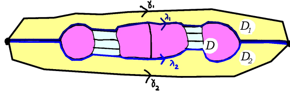
FIGURE 162. The diagram E between \gamma_1, \gamma_2 must decompose as the union of a “stemmed ladder” D surrounded by two square diagrams D_1, D_2 .
