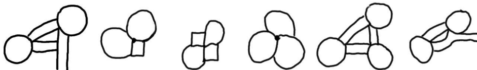
FIGURE 48. In most cases, when there is an infinite cone around a shard, then the shard (or one of its boundary vertices) will have negative curvature depending on whether we use the split-angling or the type-angling.
