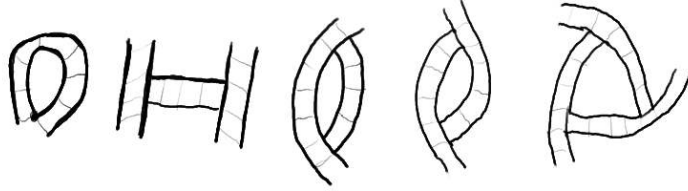
FIGURE 33. Some impossible configurations of admitted rectangles. The first diagram is impossible under the assumption that there are no cone-cells inside and this square diagram has minimal area. The other diagrams are impossible because of the logic of admitted rectangles.
