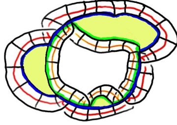
FIGURE 121. The nonplanar 2-complex B = L_1 \cup_{\varepsilon_1} E \cup_{\varepsilon_2} L_2 will be adjusted to produce a thin annular diagram.
