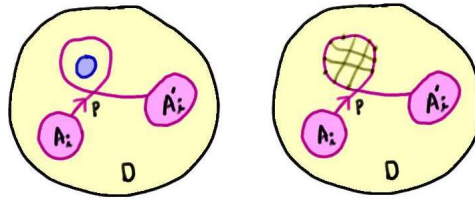
FIGURE 23. The path P wraps around a cone-cell in the diagram on the left, so we cannot combine A and A' . There is no problem on the right, as P wraps around a square diagram.
