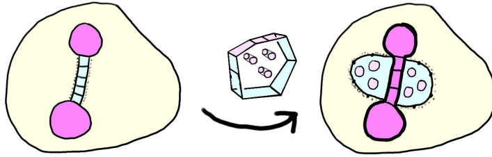
FIGURE 25. Pushing across a drum to obtain a graded replacement.
