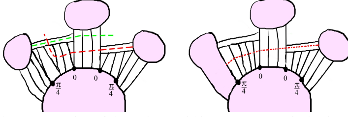
FIGURE 58. The concatenation of three pieces within C_{\frac{\pi}{4}}W_0C_0W_{\frac{\pi}{4}}C is dominated by the concatenation of two wall-pieces. When \dim(X) = 2 , it is dominated by a single wall-piece.
