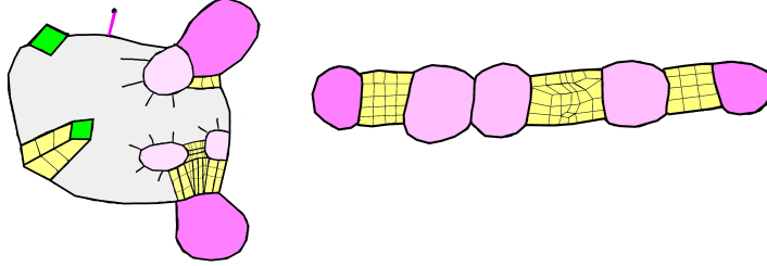
FIGURE 15. Two \theta -shells, two generalized corners of squares, and a spur in a cubical small-cancellation diagram on the left. A cubical small-cancellation ladder on the right.
