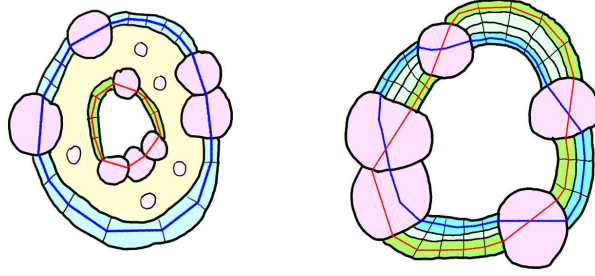
FIGURE 120. B is thick on the left, and B is thin on the right.
