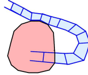
FIGURE 28. The subcomplex above interosculates with a hyperplane.
