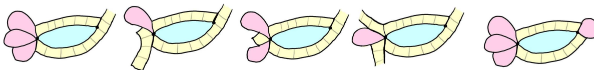
FIGURE 44. Three additional squares/cone-cells at one corner, and one at the other.
