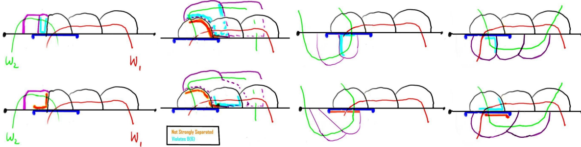
FIGURE 112. I believe this covers most of the variety of cases.
