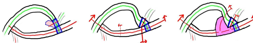
FIGURE 123. The left diagram shows that a cancellable pair of squares between L_1, L_2 cannot occur except at a bounce as illustrated in the middle. In this case, the orientations shows that the square-bounce is consecutive with a cone-event as on the right.
