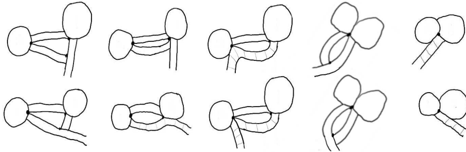
FIGURE 39. \frac{3}{4}\pi is assigned to the internal angle between edges whose emerging rectangles end in parallel on a cone-cell/rectangle pair.
