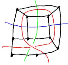
FIGURE 78. A nonembedded wall in \tilde{X}^* .
