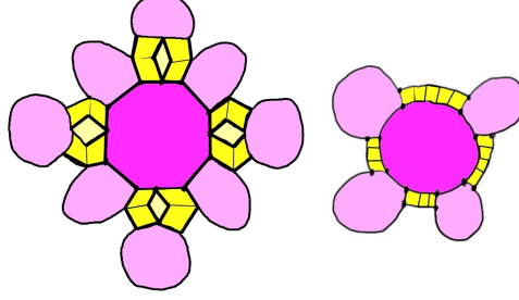
FIGURE 59. The diagram suggests that Theorem 3.31 is sharp when \dim(X) = 2 .
