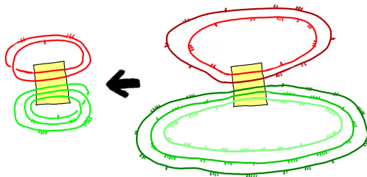
FIGURE 169. The high girth expanded edge space E_3^+ .
