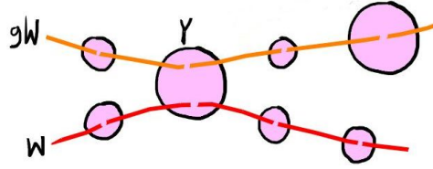
FIGURE 137. If gW \cap Y and W \cap Y diverge (by not passing through the same piece) then N(W) \cap N(gW) = Y .
