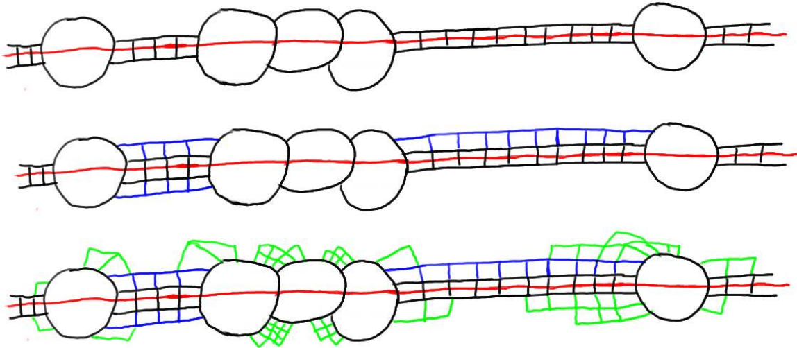
FIGURE 90. A carrier, a thickened carrier, and an extended carrier
