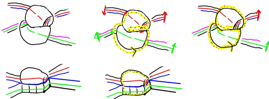
FIGURE 132. We rechoose the cone-cells so that square ladders end on disjoint arcs. There can be many ways of doing this, as illustrated on the top two.
