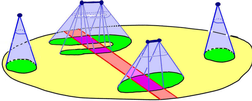
FIGURE 146. C_w(\langle X | Y_1, Y_2, Y_3, Y_4 \rangle) has Y_i \cap w with 0, 2, 1, 0 components respectively.
