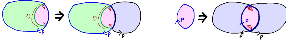
FIGURE 70. We glue a phony Y_i -cone-cell with boundary path P along the outerpath of a diagram to reach a contradiction.
