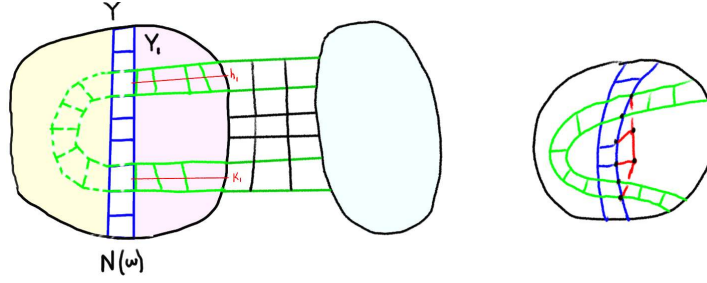
FIGURE 148. Persistence of Condition 5.67.(3)
