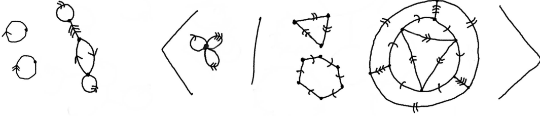
FIGURE 154. Let \tilde{Y}_{11} and \tilde{Y}_{12} and \tilde{Y}_{21} denote the universal covers of the three graphs on the left, and let \tilde{X} denote the universal cover of the bouquet of three circles. The graded cubical presentation on the right could be obtained from this initial data following Lemma 12.20.
