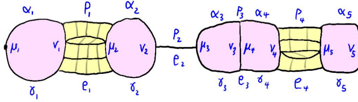
FIGURE 60. Ladder Definition Notation
