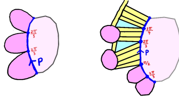
FIGURE 73. The total defect \Omega_i(P) of the path P \rightarrow Y_i on the right is \leq \frac{\pi}{3} + \frac{\pi}{2} + \frac{\pi}{3} + \frac{\pi}{4} .
