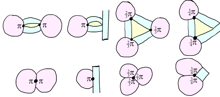
FIGURE 35. Internal cone-angles for the split-angling are modeled by the four cases above: All variants of the four cases above are provided in Figures 36, 37, 38, and 39.
