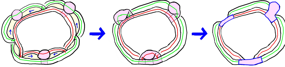
FIGURE 122. Slide bouncing events to the cone-cells and then rechoose cone-cells: We slide the events in the diagram on the left to obtain the diagram on the right. Note that the shaded parts of E are forced to have no squares. The cone-cells in the adjusted diagram are a bit larger and absorb more squares from the other ladder than they did before. We then rechoose the cone-cells to absorb squares where bouncing events occur, and thus obtain a planar B .
