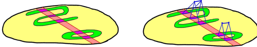
FIGURE 149. Each T_i \times I added on the right connects the wall in a cone.
