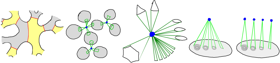
FIGURE 151. \pi_1 X^* \bar{w}^* \subset \bar{X}^* is depicted in the first diagram. Each component of \bar{X}^* - \pi_1 X^* N^o(\bar{w}^*) is a translate of \bar{X}_\pm^* that itself has a tree structure. This tree structure is indicated for \bar{X}_+^* in the second diagram. Its vertex spaces are cone points and cube complexes and its edge spaces are cones. The stabilizers of the cone point vertex spaces are the various \text{Aut}(Y_i) where Y_i is cut by \bar{w} . The stabilizers of the cone edge spaces are the subgroups \text{Aut}(Y_{ij}) , where Y_{ij} are the parts of Y_i after cutting along \bar{w} . A neighborhood of a minor vertex space is depicted in the third diagram and its vertex group \text{Aut}(Y_i) permutes the orbits of the various Y_{ij} each of which corresponds to a cone edge space attached to a distinct \bar{X}_{+k}^* translate. The “unwedging” procedure to get from X_+^* to X_{+1}^* is suggested by the last two figures.
