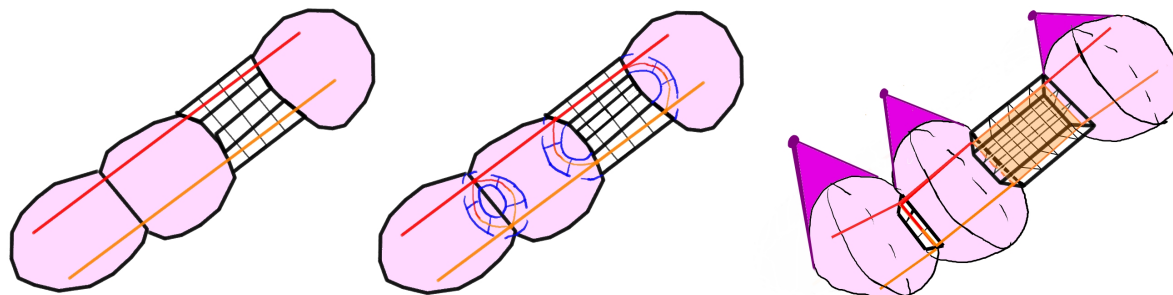
FIGURE 138. Since the annulus B is thin, Condition 5.67 implies that the two annuladders travel through the same immersed wall \bar{W} \rightarrow X^* , and hence B \rightarrow X^* factors through the immersed carrier \bar{N} \rightarrow X^* consisting of cones and carriers of hyperplanes.
