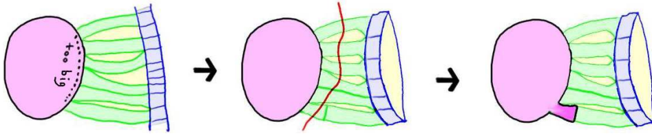
FIGURE 27. Big rectangle-piece yields an adjacent hyperplane with big piece, which must then cross \tilde{Y}_i , and hence yields an absorbable square.
