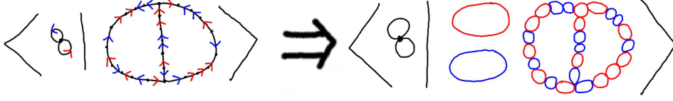
FIGURE 69. Substituting: Let \langle B \mid C \rangle denote a graphical presentation where B is a bouquet of circles u, v , and C \rightarrow B is an immersed theta-graph. Let X be a new bouquet of circles x, y , and let U, V denote immersed circles, and “substitute” copies of U, V for edges labelled by u, v in C and then fold to obtain a graph Y . Even preserving “orientation”, there are many ways of doing this, and one could choose basepoints, or just do it randomly. When \langle B \mid C \rangle and \langle X \mid U, V \rangle are sufficiently small-cancellation, then so will the cubical presentation \langle X \mid U, V, Y \rangle where U, V have grade 1 and Y has grade 2.
