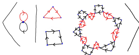
FIGURE 66. There are two grade-1 cones, and one grade-2 cone. All nonabsorbable pieces are between the grade-2 cone and itself. The example doesn't satisfy C(p) for very large p , but suggests a plethora of further examples along similar lines. For a presentation of the form \langle b, c \mid b^m, c^n, W \rangle , one can attach copies of b^m and c^n to a copy of W along its syllables. When m = 2 and n = 3 , one needs |W| quite large before typical words give graded small-cancellation presentations.
