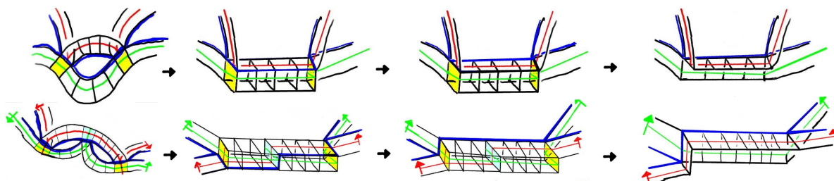
FIGURE 129. Two consecutive square events on the same side, or three alternating square events allow the reduction of the L_1, L_2 complexity.
