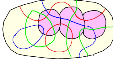
FIGURE 135. To verify Condition (3). Each wall in cones of \langle X \mid Y_i \rangle maps to a single equivalence class of hyperplanes in X , but a single equivalence class has connected intersection with each piece in each cone.
