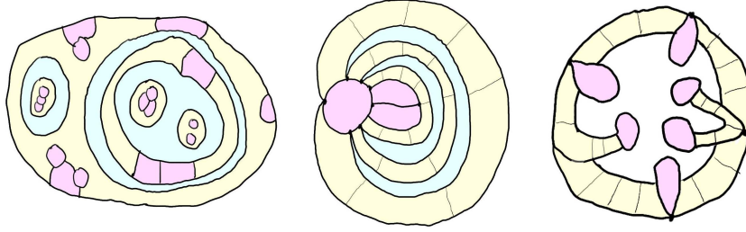
FIGURE 29. Two innermost non-simply-connected fragments on the left, a simple possibility for D' in the middle, and a complicated possibility for D' on the right (partially illustrated).
