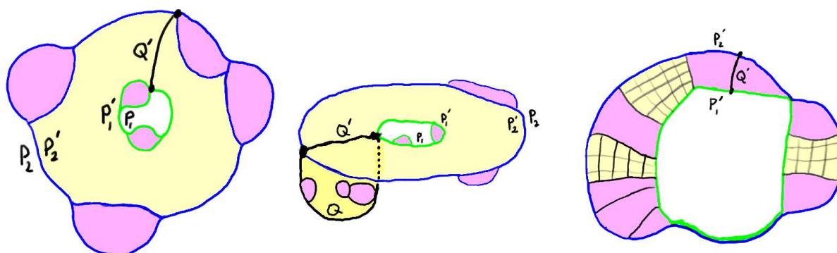
FIGURE 160. Before and after: The middle figure illustrates a typical situation where an original annulus is turned into a square annulus by pushing out cone-cells through the two bounding circles and pushing the conjugator out (so it is connected to the new conjugator by a “flap” consisting of a disk diagram in X^* ). No extra flap is illustrated on the left diagram - were Q = Q' . The diagram on the right represents the final impossible annuladder we consider.
