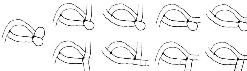
FIGURE 45. Square at one sharp corner, two cells at other.
