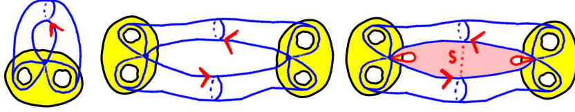
FIGURE 153. X \leftarrow \widehat{X} \hookrightarrow \widehat{X}'
