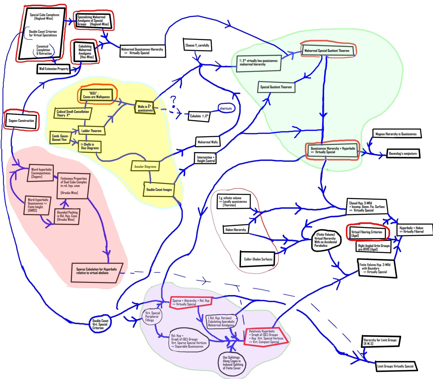
FIGURE 1. A flow chart indicating main points of the paper and some topical constellations.
