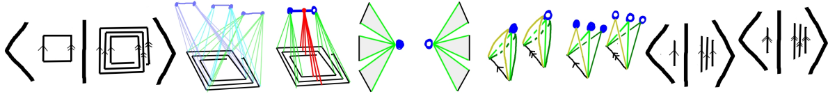
FIGURE 150. Objects considered in the hierarchy for a cubical presentation of \mathbb{Z}_3 : From left to right are: X^* , \tilde{X}^* , \bar{w}^* \subset \bar{X}^* , \bar{X}_\pm^* , X_\pm^* , X_{\pm 1}^* , and again X_{\pm 1}^* expressed as cubical presentations.
