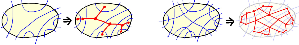
FIGURE 141. The dual cube complex on the left is a tree, the one on the right is 2-dimensional. The n -cubes correspond to certain n -fold collections of pairwise crossing walls.
