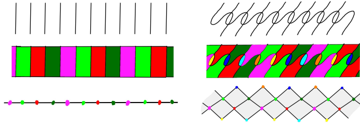
FIGURE 164. Jiggled Walls: The wallspace on an infinite strip on the left has dual cube complex homeomorphic to \mathbb{R} . If we “jiggle” the walls so that they cross their neighbors, then one obtains a thicker cube complex as on the right. Similar “thickenings” occur if we jiggle typical wallspaces on \mathbb{R}^n .
