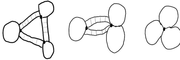
FIGURE 38. Three adjacent cone-cells.
