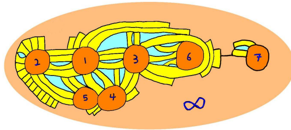
FIGURE 32. The rectified diagram: cone-cells in orange, rectangles in yellow, shards in blue. Shards corresponding to components containing no squares are not indicated.
