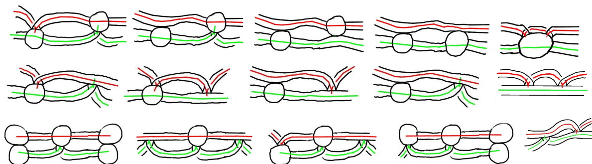
FIGURE 125. Some of these consecutive events cannot arise in a minimal situation.
