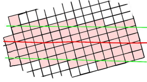
FIGURE 165. The smallest subcomplex containing a convex subspace is isometrically embedded.
