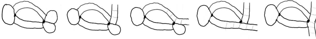
FIGURE 46. Cone-cell at one sharp corner, two additional cells at other.
