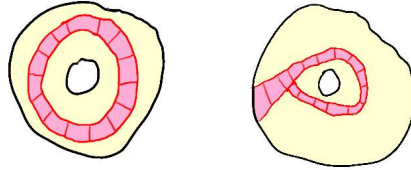
FIGURE 157. Rectangles can self-intersect in the rectified annuli
