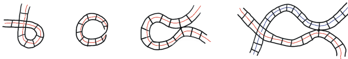
FIGURE 140. Immersed Hyperplane Pathologies
