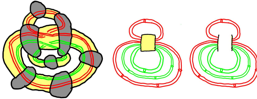
FIGURE 168. A graph of spaces on the left (the peripherals are highlighted on inside), an expanded edge space in the middle, and its associated cage on the right. In this example, the two parabolic subgroups are represented by immersed tori. The bold vertical lines in the cage correspond to the initial and terminal images of the edge space, the small circles in the cage correspond to places where the parabolic torus passes through vertex spaces, and the cylinders in the cage correspond to places where the parabolic torus passes through edge spaces.
