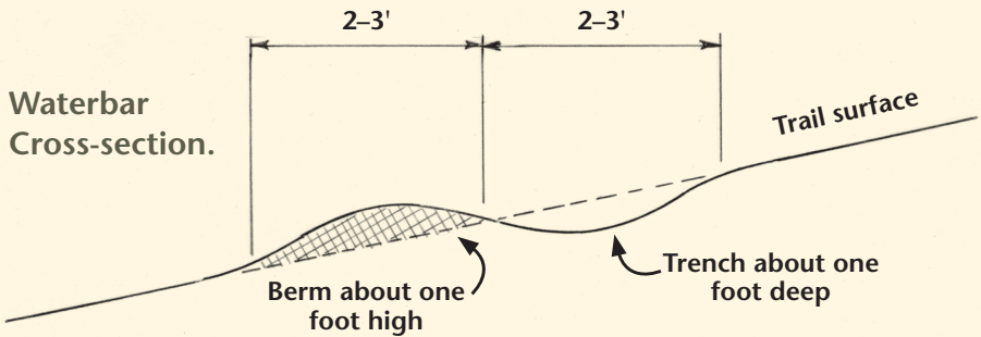
Figure 9. Waterbar Schematics.
