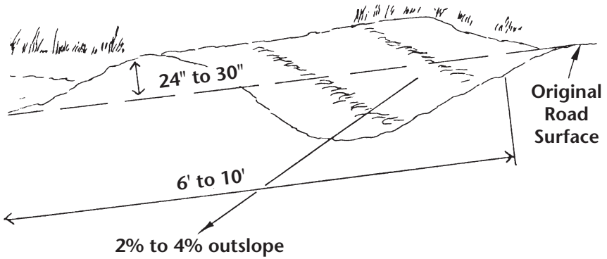
Figure 6. Waterbar Construction.
