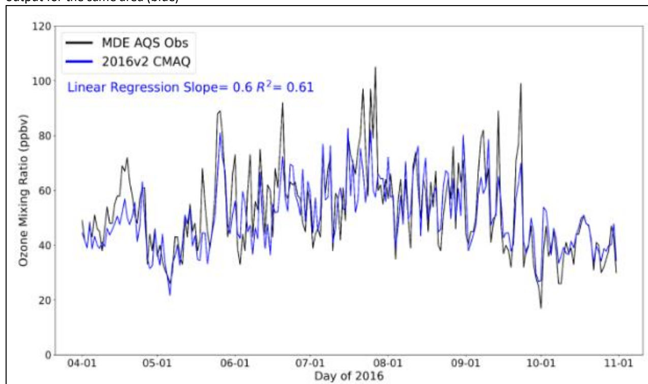
Figure 10-4: Observed averaged 8-hour ozone from the Edgewood, MD surface AQS site (black) and CMAQ model output for the same area (blue)
