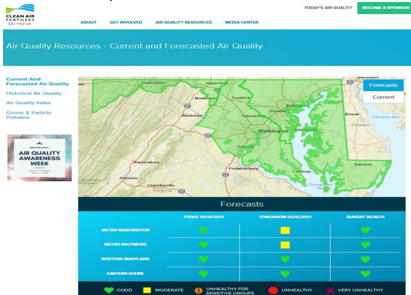
Figure 2-4: Clean Air Partners Air Quality Data and Forecasts
