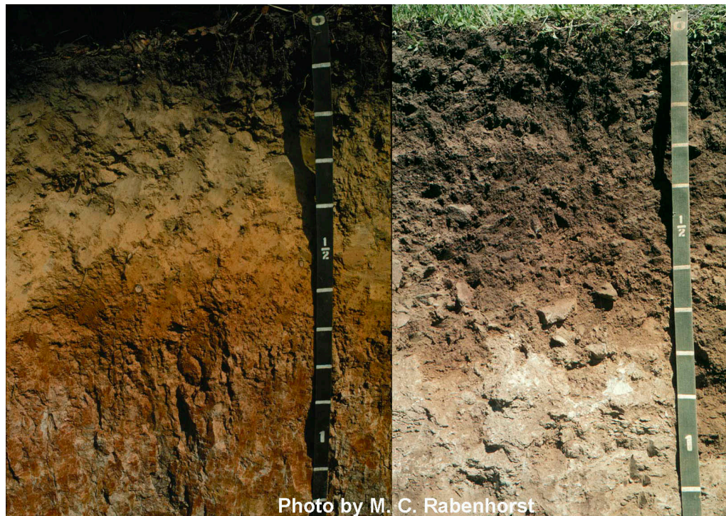
Figure 2-3. —The soil on the left, which has a fairly thin A horizon, formed under forest vegetation where much of the organic matter is added to the soil surface during leaf fall. The soil on the right, which has a much thicker A horizon, formed under prairie vegetation where much of the organic matter is added within the soil by grass roots. Scale is in 4-in increments (10 cm).
