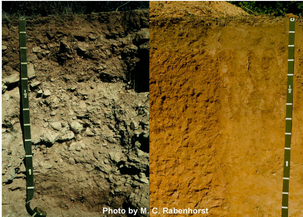
Figure 2-1. —These two soil profiles formed under dramatically different climates. The soil on the left formed under an arid climate (annual rainfall 12 in, or 300 mm) and has a zone of calcium carbonate accumulation in the Bk horizon that extends from 16 to 40 in (40 to 100 cm). The pH in the Bk horizon is approximately 8.1. The soil shown on the right formed in a humid environment (annual rainfall 44 in, or 1,100 mm) where soluble weathering products are quickly leached from the soil. This soil profile has no carbonates present at all. The pH of the Bt horizon, which extends from 8 to 28 in (20 to 70 cm), is approximately 5.5. Scale is in 4-in increments (10 cm).
