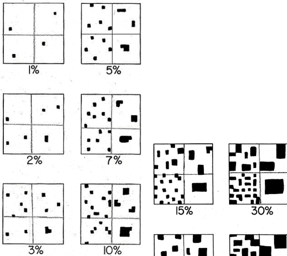
Figure 6-4.—Guide for estimating proportions from 1 to 10 percent.
