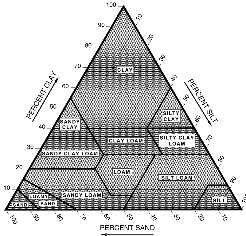
Figure 6-2.—Percentages of clay, silt, and sand in the basic USDA soil textural classes.
