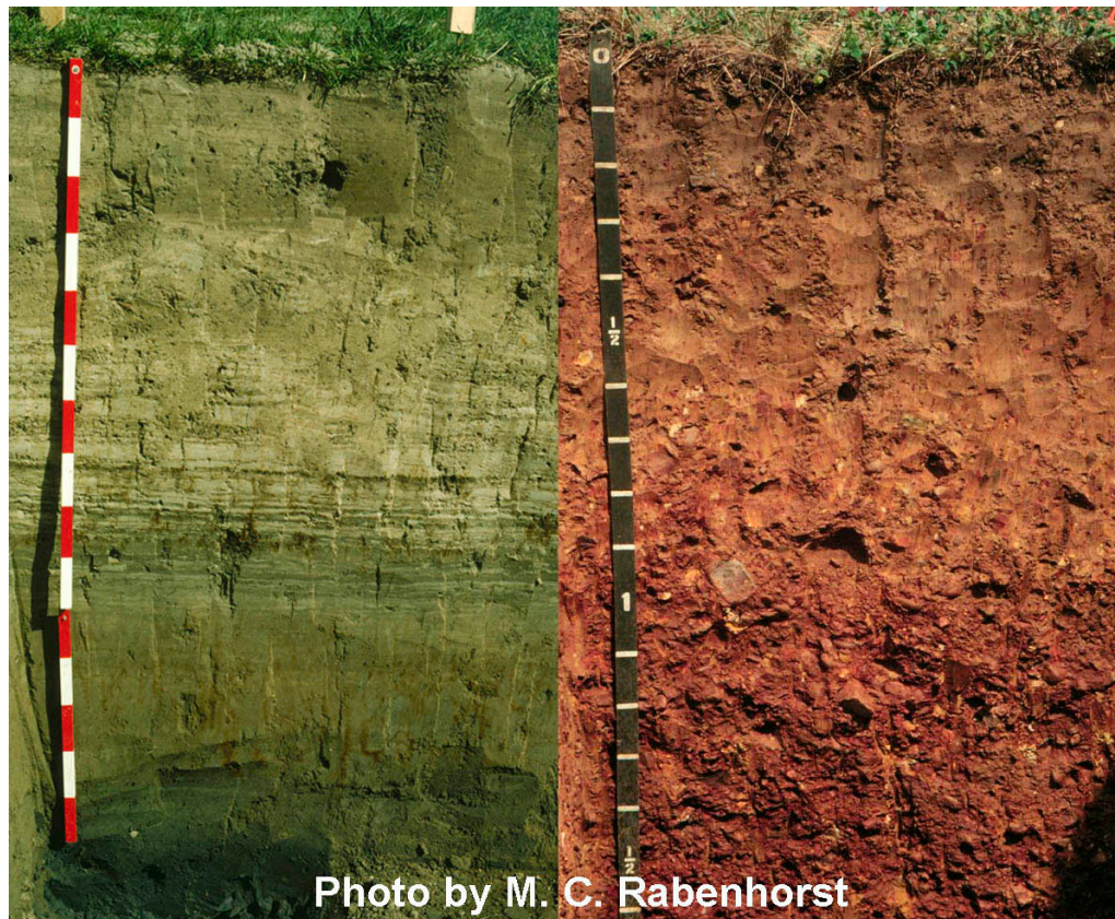
Figure 2-6. —The soil on the left is young (i.e., less than 100 years old), having formed in sediments deposited in the early 19 th century. Note the absence of well developed horizons and the preservation of original sedimentary stratification at a depth of more than 20 in (50 cm). The very old soil on the right formed in terrace deposits, which are perhaps as much as 1 million years old. It has a strong argillic (Bt) horizon that begins at a depth of about 24 in (60 cm) and extends to a depth of almost 10 ft (3 m). Scale is in 4-in increments (10 cm).
