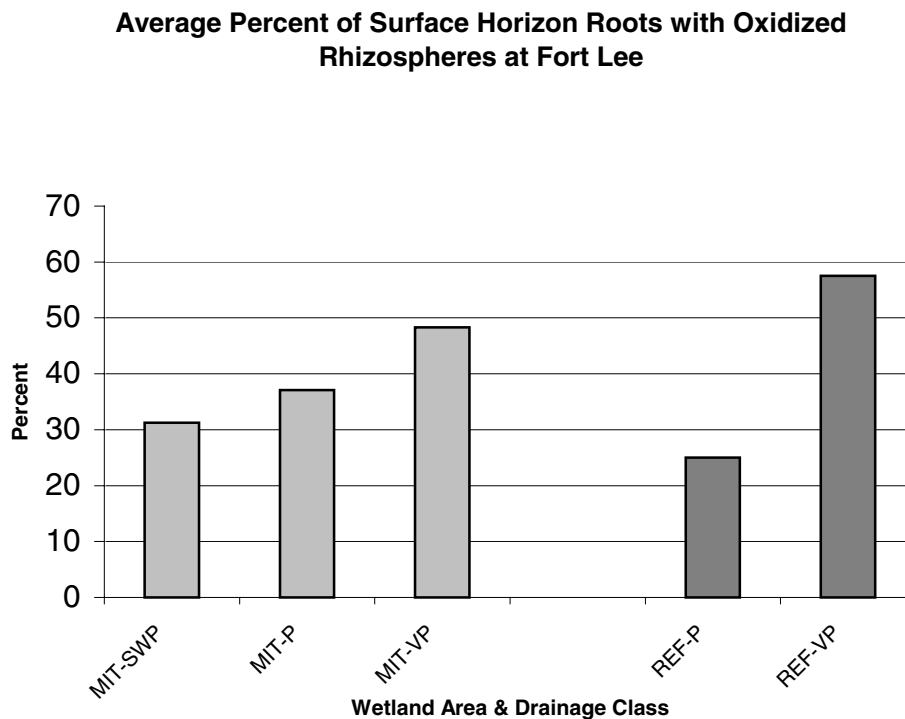
Figure 12-3. —An abundance of oxidized rhizospheres (iron concentrations) at the Fort Lee mitigation wetland (MIT) and an adjacent reference area (REF) as described by Cummings (1999). Soil drainage class was assigned based on wells directly adjacent to pedons on three study transects. Abundance of oxidized rhizospheres increased regularly as soils moved from somewhat poorly drained (SWP) to poorly drained (P) to very poorly drained (VP) conditions. The reference area soils were very high in organic matter, which may have limited or masked development of similar features in comparison.
