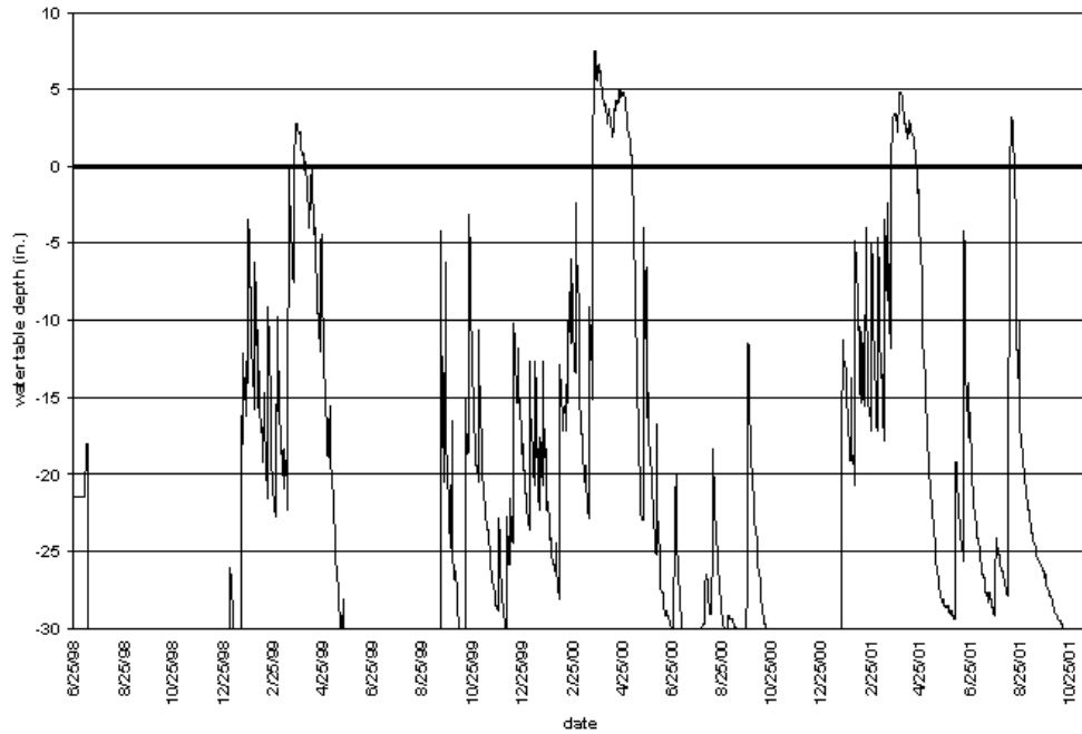
Figure 5-3.—Hydroperiod of seasonally saturated wetland.
