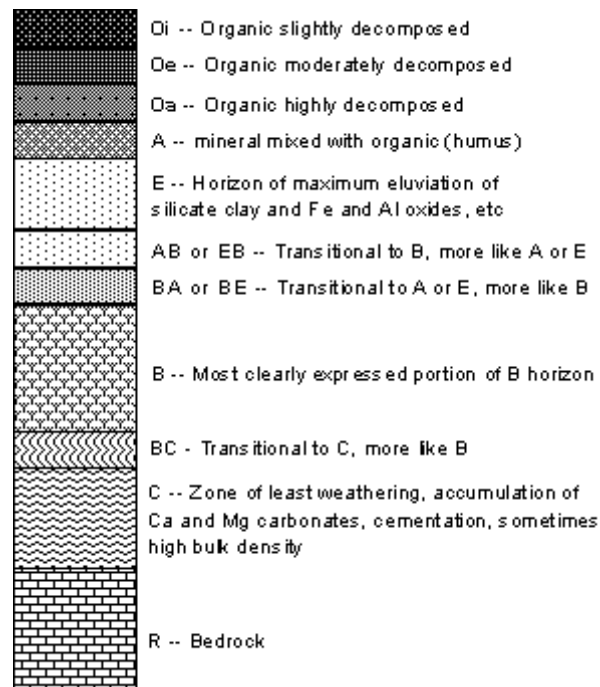
Figure 6-7.—Graphic representation of an idealized soil profile.
