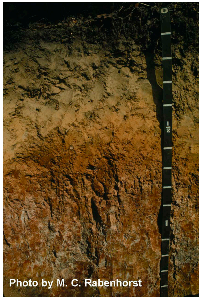
Figure 3-3.—The dark colors of the A horizon in this soil are due to enrichment with organic matter, while the reddish colors of the subsoil are primarily due to the coatings of iron oxides. Gray colors represent uncoated mineral grains where the iron oxides have been depleted.
