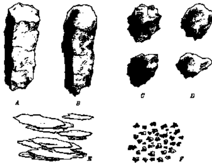
Figure 6-6.—Structure shapes: A, prismatic; B, columnar; C, angular blocky; D, subangular blocky; E, platy; and F, granular.
