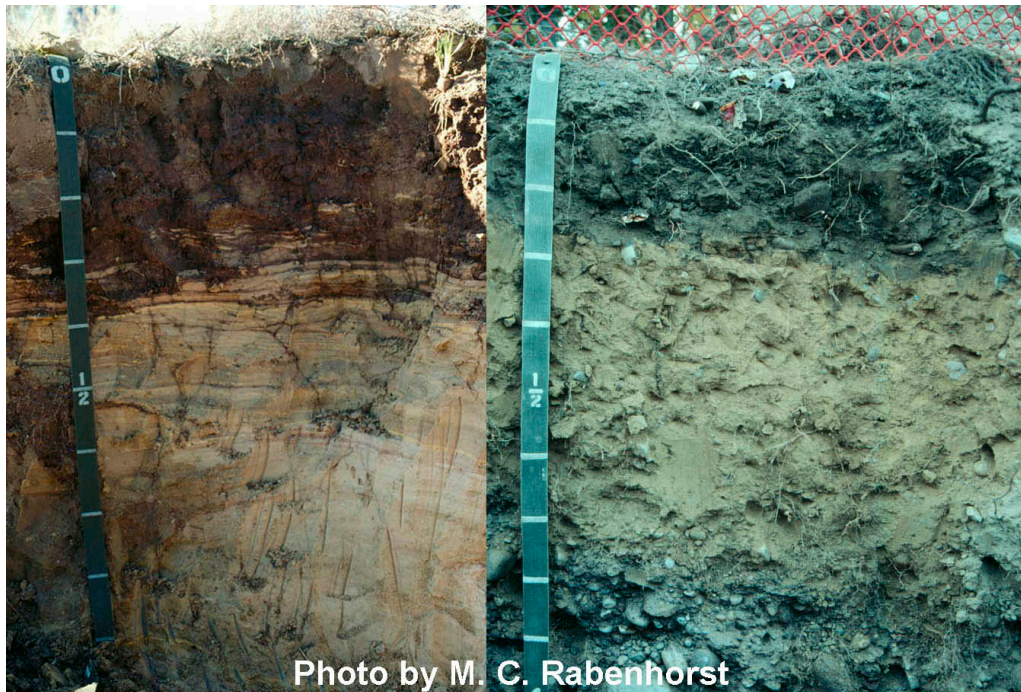
Figure 2-4. —The soil on the left formed in gray shale residuum. The shale bedrock is evident at a depth of about 16 in (40 cm). The soil on the right formed in sandy and gravelly sediments deposited by melting glaciers. Scale is in 4-in increments (10 cm).
