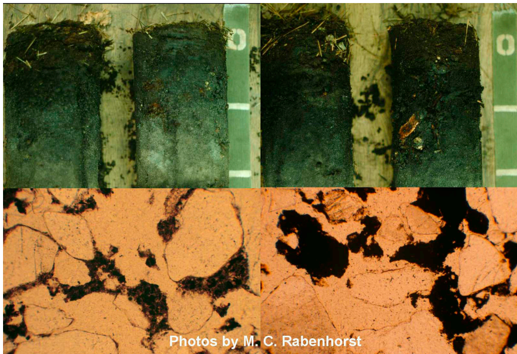
Figure 3-14. —The photographs in the upper part show cores taken from somewhat poorly drained and very poorly drained sandy soils. Note that the tape is in 4-in increments (10 cm). The thin section in the lower left corner of the illustration shows that the color of the organic matter is lighter and browner in the better drained soil, whereas that in the lower right corner is darker and blacker in the very poorly drained soil. Note frame length 0.2 in (5 mm); plane polarized light.
