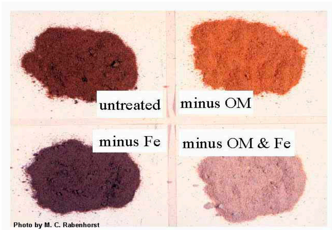
Figure 3-2. —The contributions of organic matter and iron oxides to soil color are evident in this soil sample of an Ap horizon from which organic matter and iron oxides have been removed.
