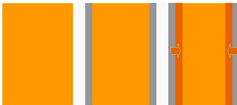
Figure 3-8. —Three steps in the formation of Type II mottles (where Fe oxides become depleted) from along a ped surface. Slow saturation of the peds relative to reduction conditions in the pores between the peds. The three steps shown illustrate: (1) the initial condition of the soil; (2) saturated and reducing conditions develop at the ped faces; and (3) moisture gradients move Fe(II) toward the ped interior where it reoxidizes to Fe(III).
