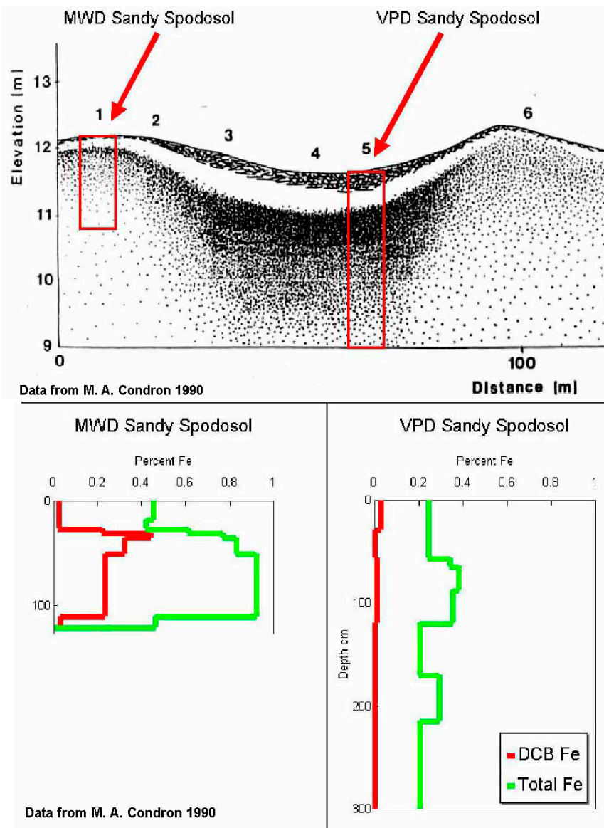
Figure 3-11.—Locations of moderately well drained and very poorly drained soils sampled from along a sandy dunal landscape. Data for total iron and DCB iron (extractable iron oxides) illustrate relative depletion of iron from the very poorly drained soil.
