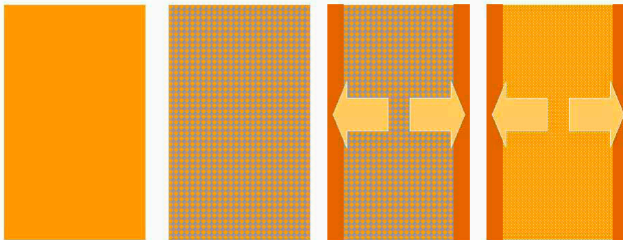
Figure 3-7a.—Four steps in the formation of Type I mottles where Fe oxides become concentrated along a ped surface: (1) the initial condition; (2) saturation of the ped and the development of reducing conditions throughout the interior of the ped; (3) drying that causes soil water to move toward the ped face, carrying soluble Fe(II) that then oxidizes to Fe(III); and (4) the final condition with Type I mottles formed at the ped face. (Diagram by M.C. Rabenhorst)
