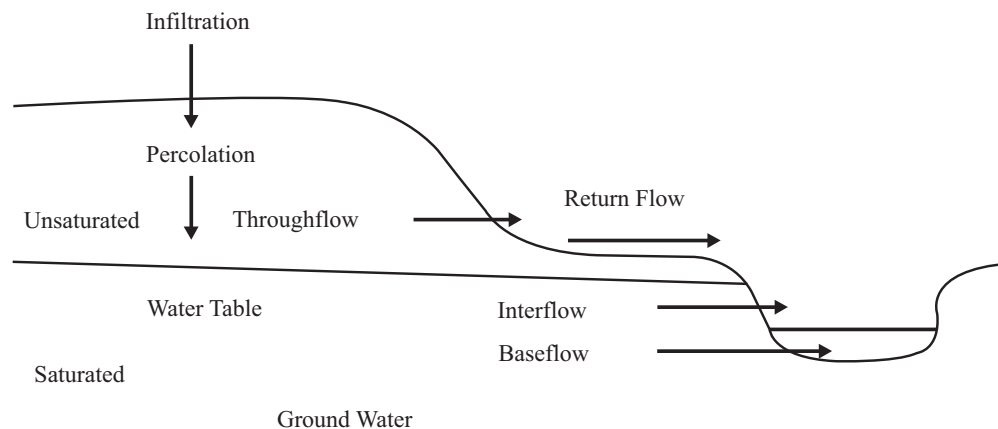
Figure 5-1.—Water flow patterns through soil.
