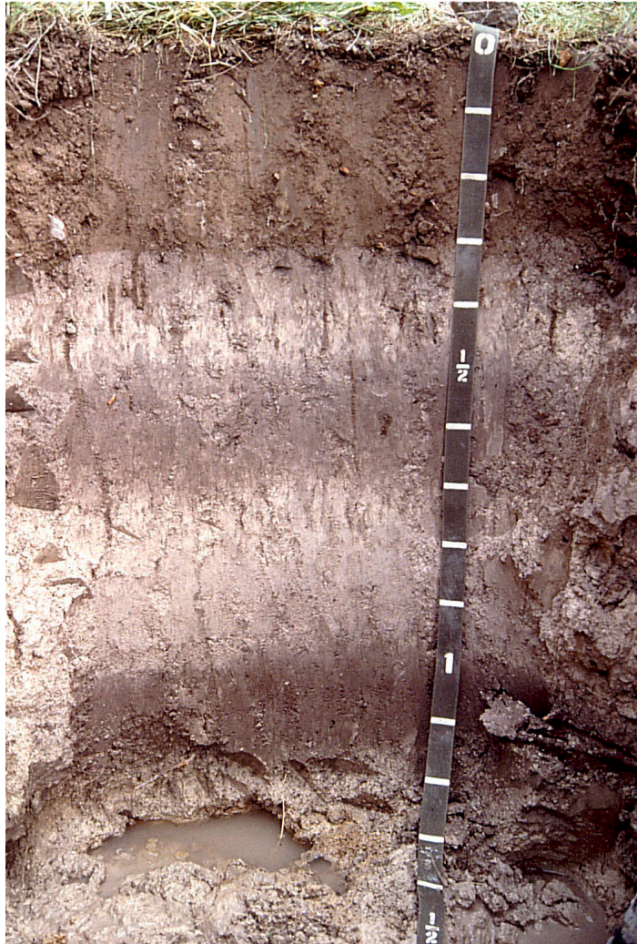
Figure 10-6. —A hydric soil derived from marl, located in a concave, backwater slough. The profile consists of 98 percent calcium carbonate throughout. Some pedons meet Field Indicator F3 (Depleted Matrix), F4 (Depleted Below Dark Surface), or F10 (Marl) if used for testing in the Mid-Atlantic Region.
