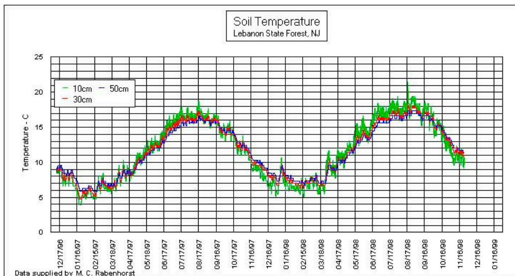
Figure 3-4. —A forested soil in New Jersey, where temperatures at depths of 10 to 50 cm did not reach “biological zero,” or 41 °F (5 °C), during a 2-year period.
