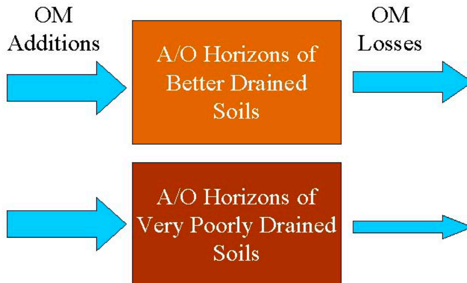
Figure 3-12.—Box model illustrating that the accumulation of organic matter (A or O horizon) in hydric soils is darker or thicker due to slower losses from anaerobic decomposition. (Diagram by M.C. Rabenhorst)
