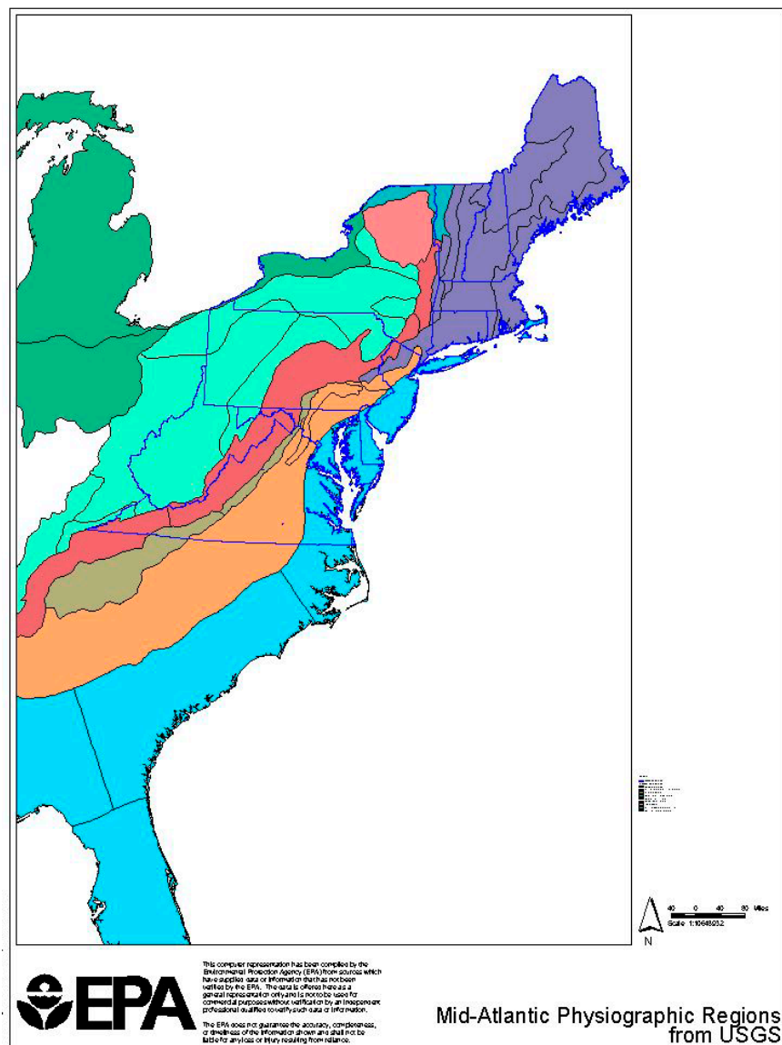
Figure 8-1.—Map of the mid-Atlantic physiographic regions.
