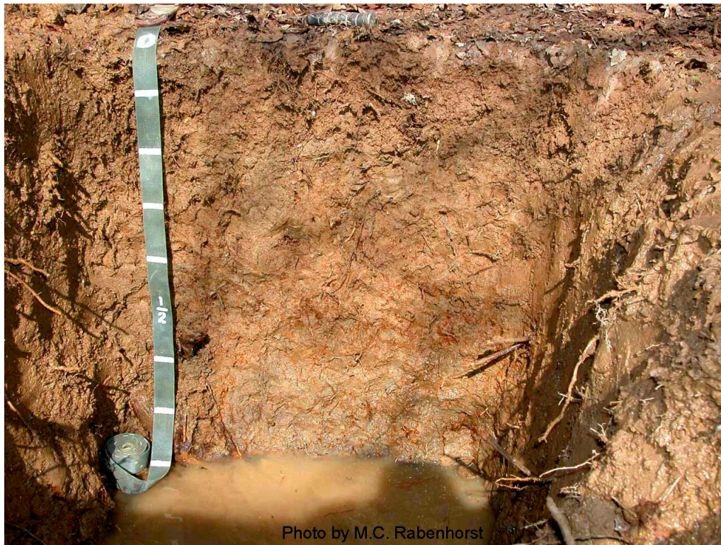
Figure 10-5. —A hydric soil from a University of Maryland study site on a Piedmont flood plain. It has a bright matrix near the surface.
