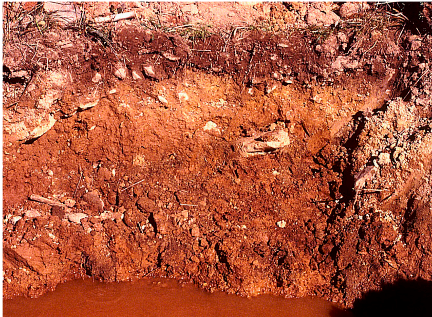
Figure 10-1. —A hydric soil formed in red parent material that meets Field Indicator TF2 (Red Parent Material) but does not have the typical gray matrix that would meet Field Indicator F3 (Depleted Matrix).
