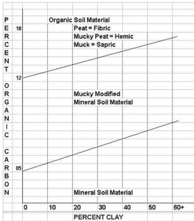
Figure 6-1.—Definition of organic and mineral soil materials based on percent organic carbon and clay. Mucky modifiers are used with some mineral material.
