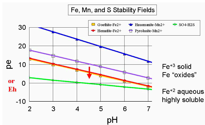
Figure 3-5.—The stability fields of various elements under particular pe (Eh) and pH conditions. In the zone above the orange and yellow lines, the oxidized form of iron is stable (solid phase iron oxides). In the zone below the lines, the reduced form of iron is stable (highly soluble ferrous iron). Note: \text{Eh} = 59 \cdot \text{pe} .
