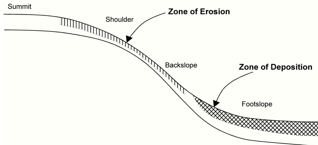
Figure 2-5. —A schematic diagram of a hillslope illustrating the various components. Erosional processes are generally most dramatic along the shoulder and backslope portions of the hillslope, and depositional processes are most pronounced in the footslope portion.
