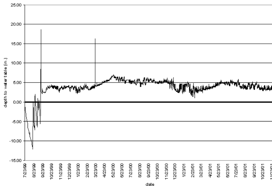
Figure 5-2.—Hydroperiod of permanently saturated wetland.
