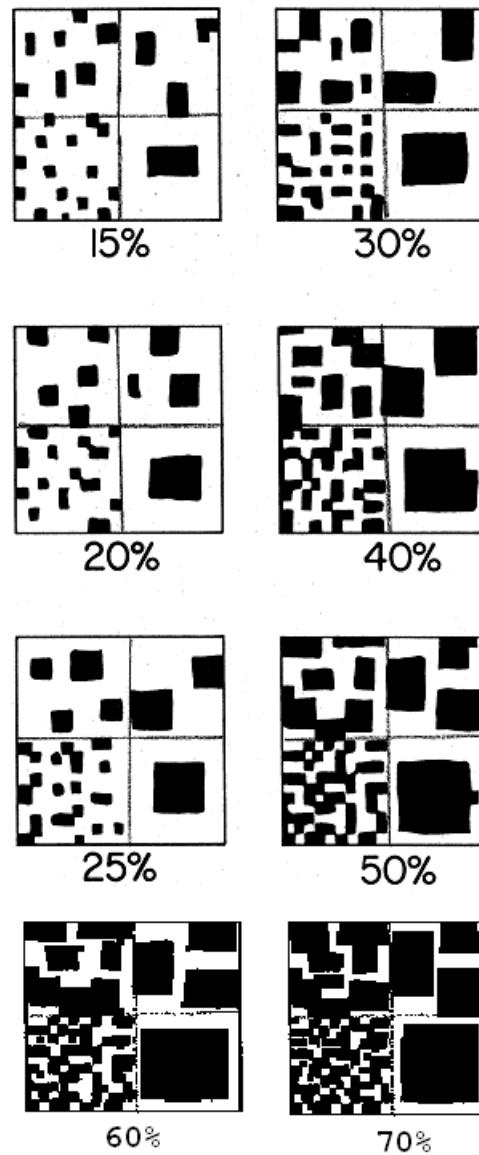
Figure 6-5.—Guide for estimating proportions from 15 to 70 percent.
