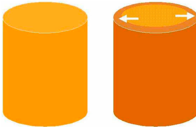
Figure 3-7b. —An illustration showing peds before and after processes that form Type I mottles. (Diagram by M.C. Rabenhorst)
