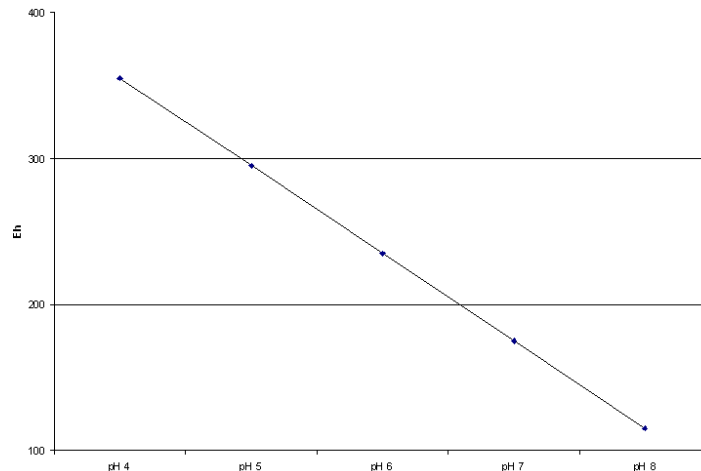
Figure 11-5.—Eh/pH threshold for anaerobic conditions.
