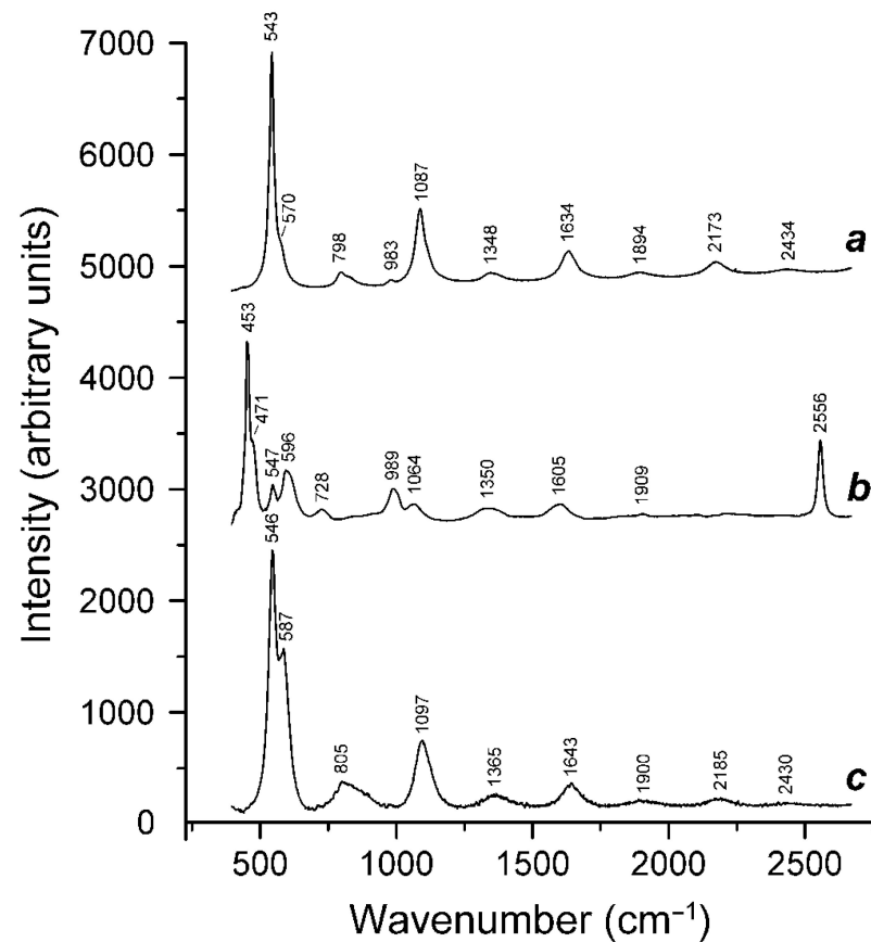
Figure 13. Raman spectra of (a) initial \text{S}_4 -bearing hauyne (Sample 5), (b) Sample 5 preheated for three days at 700 °C, over the Fe-FeS buffer and (c) preheated Sample 5 additionally annealed at 800 °C in air for one day.
