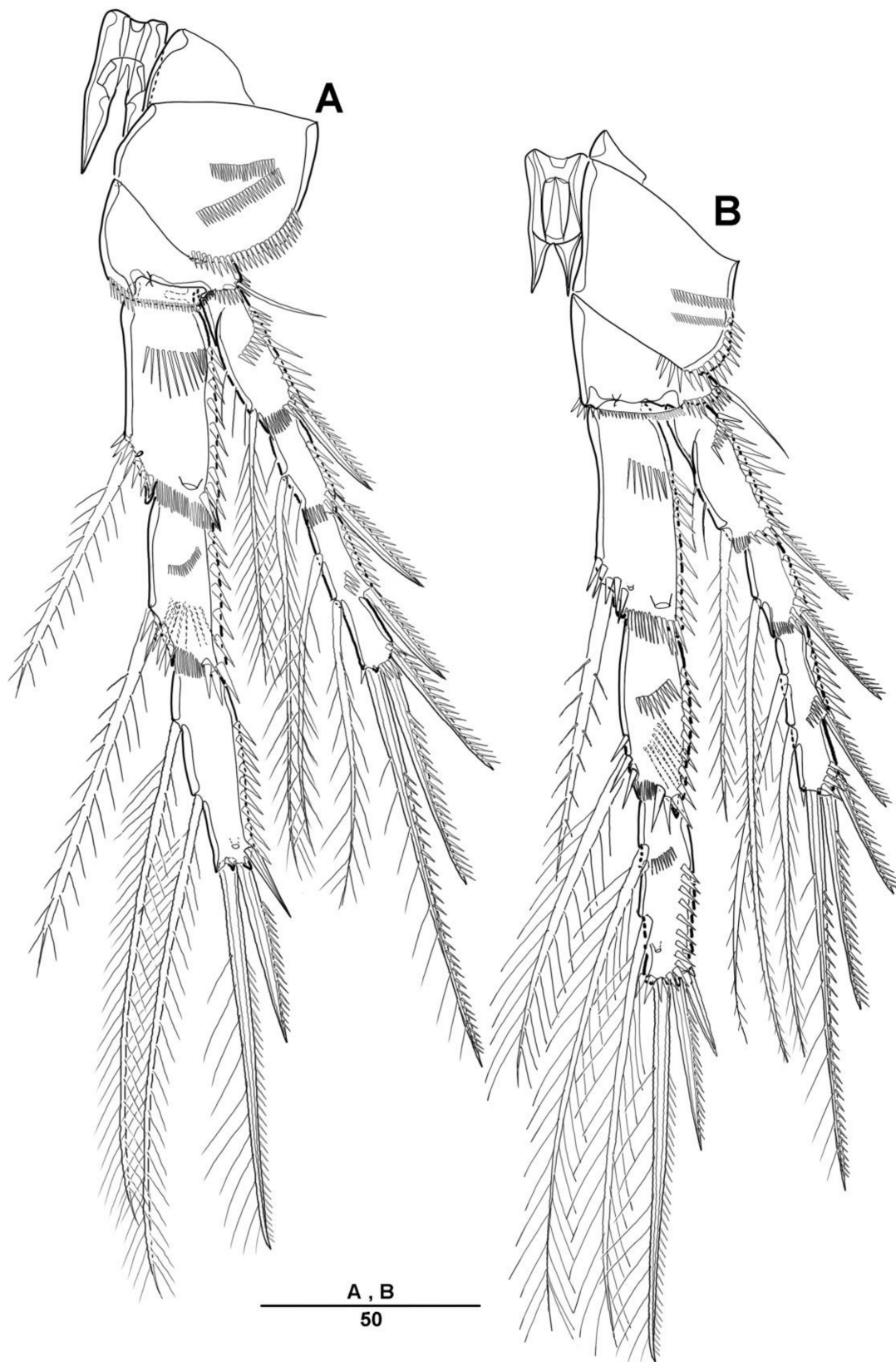
Figure 6. Halectinosoma munmui sp. nov. holotype female. (A) P3, anterior; (B) P4, anterior.
