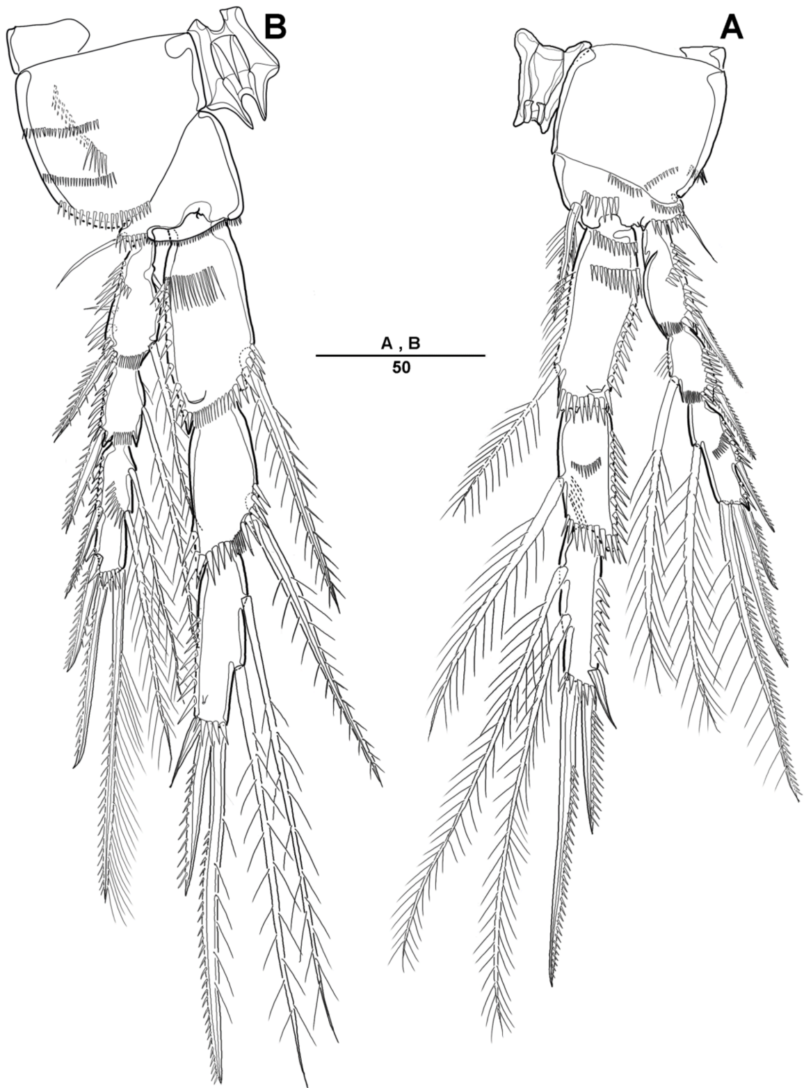
Figure 5. Halectinosoma munmui sp. nov. holotype female. (A) P1, anterior; (B) P2, anterior.
