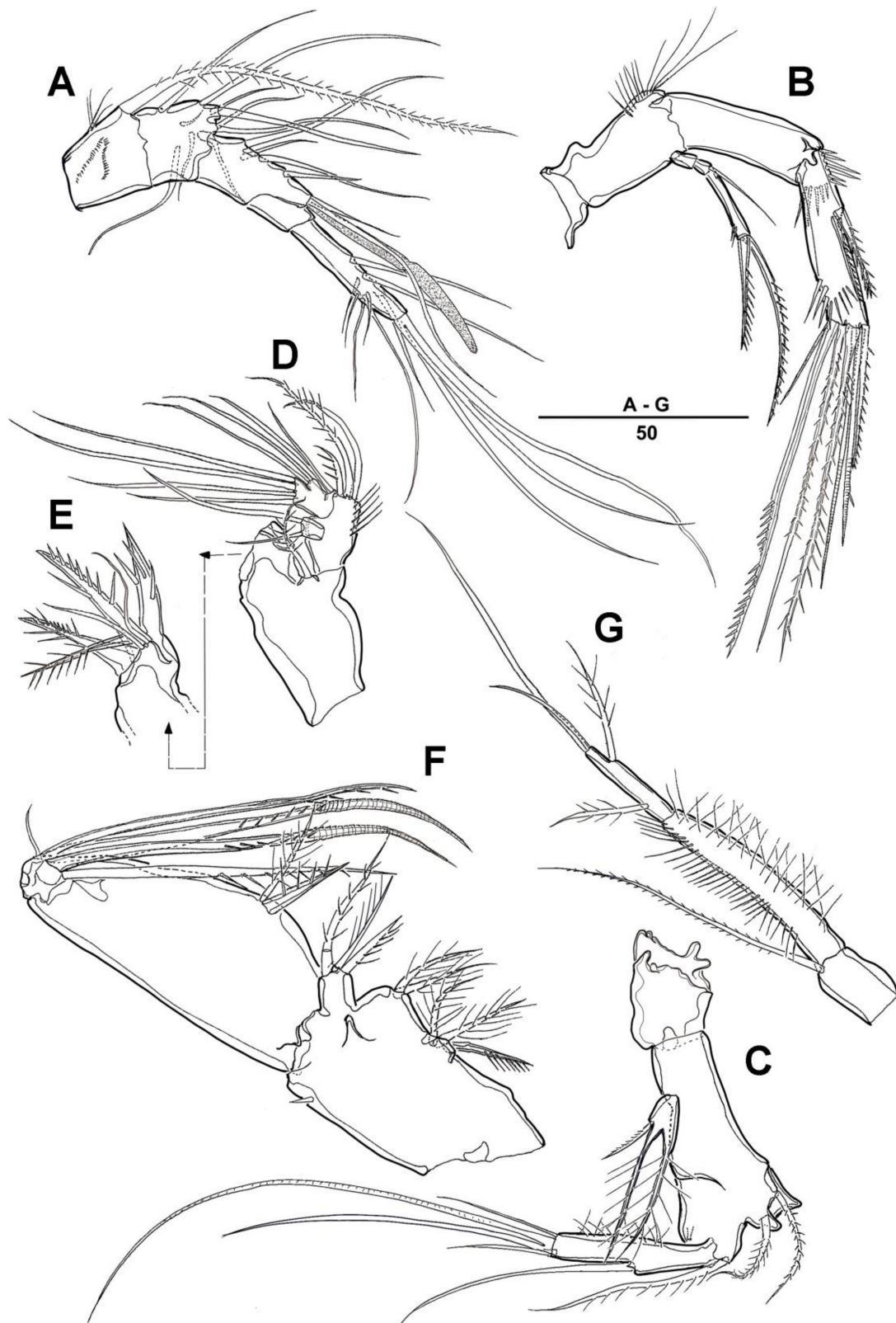
Figure 4. Halectinosoma munmui sp. nov. holotype female. (A) Antennule; (B) antenna; (C) mandible; (D) maxillule; (E) maxillule, praecoxal arthrite; (F) maxilla; (G) maxilliped.
