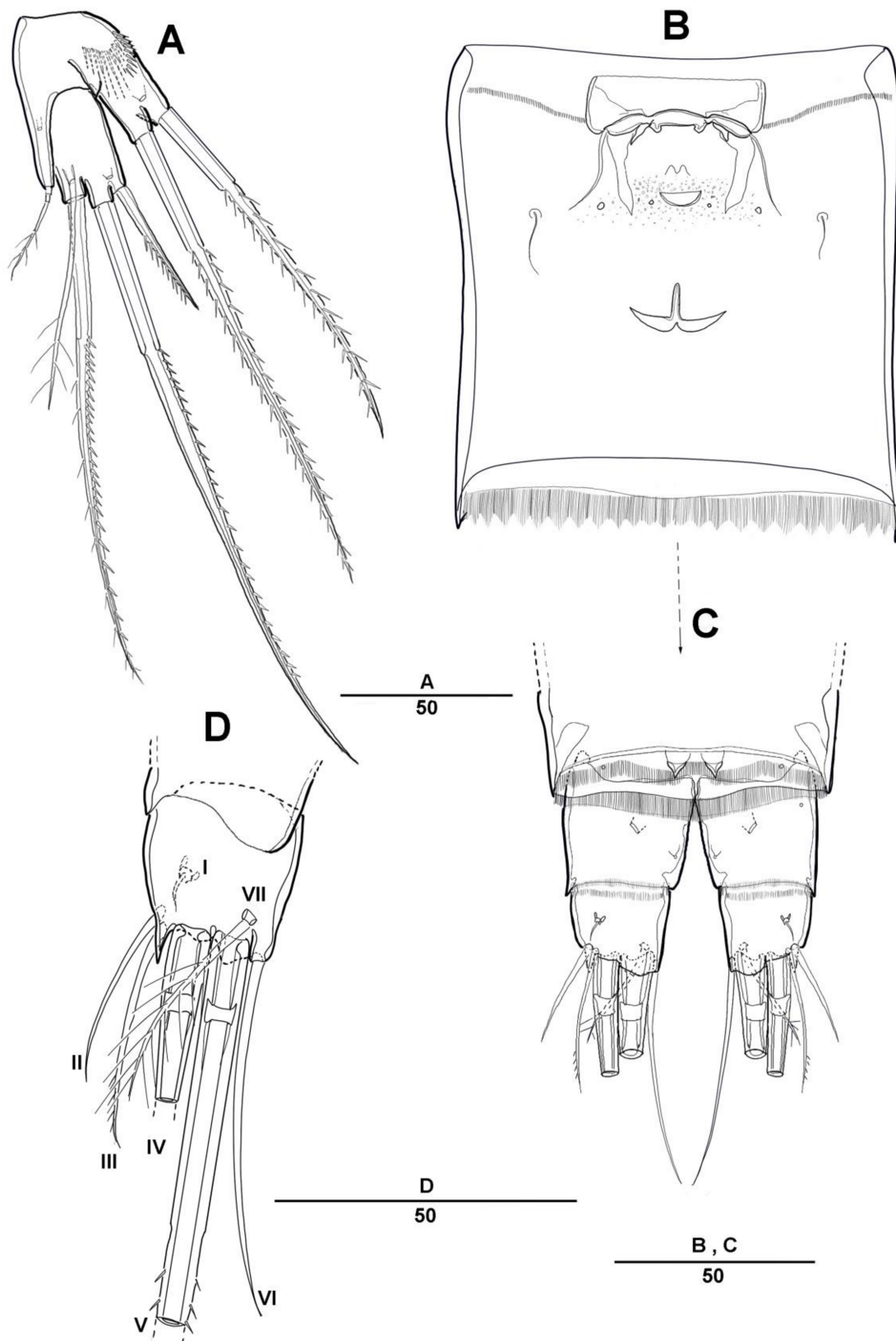
Figure 3. Halectinosoma munmui sp. nov. holotype female. (A) P5, anterior; (B) genital field, ventral; (C) anal somite and caudal rami, ventral; (D) caudal ramus, dorsal.
