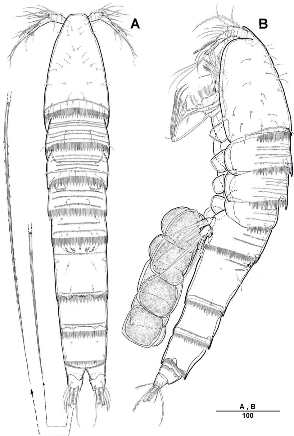
Figure 2. Halectinosoma munmui sp. nov. holotype female. (A) Habitus, dorsal; (B) habitus, lateral.
