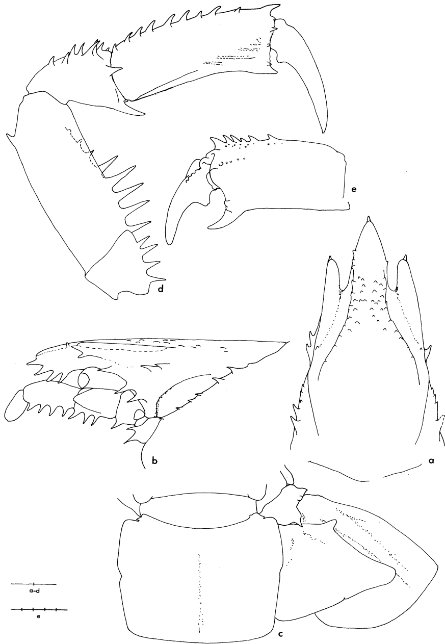
Fig. 53. Upogebia spinifrons (AM P.12943, female, 19 mm): a, b , dorsal and lateral views of anterior region; c , telson and uropod; d , pereopod 1. (QM W.1435, female, 24 mm): e , propod and dactyl of pereopod 1 (lateral).
