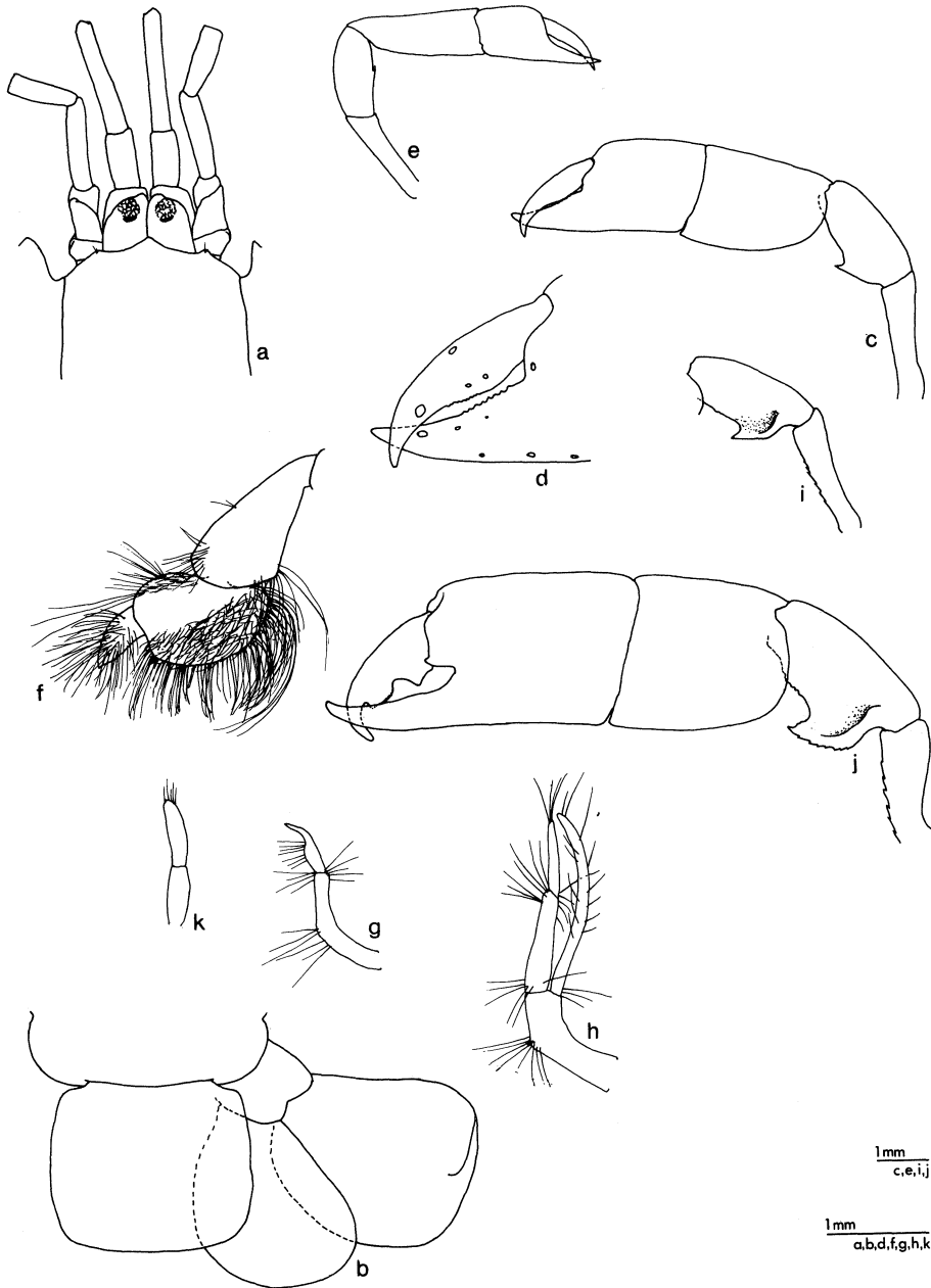
Fig. 15. Callianassa arenosa (NMV J.271, female, 24 mm (holotype) ): a , front; b , tail fan; c , d , large cheliped (left); e , small cheliped (right); f , pereopod 3; g , h , pleopods 1, 2. (PPBES stn 982, female, 20 mm): i , large cheliped ischium and merus. (NMV J.272, male, 22 mm (allotype) ): j , large cheliped (left); k , pleopod 1.
