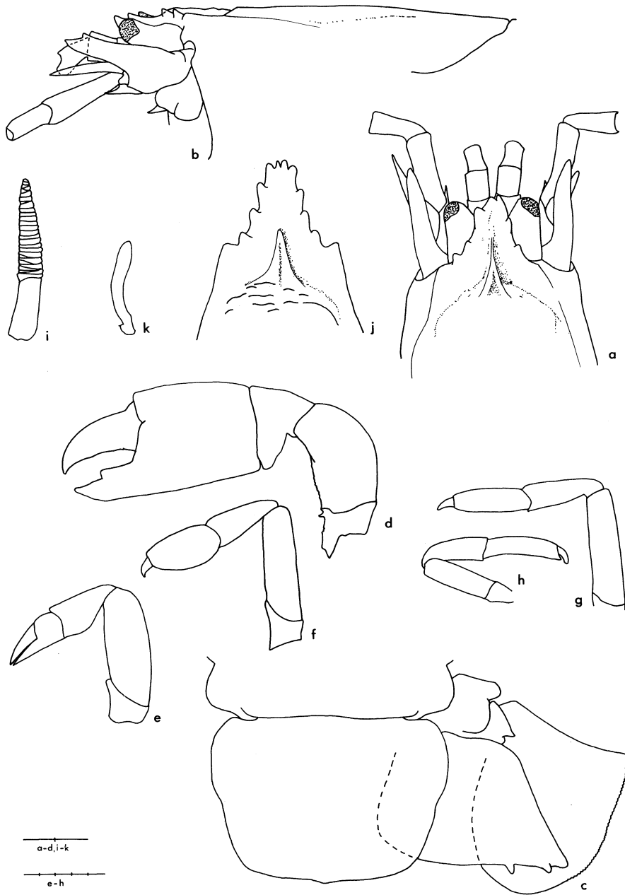
Fig. 9. Axius plectrorhynchus (WAM 23-75, female, 19 mm): a, b, dorsal and lateral views of anterior region; c, telson and uropod; d-h, pereopods 1-5; i, pleopod 1. (WAM 167-60, female, 22 mm): j, dorsal view of anterior. (WAM 167-60, male, 17 mm): k, pleopod 1.
