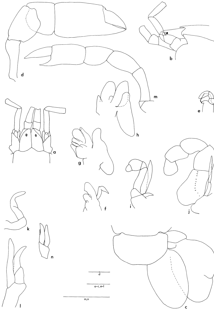
Fig. 36. Callianassa tooradin (NMV J.301, female, 19 mm): a, b , dorsal and lateral views of anterior region; c , telson and uropod; d , cheliped; e , mandible; f, g , maxillae, 1, 2; h-j maxillipeds 1-3; k, l , pleopods 1, 2. (NMV J.302, male, 7 mm): m , small cheliped; n , pleopod 2.
