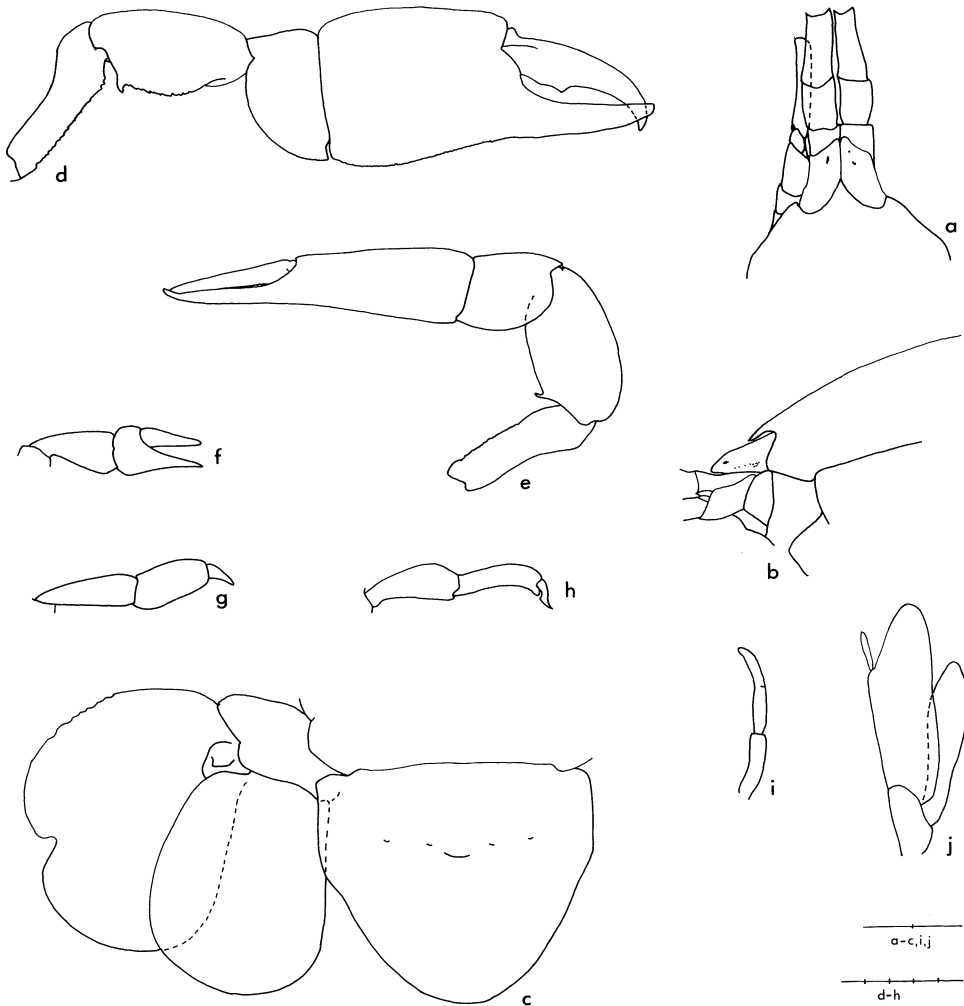
Fig. 38. Gouretia coolibah (WAM 66-75, female, 48 mm): a, b, dorsal and lateral views of anterior region; c, telson and uropod; d, large cheliped; e, small cheliped; f, g, h, pereopods 2, 4, 5; i, j, pleopods 1, 2.
