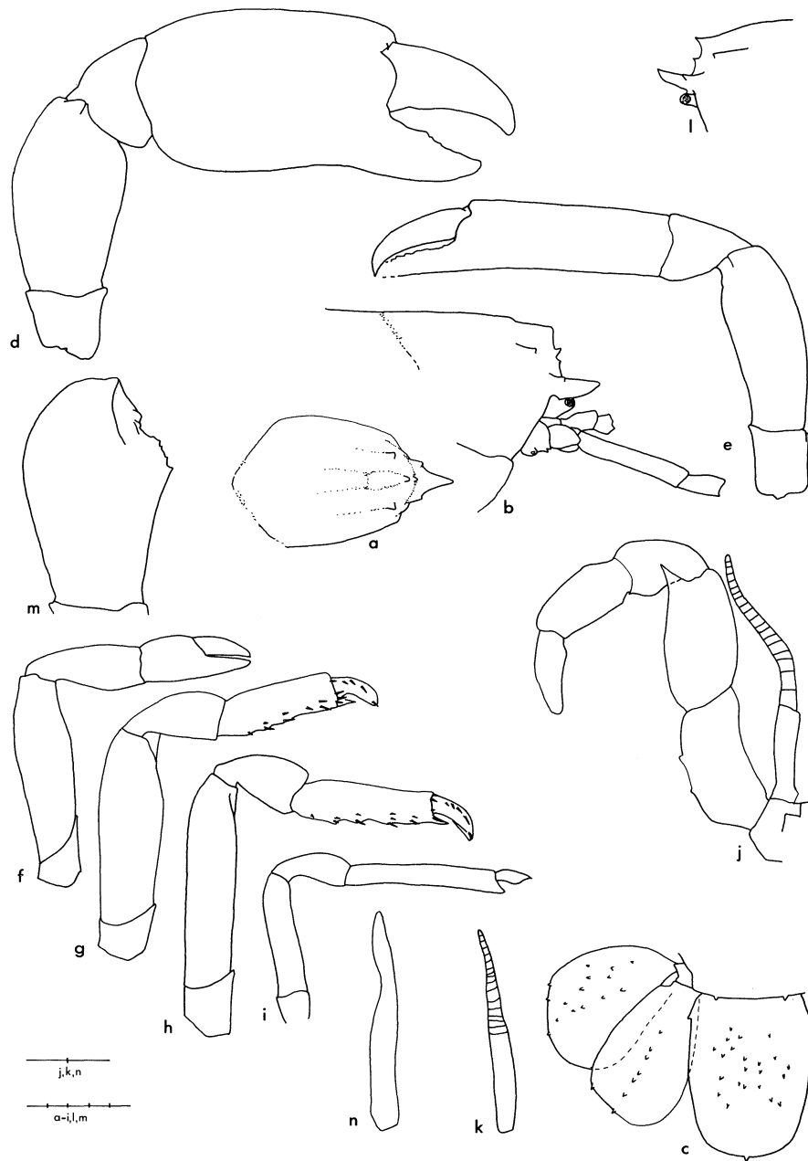
Fig. 11. Scytoleptus serripes (QM W.4531, female, 20 mm): a, b , dorsal and lateral views of anterior region; c , telson and uropod; d , large cheliped; e , small cheliped; f-i , pereopods 2-5; j , maxilliped 3; k , pleopod 1. (QM W.4531, female, 16 mm): l , lateral view of anterior. (WAM 74-75, female, 18 mm): m , merus of large cheliped. (WAM 47-75, male, 21 mm): n , pleopod 1.
