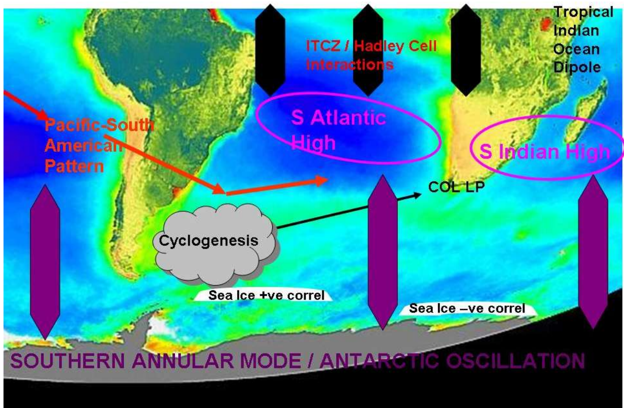
Figure 2.2 Schematic of important features for austral winter rainfall (after Reason and Rouault 2007)
