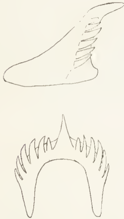
Text fig. 15.— Facelina newcombi (Angas). Lateral and dorsal views of a radula tooth.
