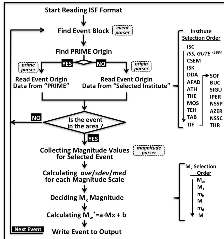
120 Figure 2. Flowchart of the ISC database processing. Ave: Average (mean), Med: Median, Sdev: Standard deviation. Mw* is equivalent moment magnitude. See Appendix A for the institute codes.
