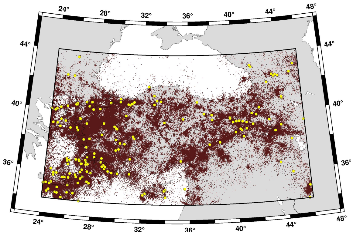
145 Figure 3. The earthquakes in the homogenised catalogue (dots). Yellow circles are the events with an equivalent moment magnitude ( M_w^* ) greater than 6.0 (total 179 events).
