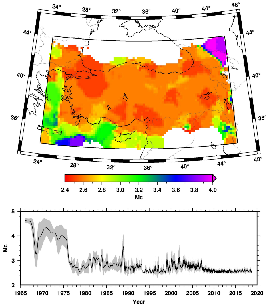
Figure 8. Top: Mc spatial distribution map for the events since 1964. There is no data in white areas. Bottom: Temporal Mc variation as a function of year. Grey area is the \pm\sigma interval estimated by bootstrapping.
