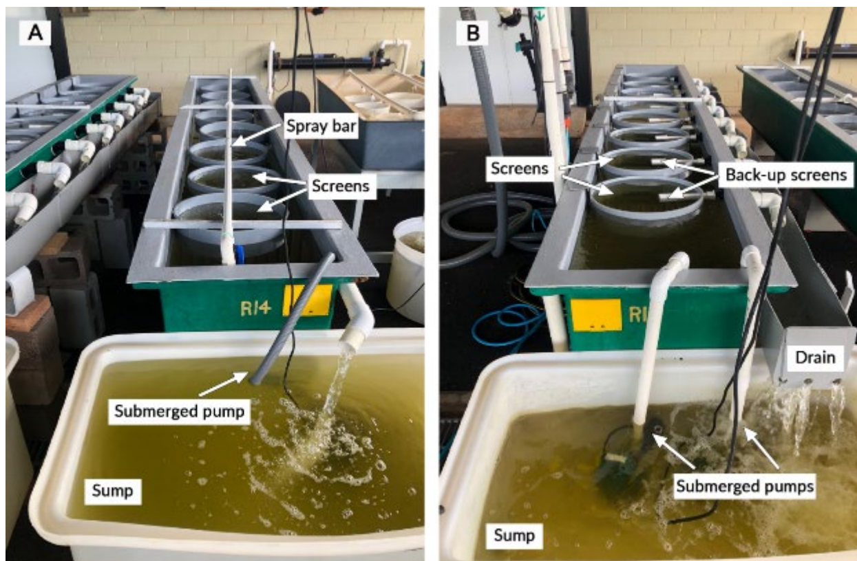
Figure 21. (A) Downweller nursery system and (B) upweller nursery system.
