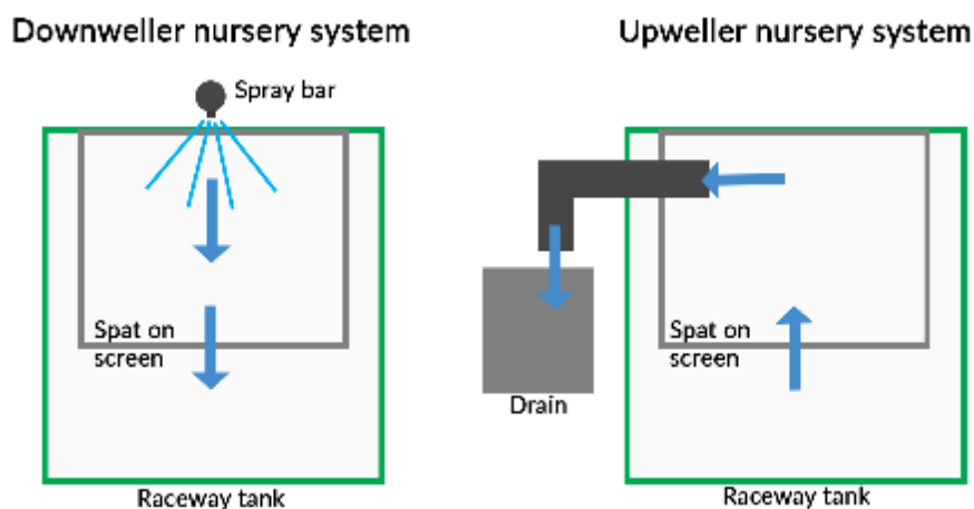
Figure 20. Downweller and upweller nursery system diagram. Arrows indicate the flow of seawater through the systems.
