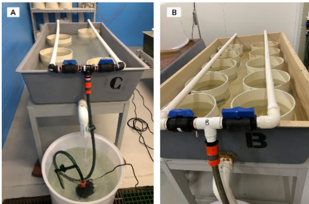
Figure 18. (A) Recirculating downweller system for settlement and (B) close up of spray bars and holding screens in the downweller system.
