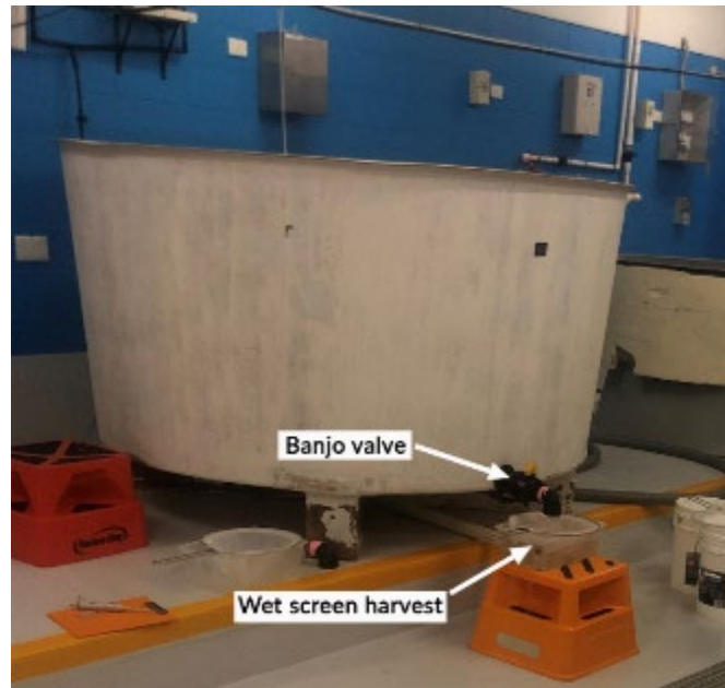
Figure 14. Wet screen harvesting showing larvae passing through 50 mm valve outlet into a nylon mesh larval net.
