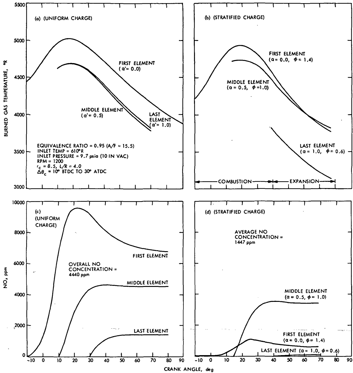
Fig. 4-12. Comparison of temperature and NO profiles for uniform-charge and linearly stratified-charge Otto engines with similar operating and design parameters (from Refs. 4-18 and 4-20): (a) Temperature profiles for uniform charge at \phi = 0.95 . (b) Temperature profiles for linearly stratified charge of width = 1.4/0 and \phi = 1.0 . (c) NO profiles for uniform charge as above. (d) NO profiles for linearly stratified charge as above.
