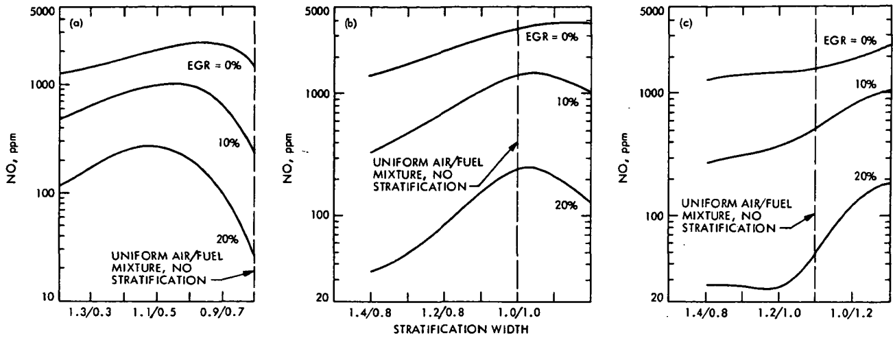
Fig. 4-13. Effect of linear stratification on total NO production at three EGR rates for three overall equivalence ratios (from Ref. 4-20). Engine parameters: EGR temperature = 610^{\circ}\text{R} , intake manifold temperature = 610^{\circ}\text{R} , intake manifold pressure = 9.7 psia, RPM = 1500, r_c = 8.5 , L/R = 4.0 , \Delta\theta_c = 10^{\circ}\text{ BTDC to } 40^{\circ}\text{ ATDC} . (a) Effect of linear stratification on NO production for \phi = 0.8 , \bar{A}/\bar{F} = 18.4 . (b) Effect of linear stratification on NO production for \phi = 1.0 , \bar{A}/\bar{F} = 14.7 . (c) Effect of linear stratification on NO production for \phi = 1.1 , \bar{A}/\bar{F} = 13.4
