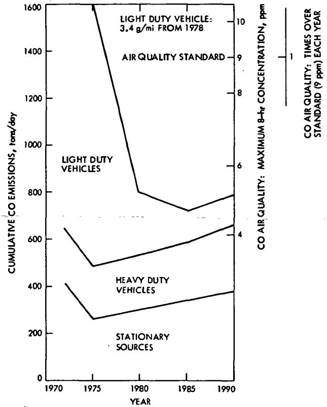
Fig. 19-24. St. Louis Urban-in Fact Area carbon monoxide (CO) emissions projection
