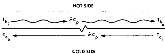
Fig. 2-2. An infinite area counterflow heat exchanger
