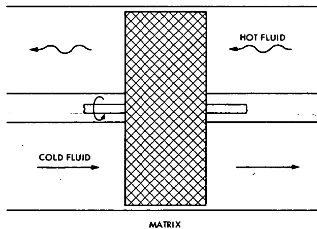
Fig. 2-4. Rotary, periodic flow regenerator
