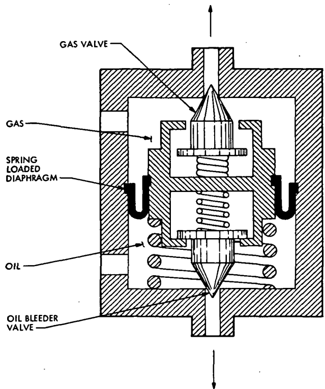
Fig. 6-22. Regulating valve (Philips Laboratories)
