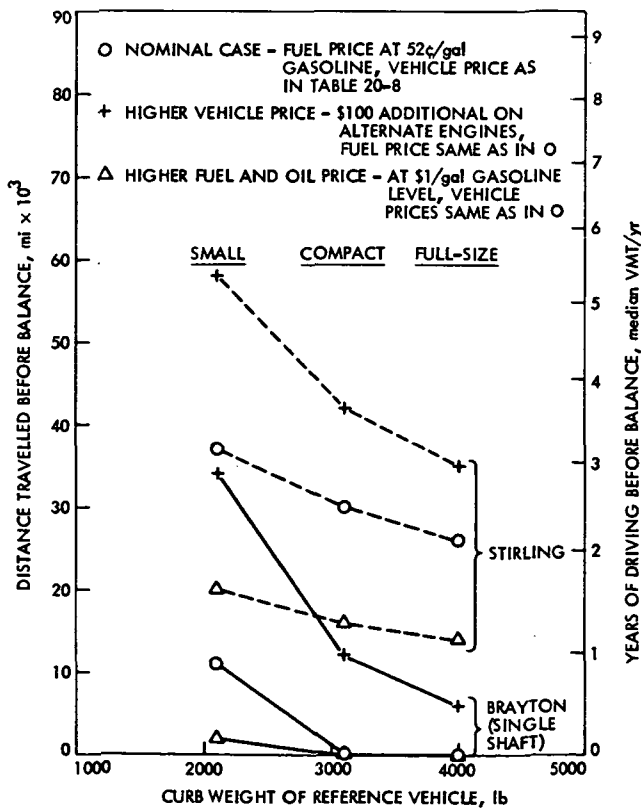
Fig. 20-10. Break-even mileage for Stirling and single-shaft Brayton engines vs baseline UC Otto vehicles
