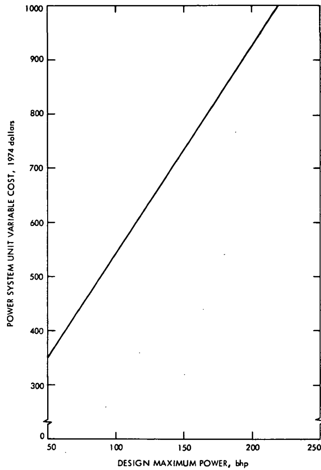
Fig. 7-17. Mature Rankine power system variable cost
