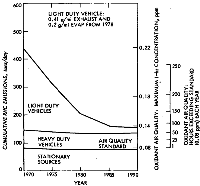
Fig. 19-18. New York study area effective hydrocarbon (RHC) emissions projection
