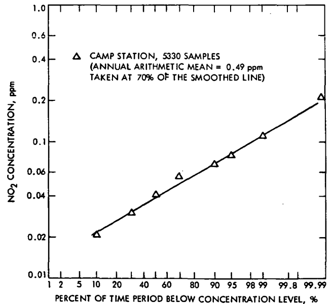
Fig. 19-20. Frequency distribution of nitrogen dioxide (NO 2 ) measurements, 1-hr average, St. Louis, 1972 data
