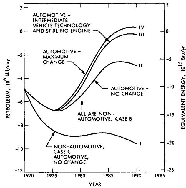
Fig. 17-16. Projections of the difference between domestic petroleum production and various demand alternatives
