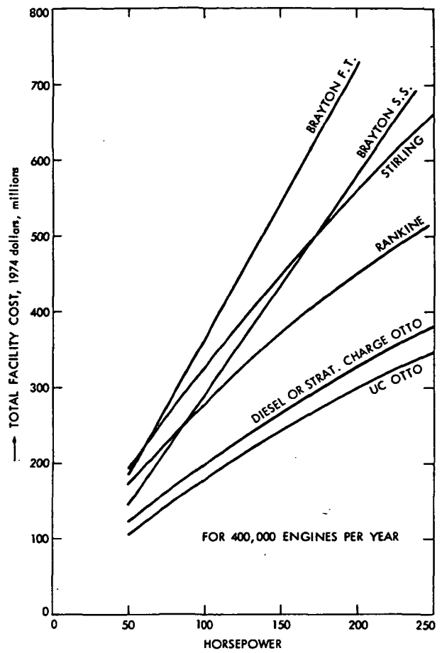
Fig. 11-3. Facility cost vs design maximum horsepower
