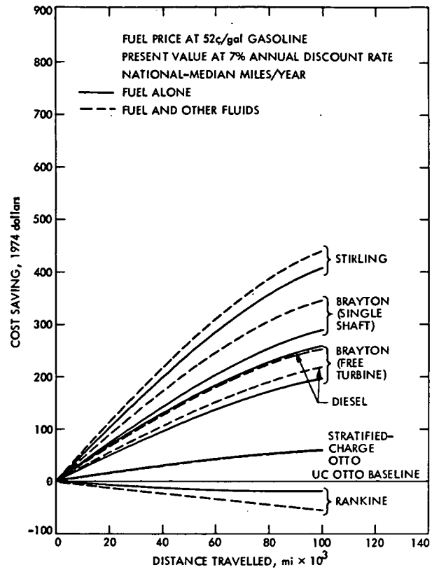
Fig. 20-7. Differential costs of fuel, oil, and coolant over equivalent UC Otto baseline vehicle: small cars
