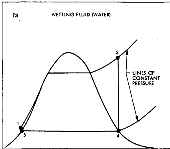
Fig. 7-2. Rankine cycles for "drying" and "wetting" working fluids
