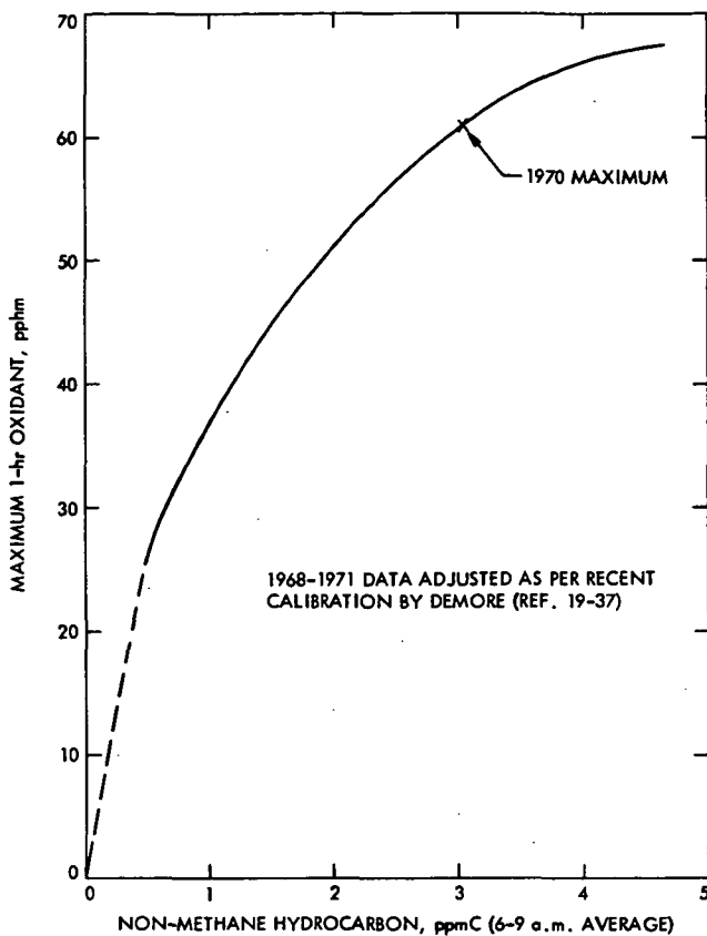
Fig. 19-7. Upper limit 1-hour oxidant curve for Azusa station
