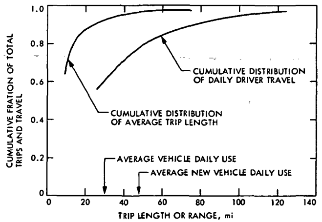
Fig. 14-26. Cumulative distribution of vehicle use by average trip length and daily driver travel
