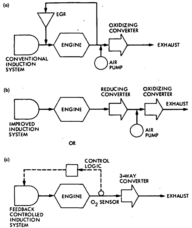
Fig. 3-11. Emission control systems (simplified conceptual): (a) oxidizing converter plus EGR (Present configuration); (b) dual converter approach; (c) 3-way catalyst approach; (b) or (c) is used in Mature and Advanced configurations
