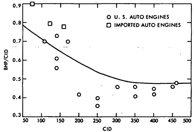
Fig. 4-28. BHP/CID for various U.S. and imported automobile engines - the solid line represents the Mature SC Otto engine
