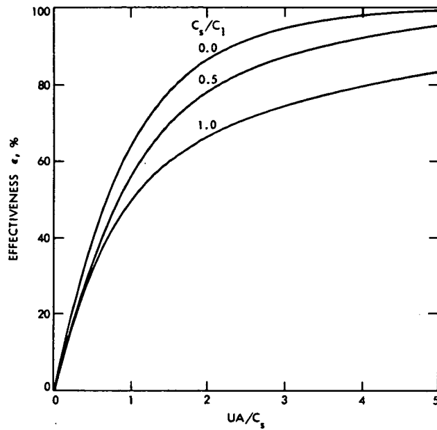
Fig. 2-3. Effectiveness of a counterflow heat exchanger
