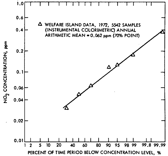
Fig. 19-11. Frequency distribution of nitrogen dioxide (NO 2 ) measurements, 1-hr average, New York City
