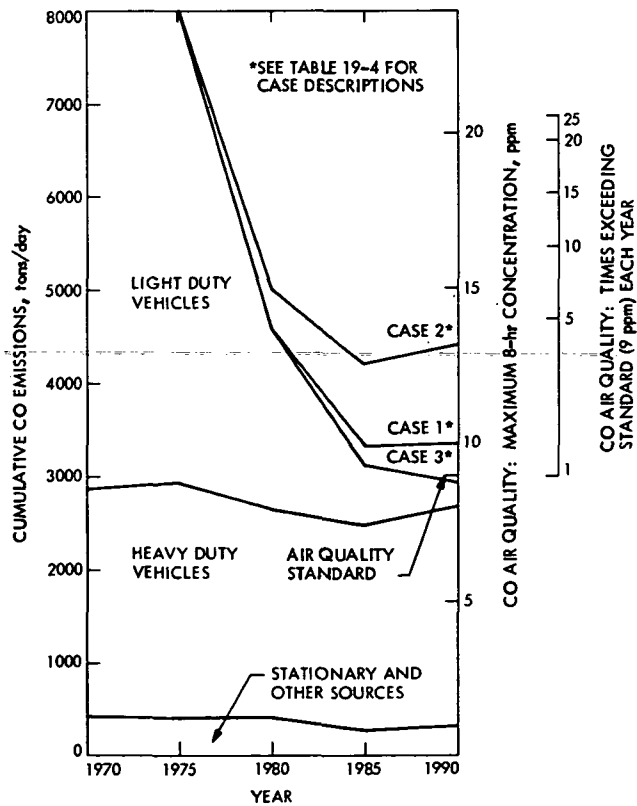
Fig. 19-8. Los Angeles AQCR carbon monoxide (CO) emissions projection
