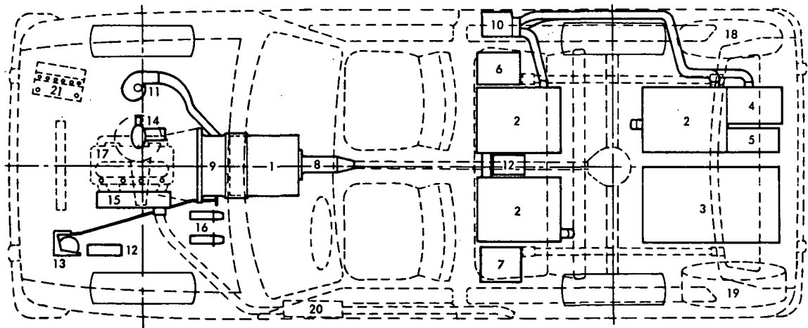
(a) GENERAL MOTORS STIR-LEC I CONFIGURATION
