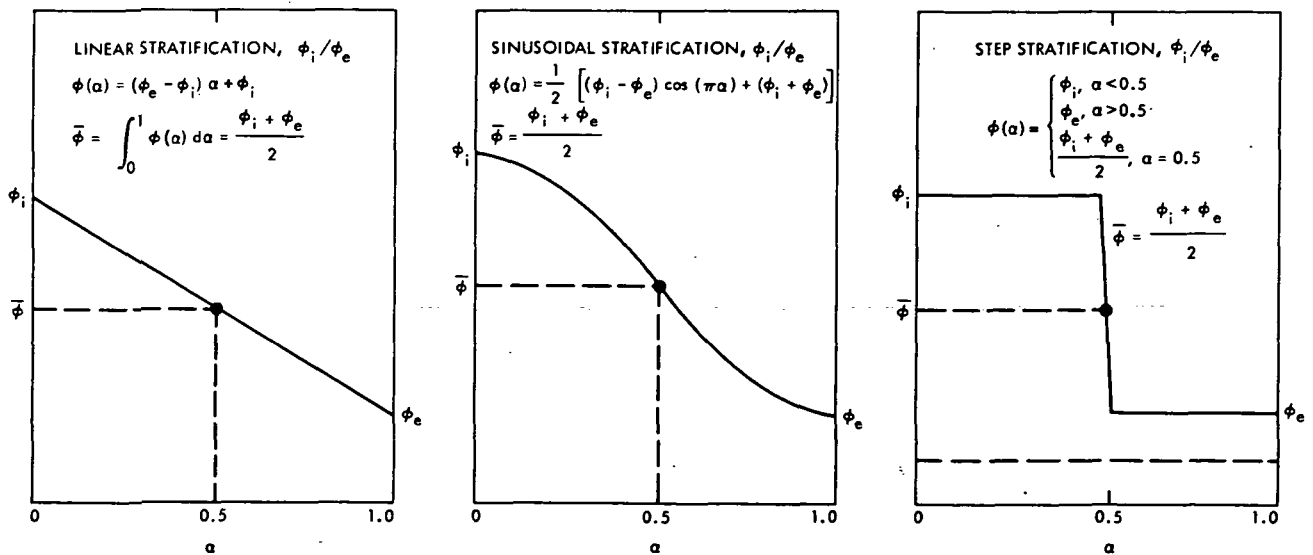
Fig. 4-8. Stratification functions (from Ref. 4-20)
