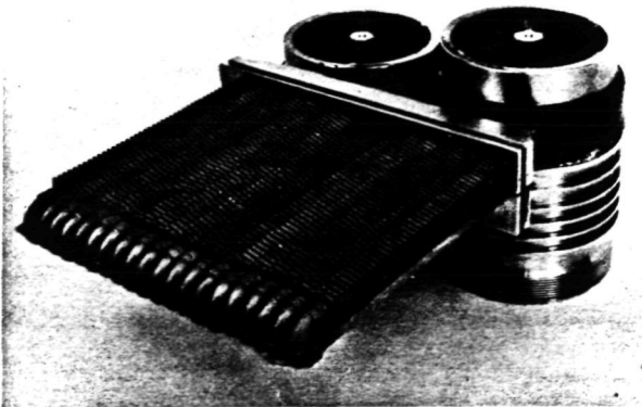
Fig. 6-30. MAN-MWN investment cast Haynes 31 heater head design
