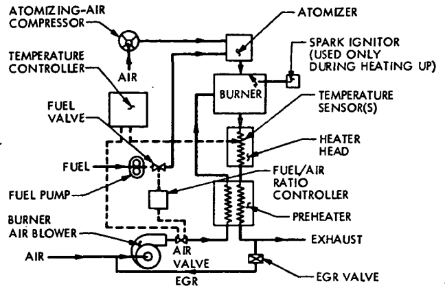
Fig. 6-18. Component schematic of combustion system (Ref. 6-7)
