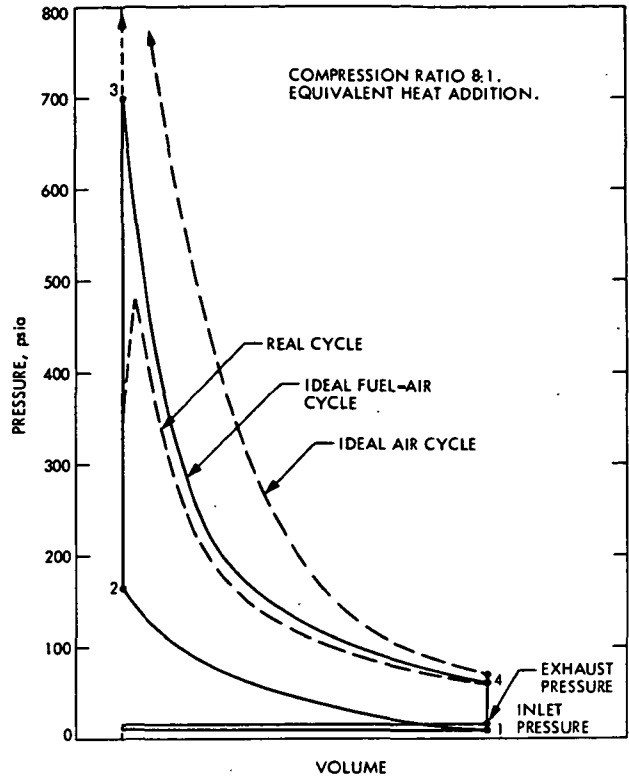
Fig. 3-4. Deviation of real Otto cycle operation from the ideal air cycle, and the ideal fuel-air cycle (compression ratio 8:1; equivalent heat addition)
