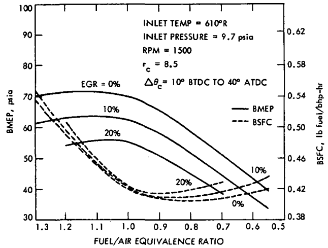
Fig. 4-11. BMEP and BSFC as affected by fuel/air equivalence ratio \phi and % EGR; \phi = 1.0 corresponds to A/F = 14.7 (from Ref. 4-18)
