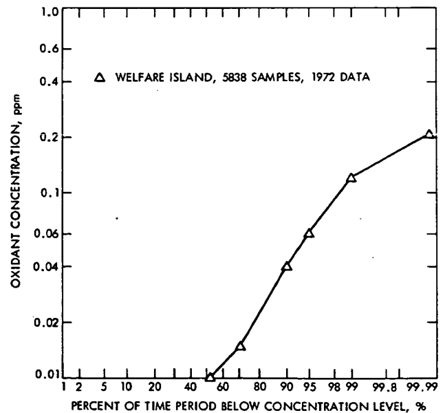
Fig. 19-12. Frequency distribution of oxidant (O x ) measurements, 1-hr average, New York City
