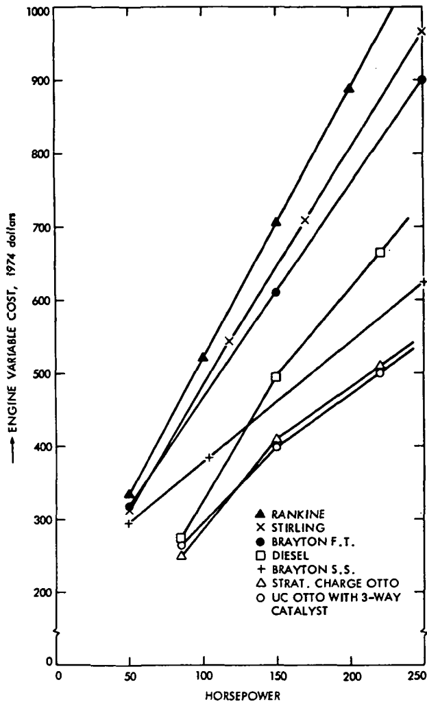
Fig. 11-2. Engine variable cost vs design maximum horsepower
