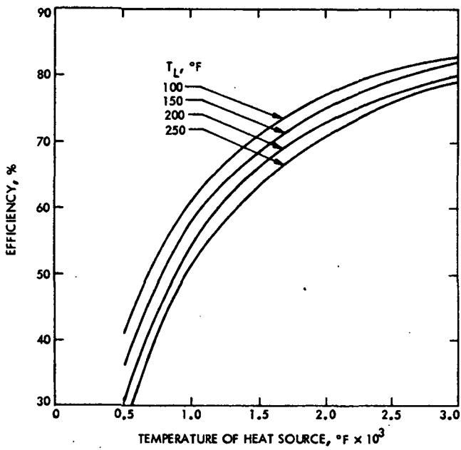
Fig. 6-10. Variation of ideal Stirling cycle efficiency with heat source ( T_N ) and heat sink ( T_L ) temperatures
