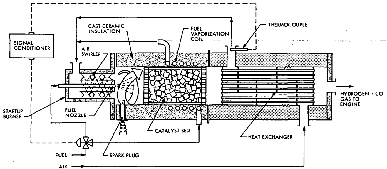
Fig. 4-34. Catalytic hydrogen generator
