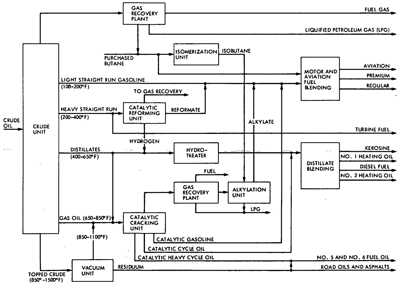
Fig. 17-17. Sample refinery
