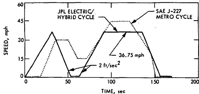
Fig. 8-3. Speed-time profile
