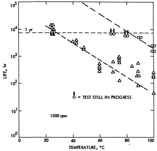
Fig. 6-31. Life of polyurethane-rubber roll-socks tested as a function of temperature; speed 1500 rpm; stroke 65 mm
