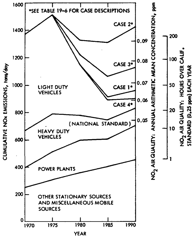
Fig. 19-9. Los Angeles AQCR oxides of nitrogen (NO x ) emissions projection
