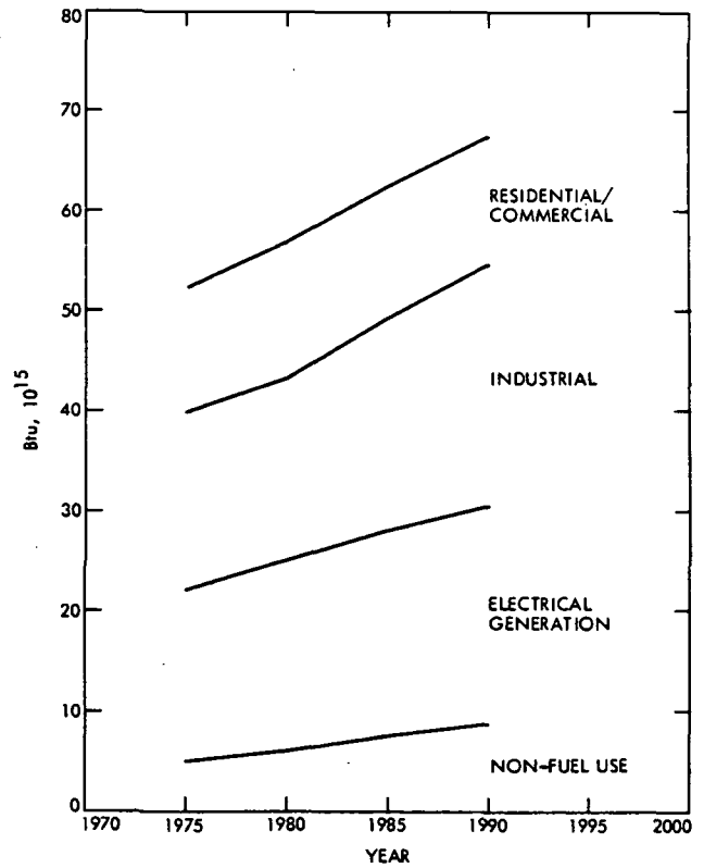
Fig. 17-8. Non-transportation demand for fossil fuel, case B
