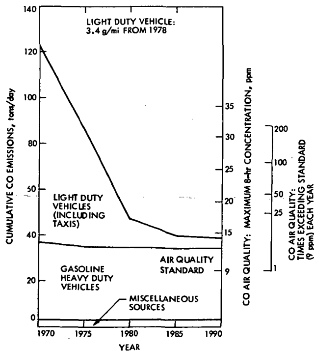
Fig. 19-16. Downtown Manhattan carbon monoxide (CO) emissions projection
