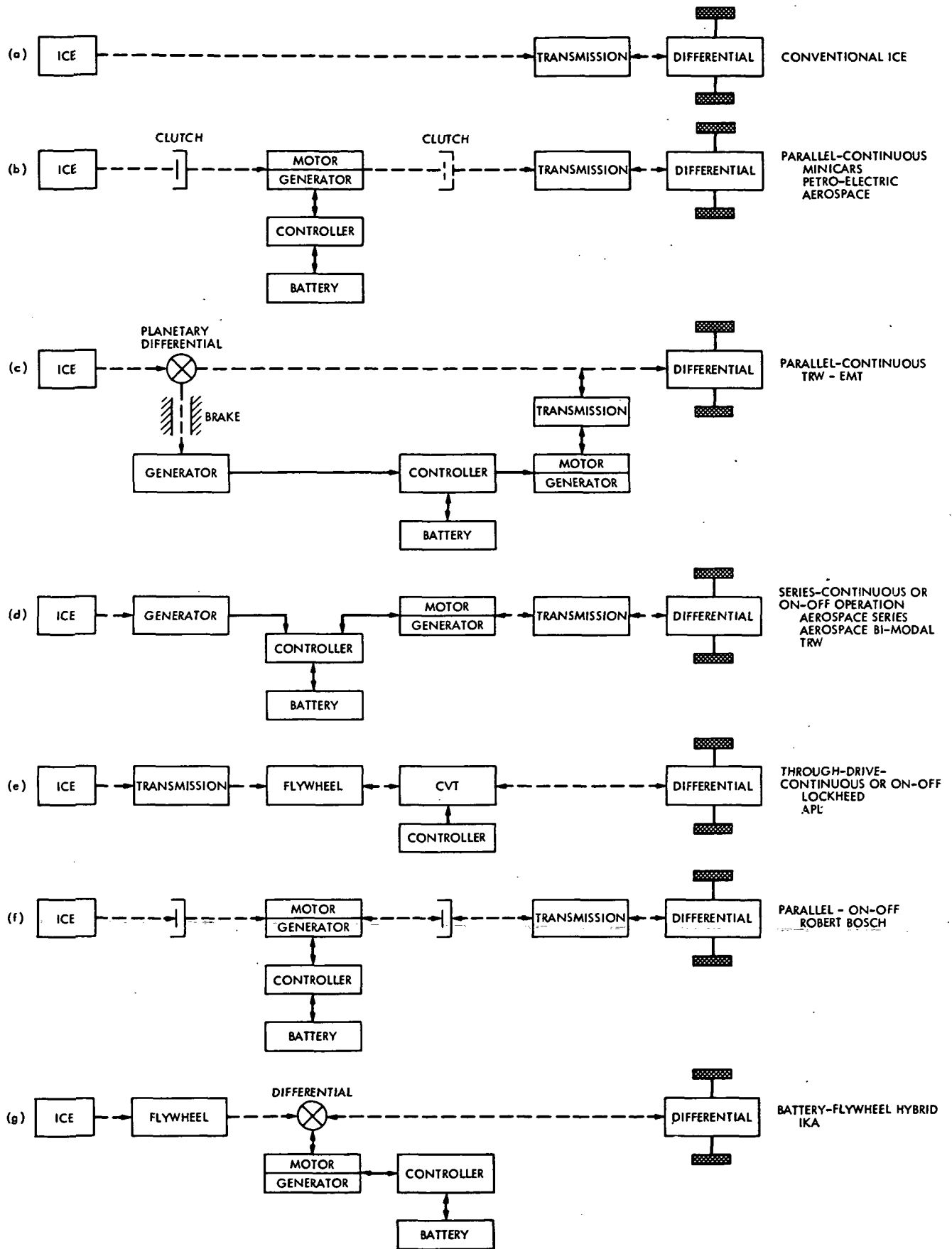
Fig. 9-2. Hybrid configurations
