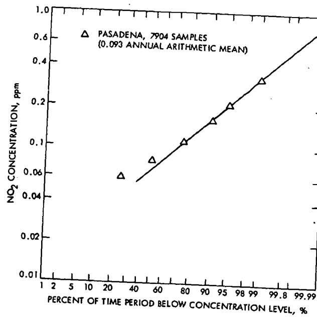
Fig. 19-4. Frequency distribution of nitrogen dioxide (NO 2 ) measurements, 1-hr average, Los Angeles Air Basin, 1970 data
