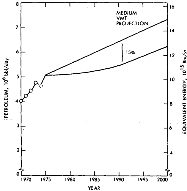
Fig. 17-10. Total automobile fuel consumption as affected by VMT (current market, "Present" UC Otto engine, current vehicle technology)
