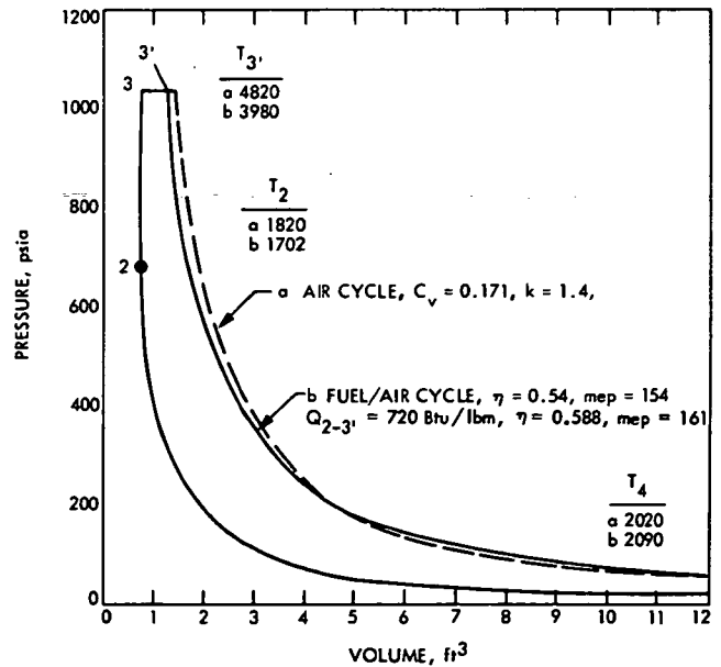
Fig. 4-22. Limited-pressure fuel/air cycle; r_c = 16 , \phi = 0.6 , p_1 = 14.7 , T_1 = 600 , p_3/p_1 = 70 ; temperatures are in degrees Rankine (from Ref. 4-17)
