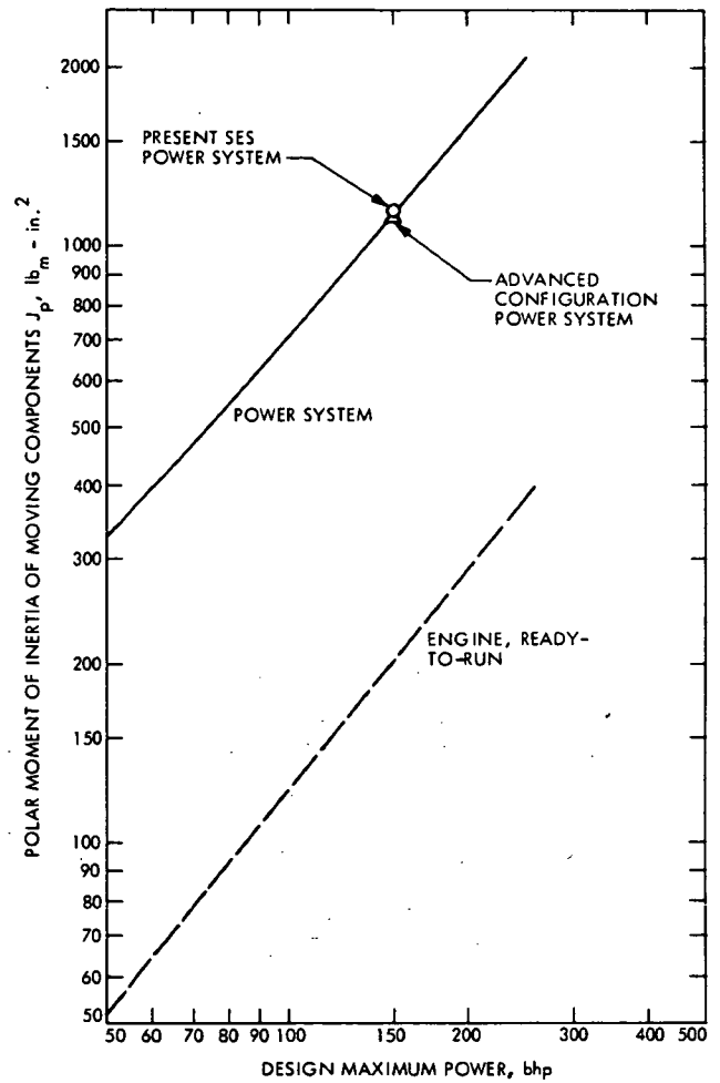
Fig. 7-16. Projected Rankine engine inertias (Mature configuration)
