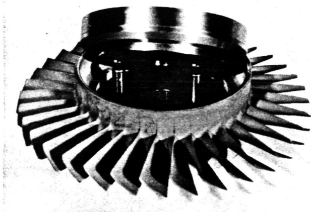
Fig. 5-15. Example of an experimental silicon nitride rotor blade ring
