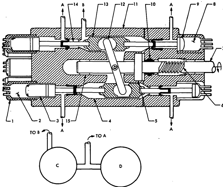
Fig. 6-28. Illustration of a pressurized crankcase Stirling engine, with diaphragm oil barriers and a GMRL hydrodynamic screw seal for the output shaft
