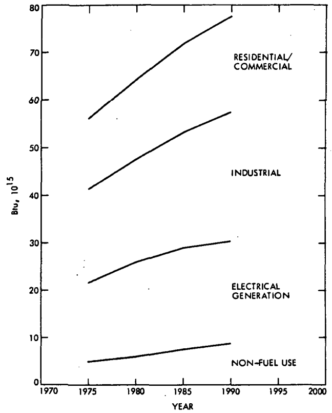
Fig. 17-7. Non-transportation demand for fossil fuel, case C
