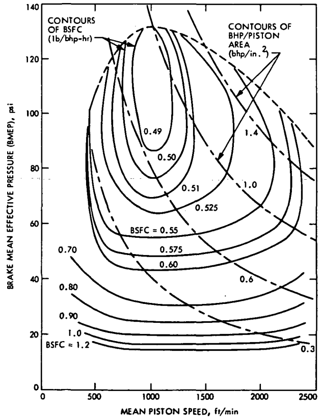
Fig. 3-5. Performance map, typical gasoline engine, 300 in. 3 V-8
