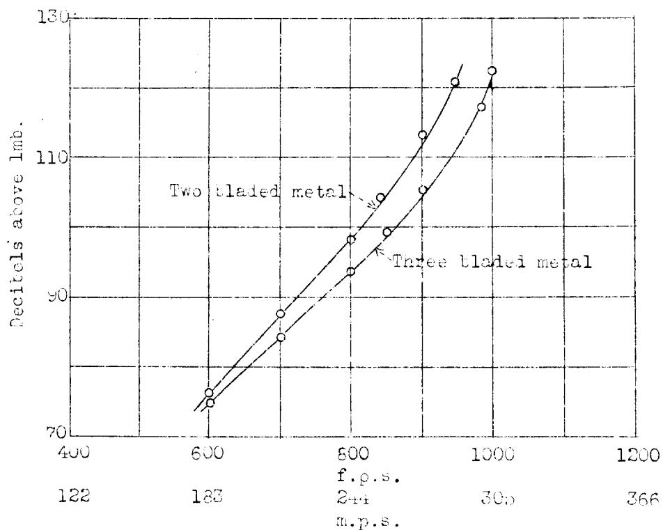
Figure 10.- Noise level (in db above 1 millibar; add 13.8 db to convert to usual reference level) produced by airscrews at various tip speeds.
