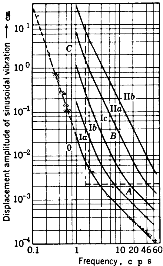
Figure 8.- Response of the individual to vibration (see text).
