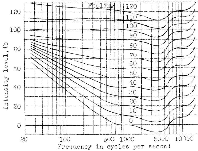
Figure 2.- Loudness level contours of the ear; each contour represents all the tones which are equally as loud as a 1000 cycle per second note. For example, an 80 cycle per second note at 70 decibels sounds as loud as a 1000 cycle note at 50 decibels.
