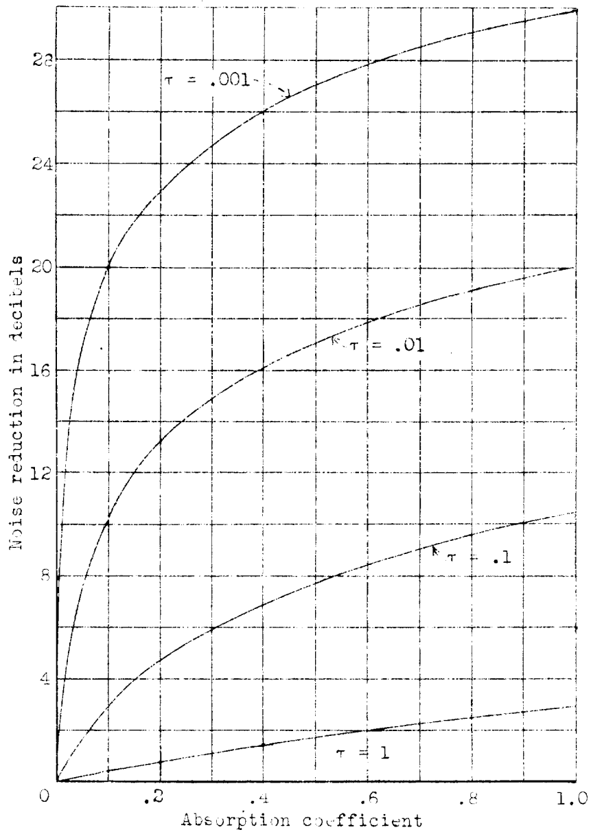
Figure 13.- Variation of noise reduction with absorption coefficient and transmissivity \tau , for an idealized cabin (see text).
