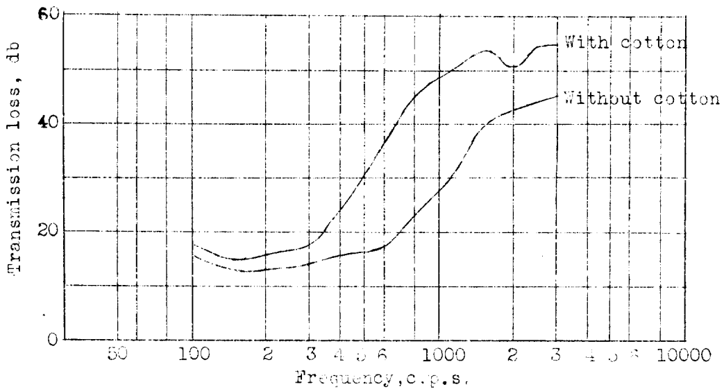
Figure 19.- Transmission loss of a wall consisting of 3 layers of plywood with and without cotton around the borders of the wall.
