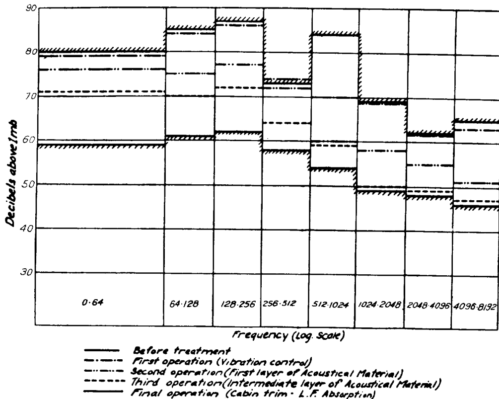
Figure 22.- Progress of noise reduction at various stages of the treatment. Approximately 14 db should be added to noise levels to convert to usual reference level.
