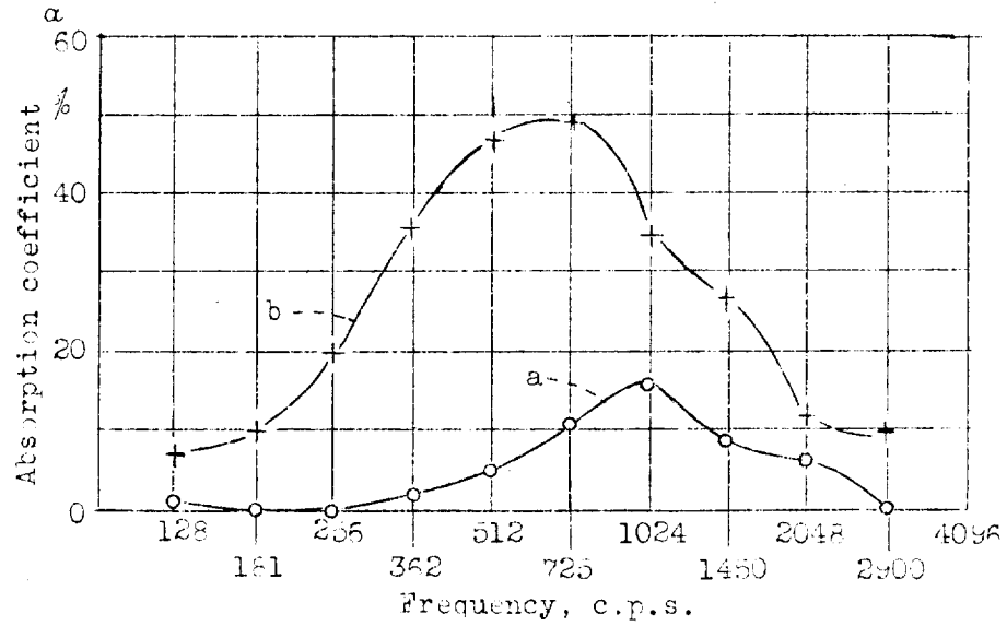
Figure 14.- Sound absorption coefficient of wrapping paper placed 5 cm from wall; a, with airspace only; b, airspace filled with cotton.
