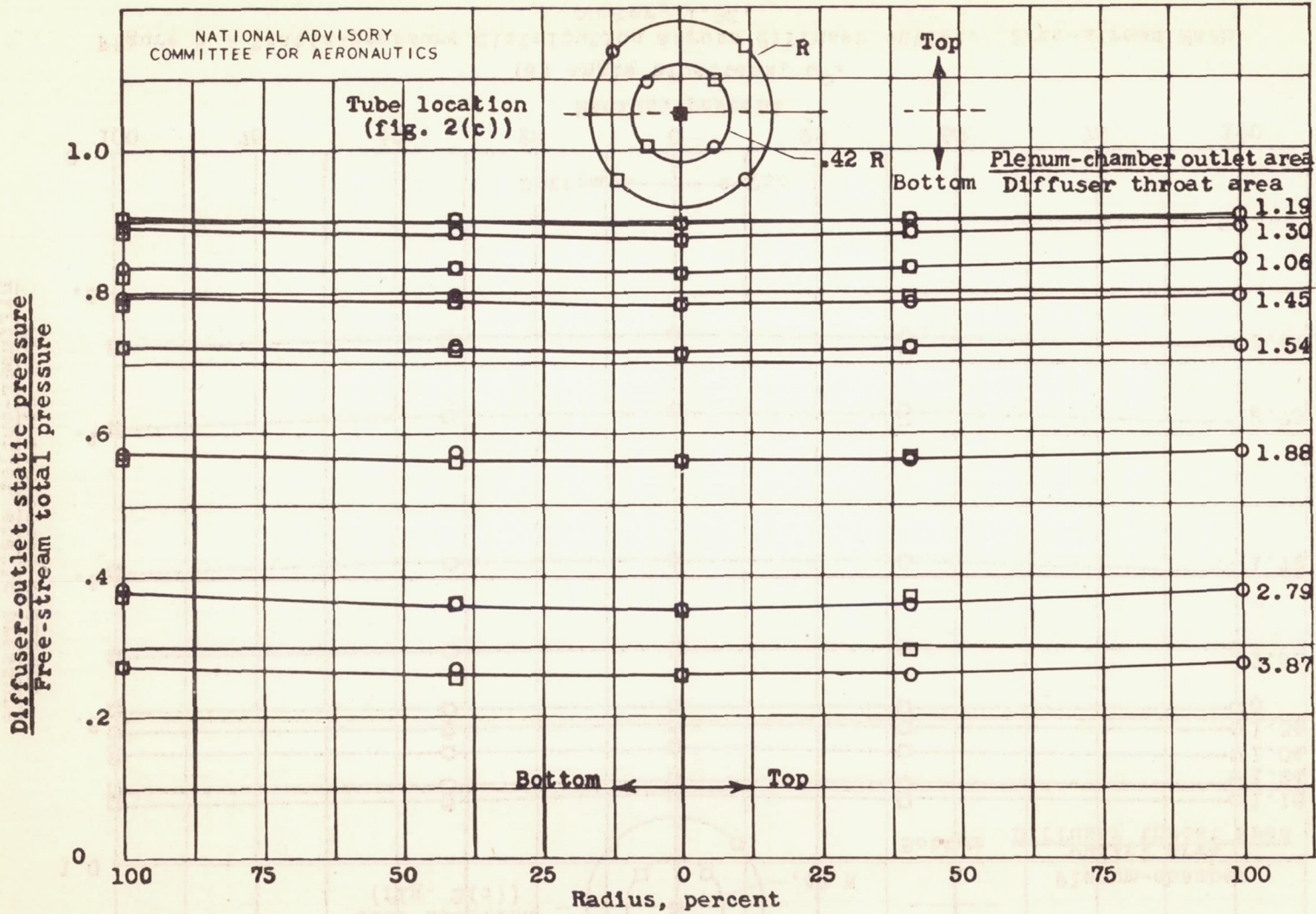
(b) Angle of attack, 3^\circ .
