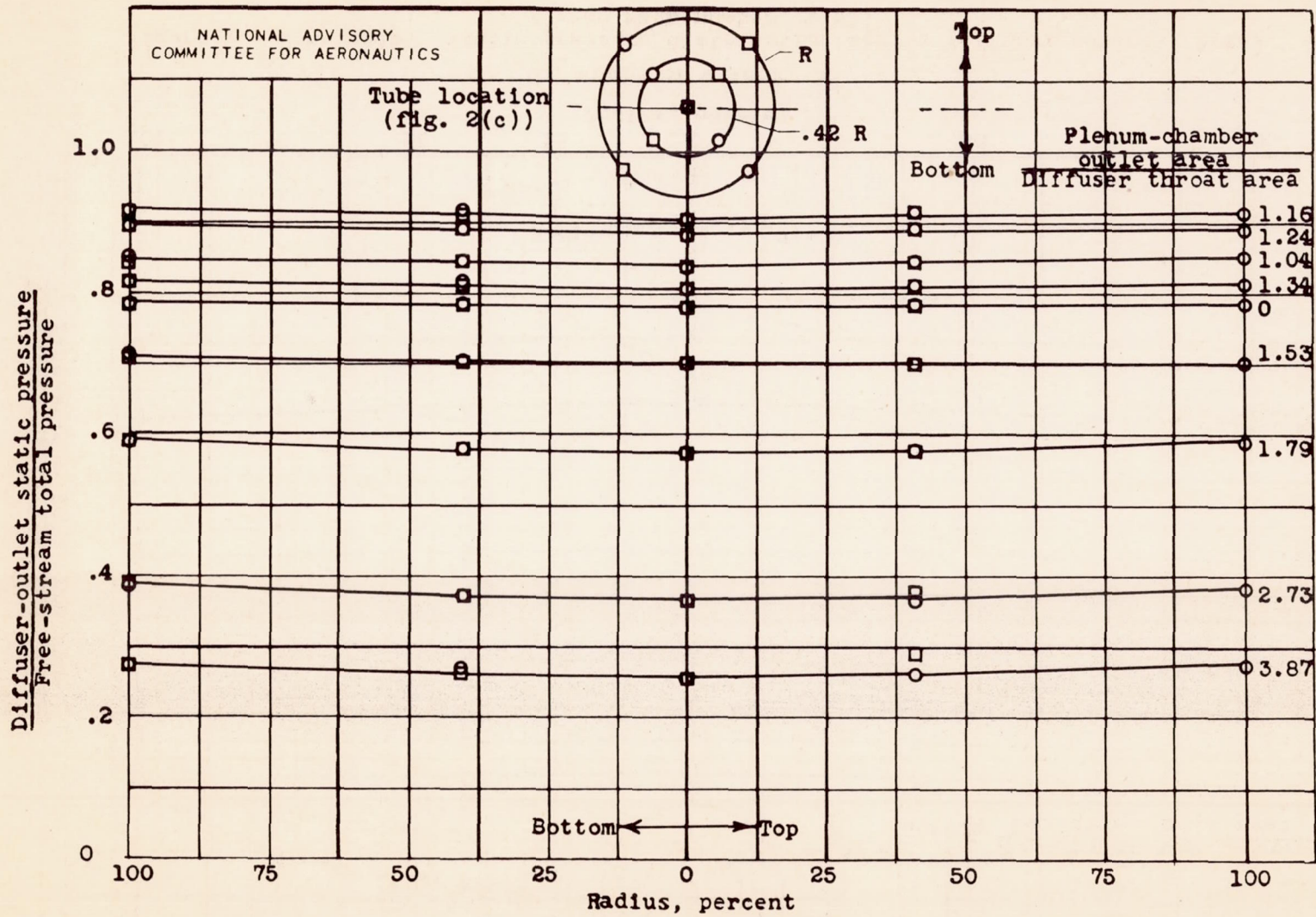
(a) Angle of attack, 0^\circ . Figure 5.- Static-pressure distribution across diffuser outlet. Free-stream Mach number, 1.85.
