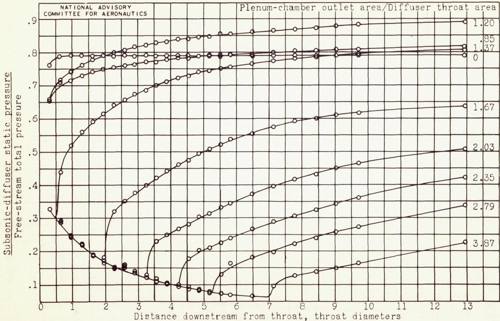
(c) Angle of attack, 5°. Figure 4.- Concluded. Static-pressure distribution along subsonic diffuser. Free stream Mach number, 1.85.
