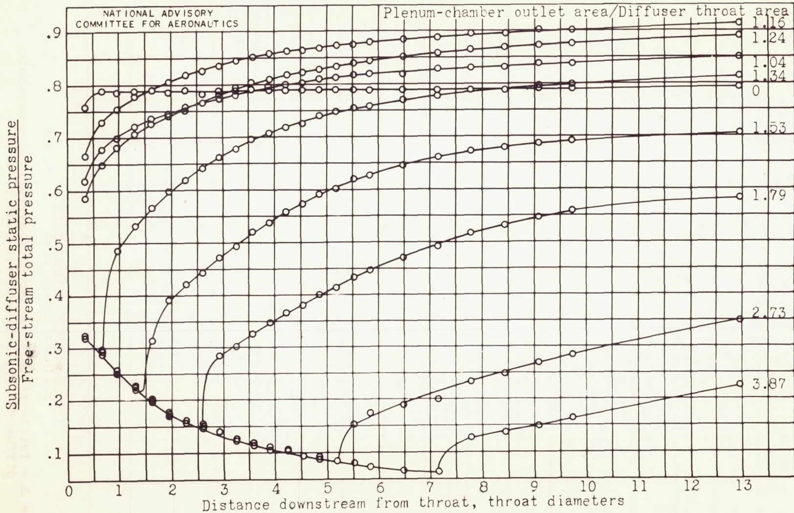
Figure 4.- Static-pressure distribution along subsonic diffuser. Free-stream Mach number, 1.85.
