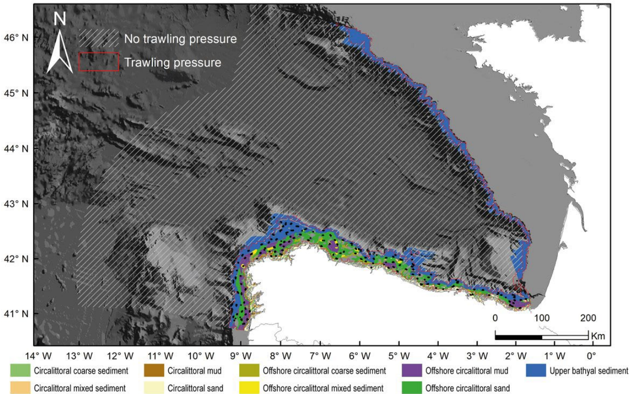
Figure f: The extent and distribution of the nine BBHTs assessed and the location of the hauls used in the North-Iberian Atlantic assessment unit. The grey-hatched area corresponds to areas where there was no trawling effort
