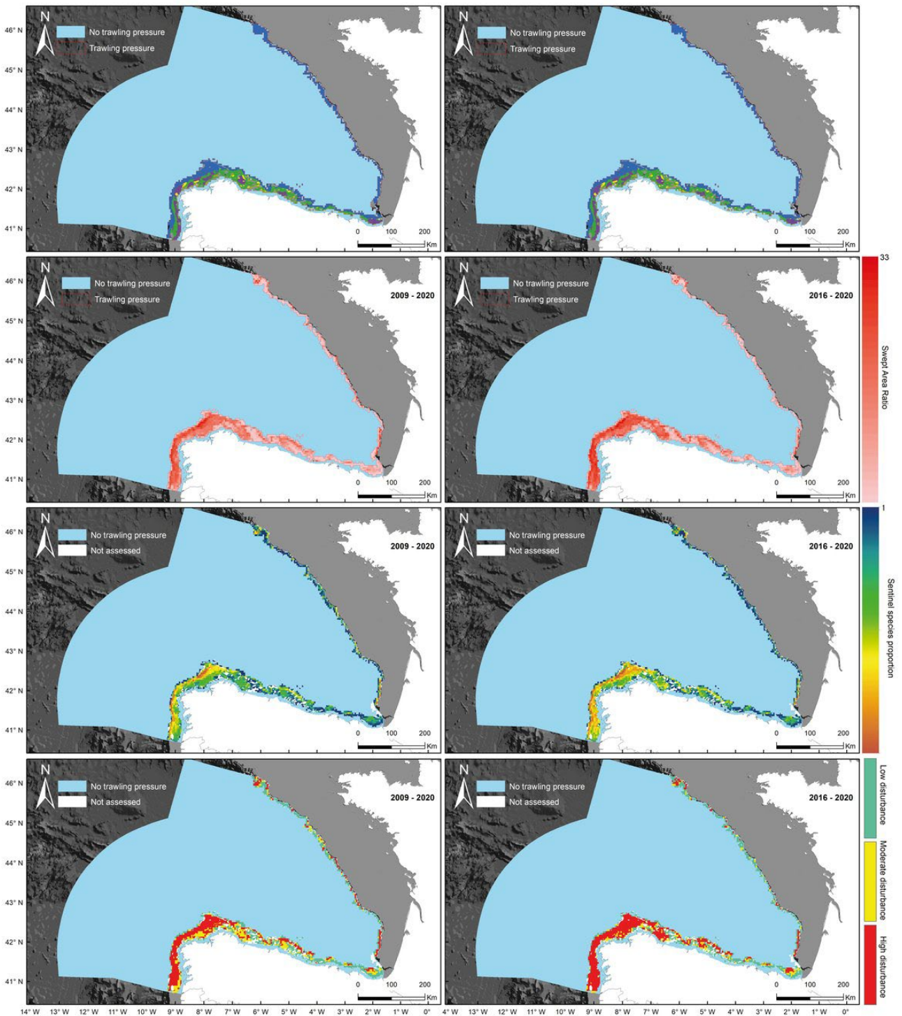
Figure ak: North Iberian Atlantic Summary figure of the BH1 QSR 2023 assessment. From top to bottom: MSFD habitats assessed; Mean swept area ratio (SAR); Predicted sentinel species proportion based on the pressure-states curves; Final assessment status. From left to right: From 2009 to 2020; from 2016 to 2020
