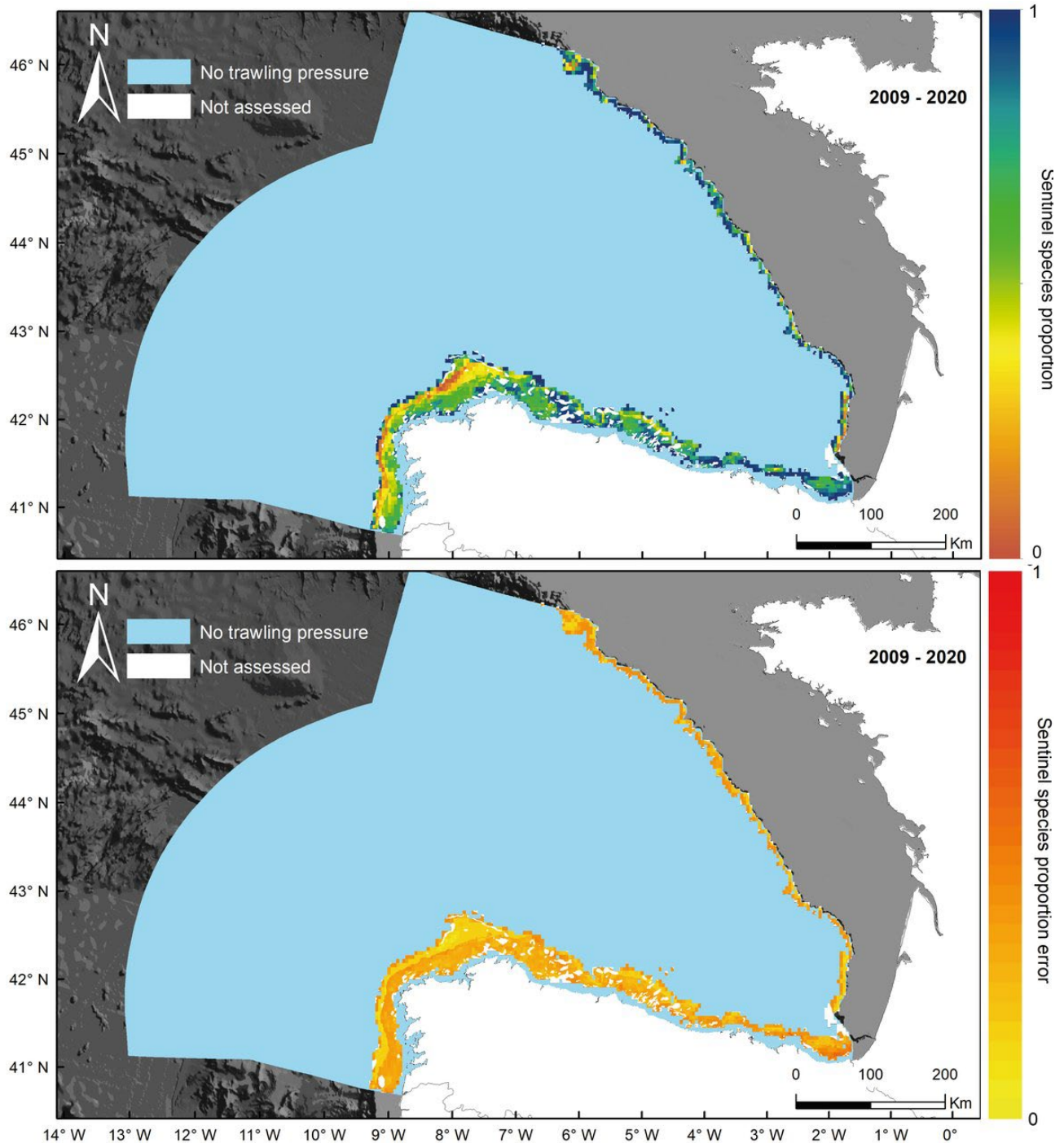
Figure t6: North Iberian Atlantic. Overall Common Indicator Assessment area. Top: Prediction of sentinel species based on the mean SAR value from 2009 to 2020. Bottom: Standard error associated with the prediction of sentinel species proportion from 2009 to 2020
