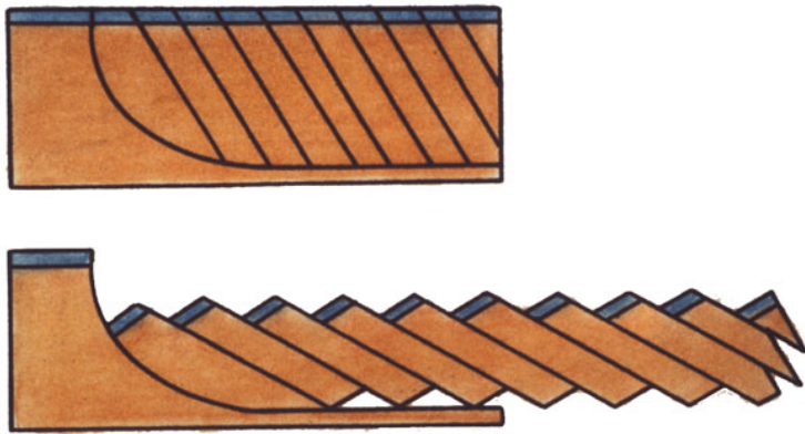
Figure 4: Listric fault, with rotating upper plate blocks and breakaway fault
