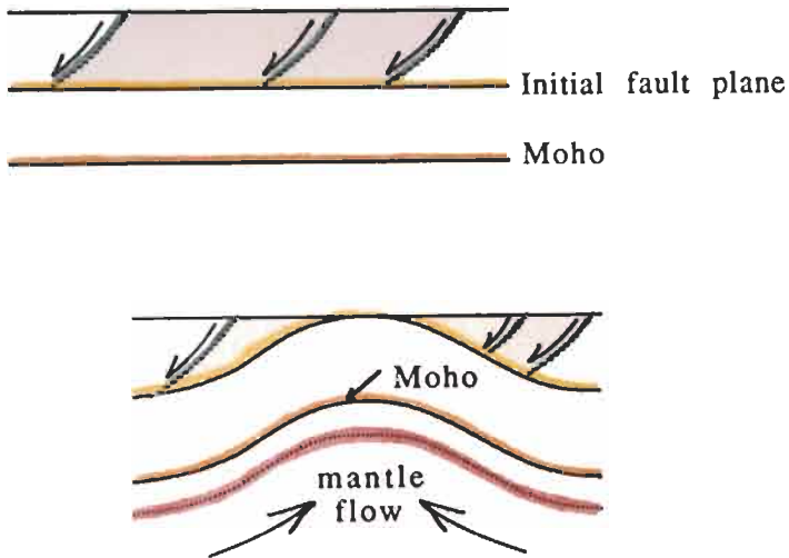
Figure 7: Two models for accommodating large amounts of extension in the upper crust. From Block and Royden 1984
