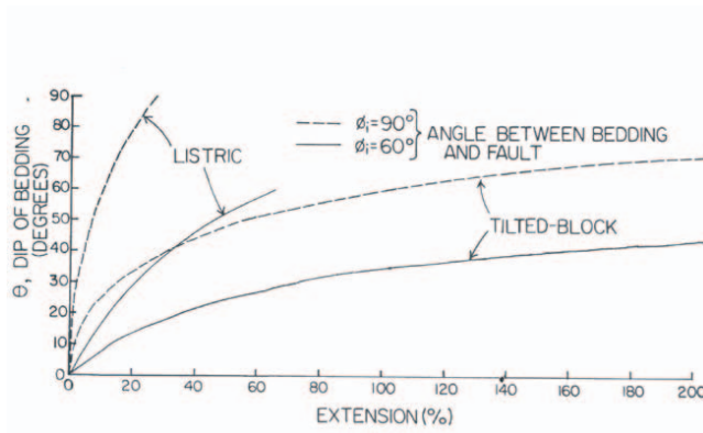
Figure 3: A system of rotating, planar faults. The bottom figure shows how this geometry compares to simple listric normal faults in terms of the amount of extension that can be produced
