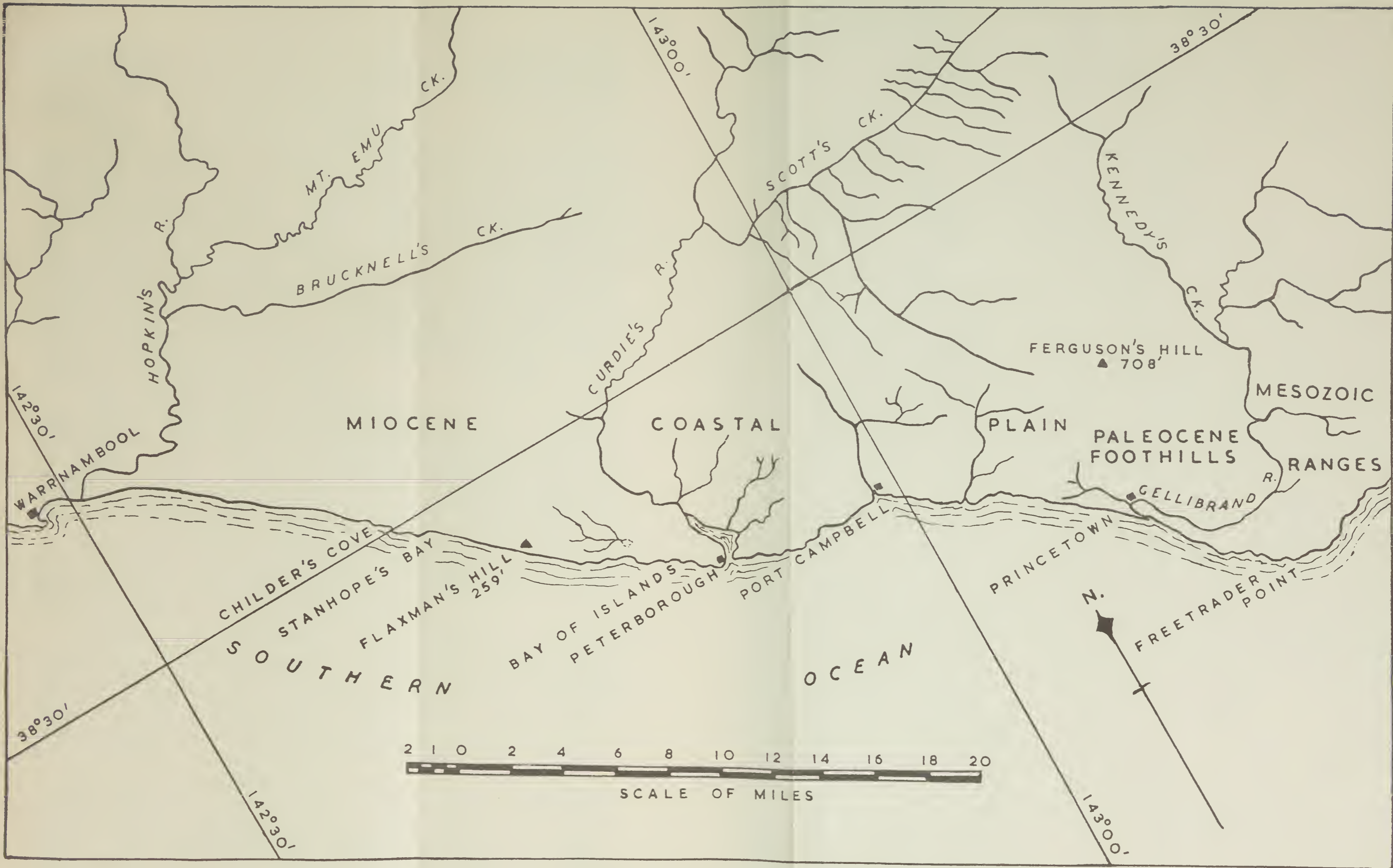
FIGURE 1.—Locality map of the coastal region between Freertrader Point and Warrnambool, South-western Victoria.
