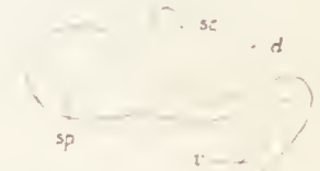
Text fig. 9. Austroboris peculiaris (Abraham). Detail of the position of the vesiculae seminales in relation to the vagina and uterine duct.
