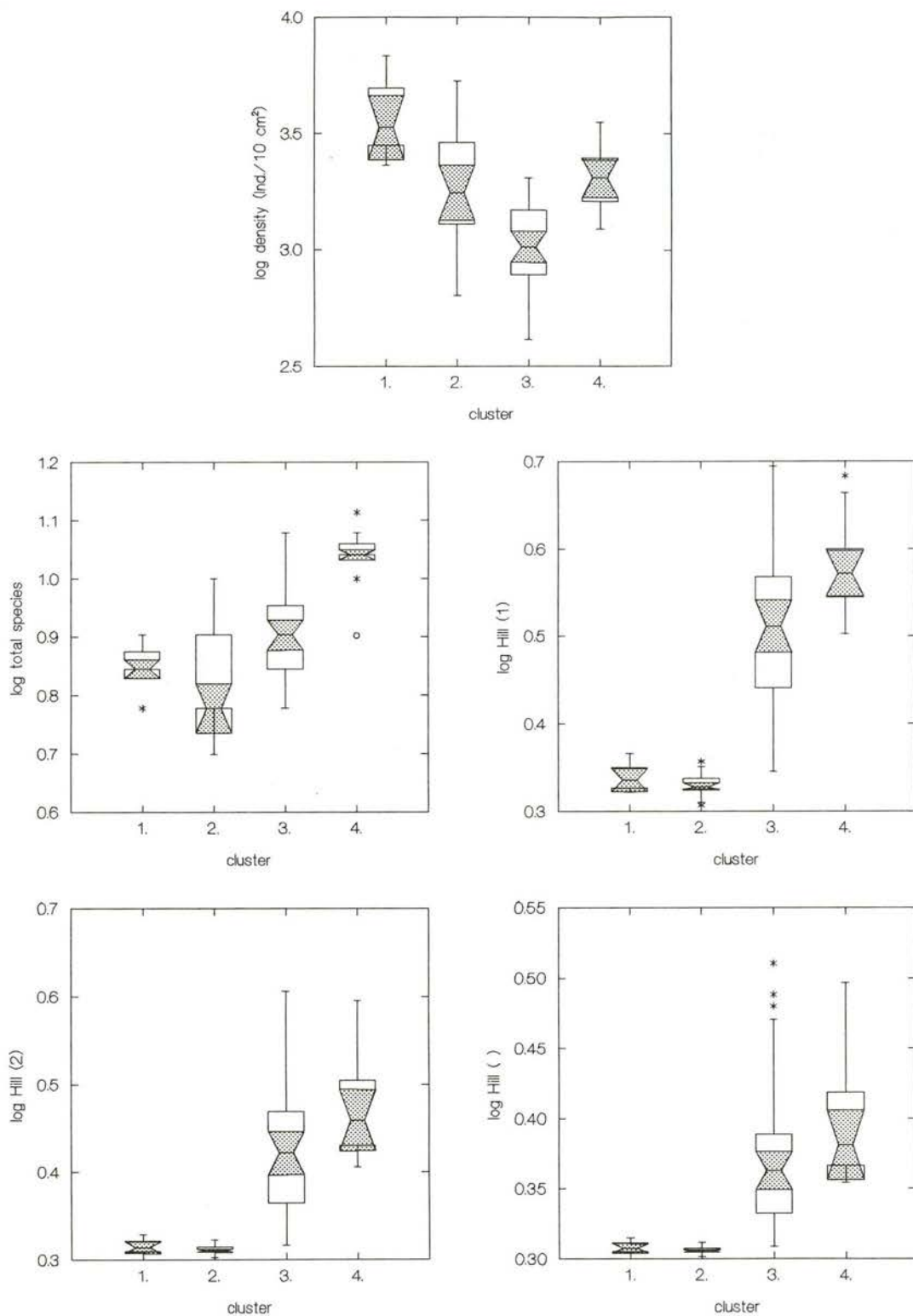
Fig. 31b. Box and whisker plots of some average meiobenthic parameters ( \log(x+1) -transformed) after TWIN-SPAN analysis using the data of the meiobenthos density (ind./10 cm 2 ) (cf. Figs. 28, 29 and Table 6).
