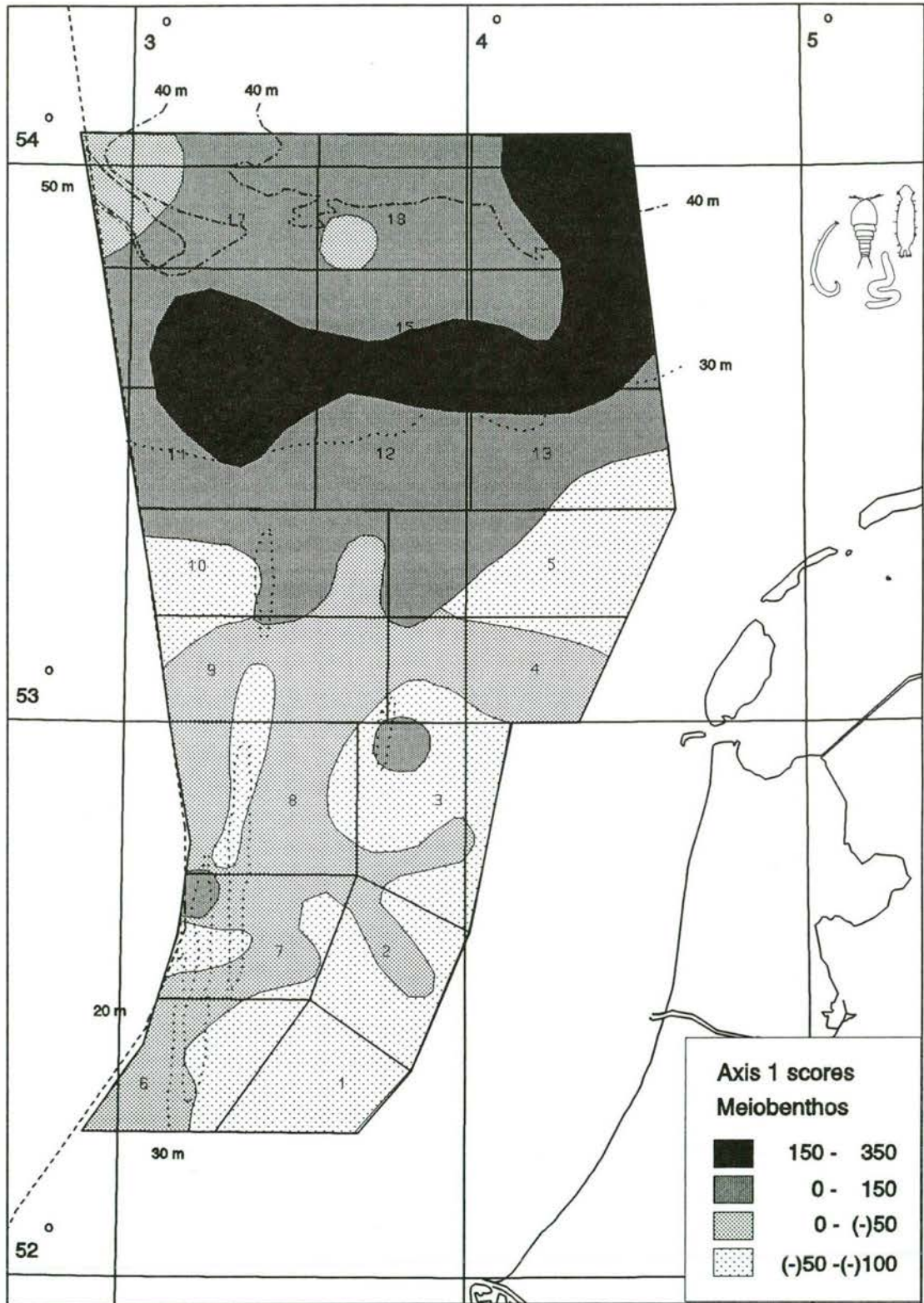
Fig. 86. Axis 1 contours of the meiobenthos.
