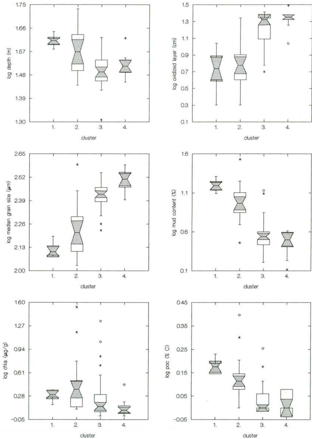
Fig. 31a. Box and whisker plots of the average abiotic parameters (log(x+1)-transformed) after TWINSPLAN analysis using the data of the meiobenthos density (ind./10 cm 2 ) (cf. Figs. 28, 29 and Table 6).
