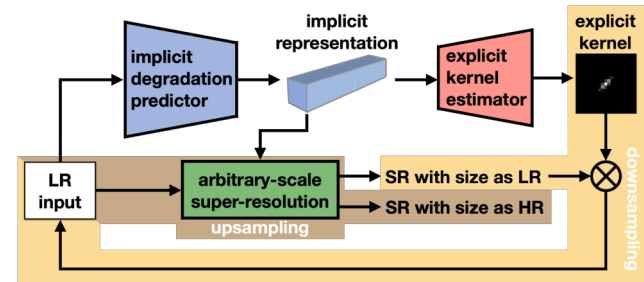
Figure 1. Conceptual illustration of our proposed method for tackling arbitrary-scale blind super-resolution problem, with highlighting our two main designs: 1) utilizing both implicit degradation representation and explicit degradation kernel, and 2) integrating both upsampling and downsampling processes (shaded by light brown color and light yellow color respectively) into a holistic framework for enabling the training objective of cycle-consistency.
