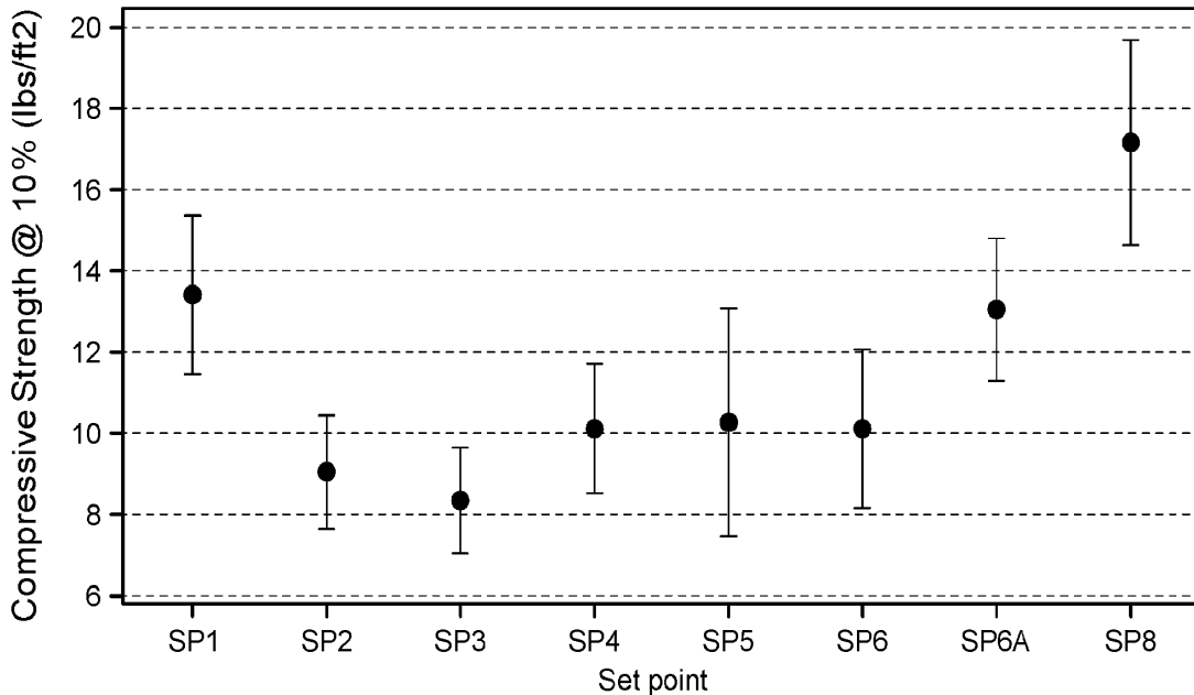
Interval Plot of Compressive Strength @ 10% (lbs/ft 2 ) 95% CI for the Mean
