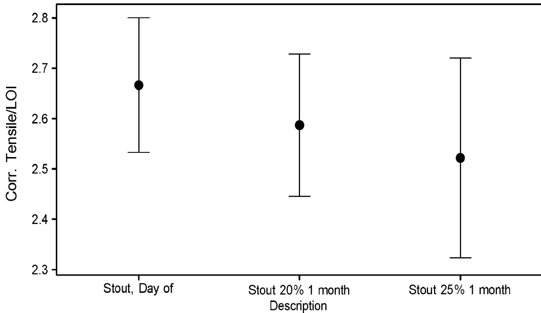
Interval Plot of Corr. Tensile/LOI 95% CI for the Mean
