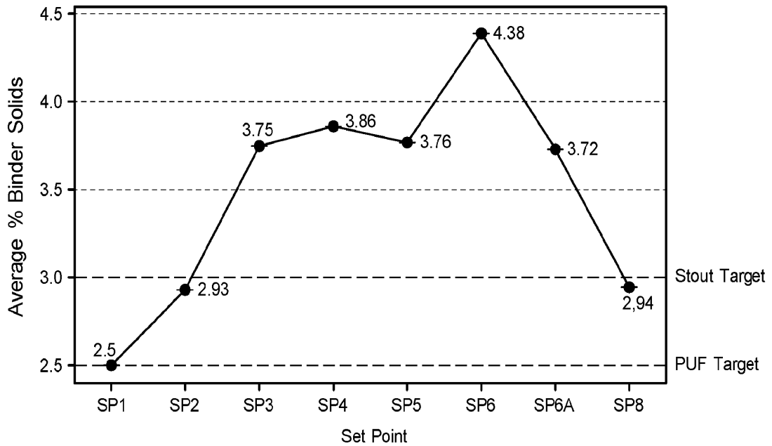
Interval Plot of Average % Binder Solids 95% CI for the Mean
