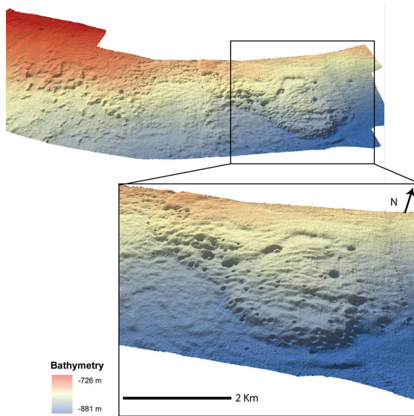
Fig. 3. Perspective view of the shaded relief DTM (resolution 5 m and 10 × vertical exaggeration) of the study area showing the distribution of the pockmarks and their geometries; the inset shows a magnification of the highest density pockmarks area with more than 40 pockmarks with variable dimensions (8 of the major ones and up to 30 minor features).
