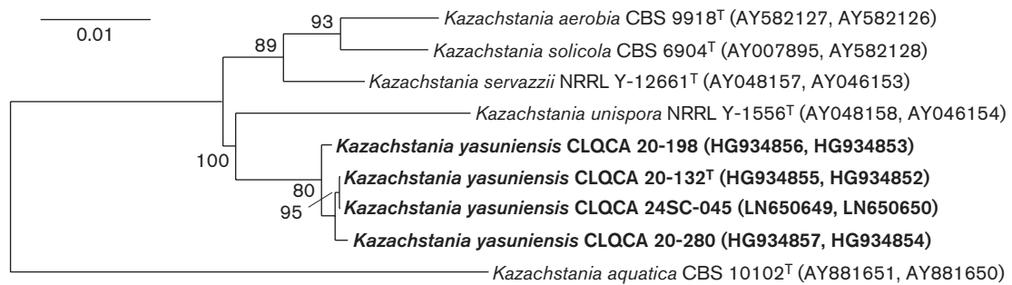
Fig. 1. Neighbour-joining dendrogram based on the combined sequences of the LSU D1/D2 and ITS regions (including 5.8S rDNA) of Kazachstania yasuniensis sp. nov. and its closest relatives. Species names are followed by CBS, CLQCA or NRRL strain accession numbers and, respectively, the EMBL/GenBank accession numbers for the LSU D1/D2 and ITS regions. Kazachstania aquatica was used as the outgroup species for the analysis. Bootstrap values of \geq 50\% , determined from 1000 replicates, are shown at branch nodes. Bar, 1 base substitution per 100 nt.
