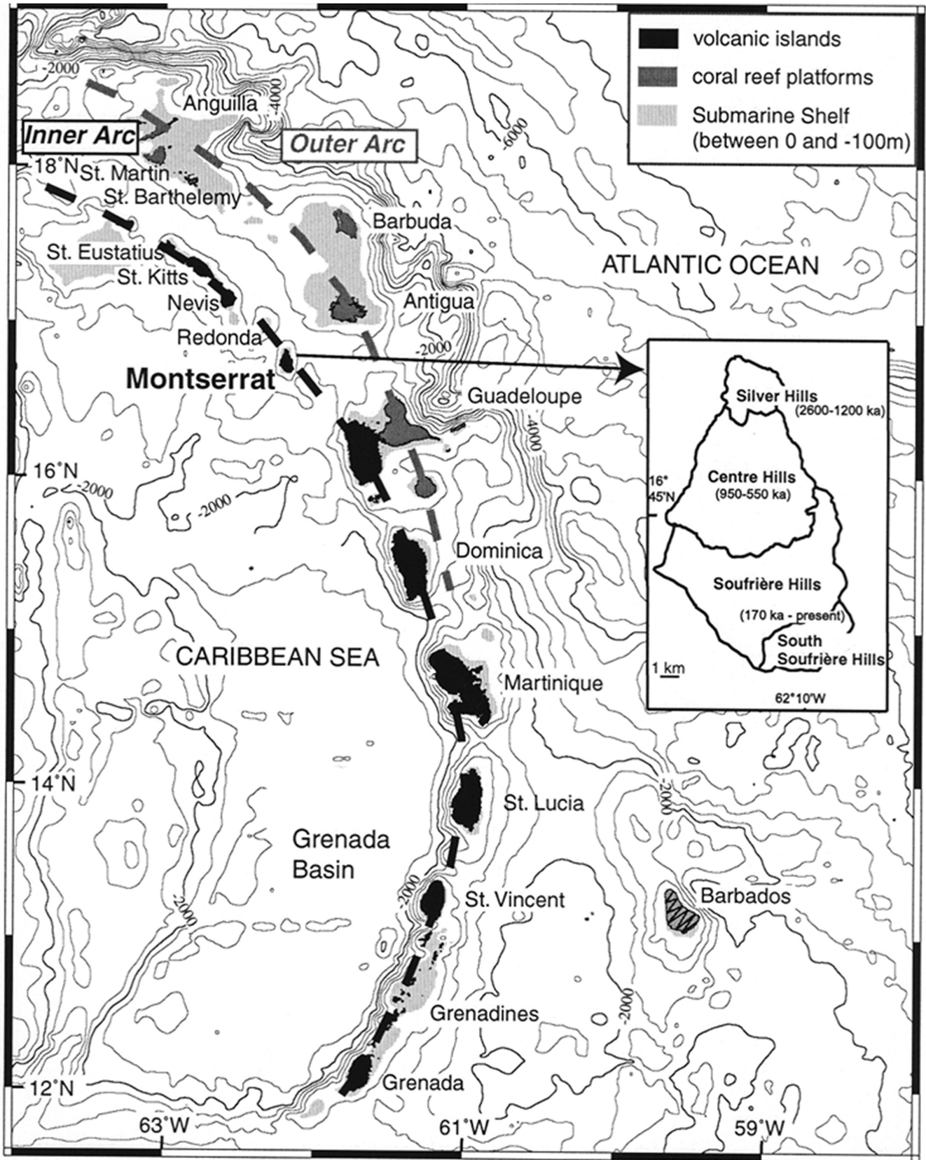
TEXT-FIGURE 1 Location of Montserrat within the Lesser Antilles Volcanic Arc. Inset map shows the main volcanic areas of Montserrat and their relative ages; after Le Friant et al. (2008).
