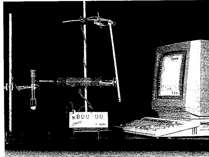
10. Dialometer for measuring the change in volume of a gas as its temperature varies.
