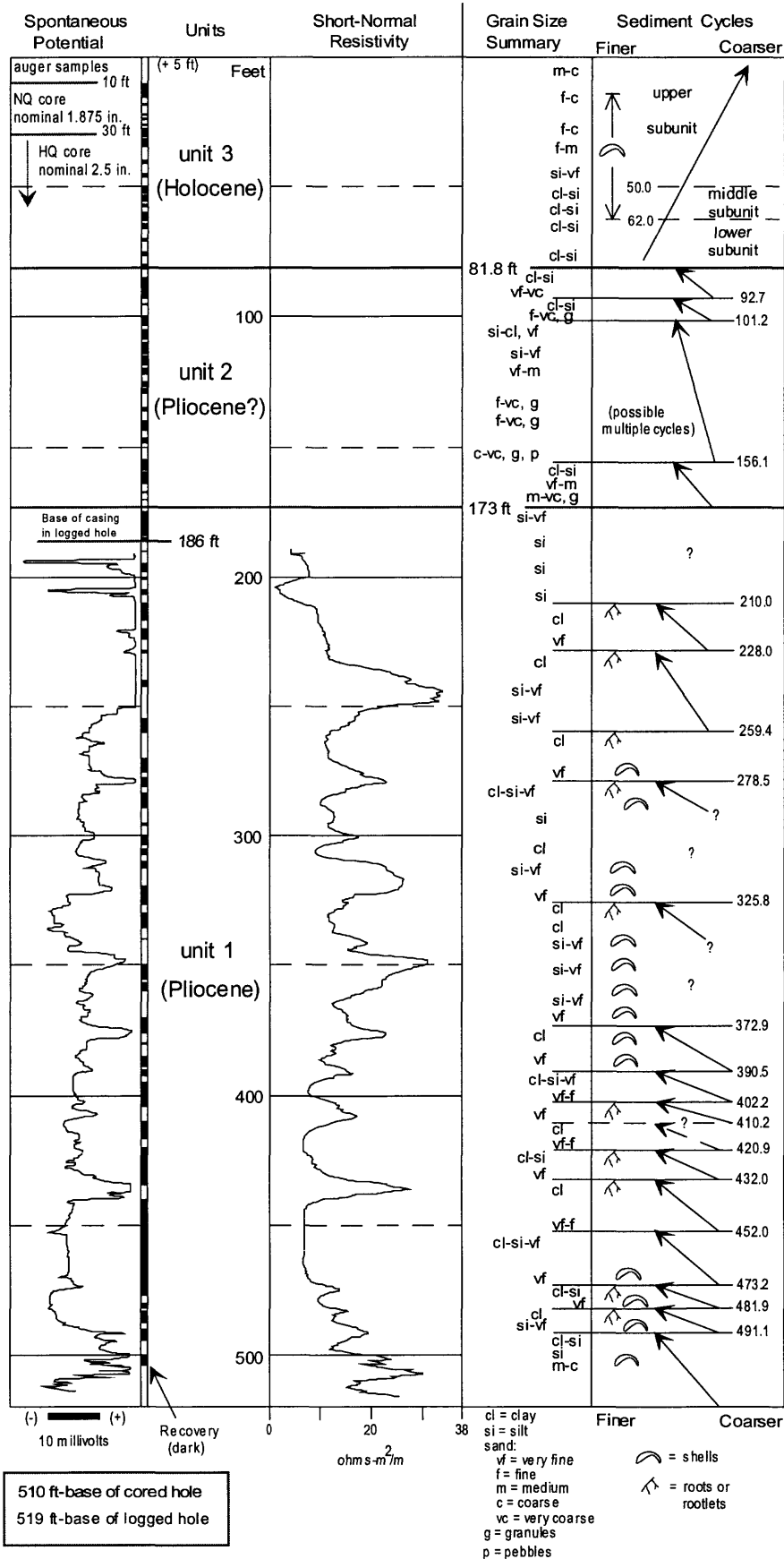
Figure 2. Electric log and lithologic data for the USGS Horn Island core.
