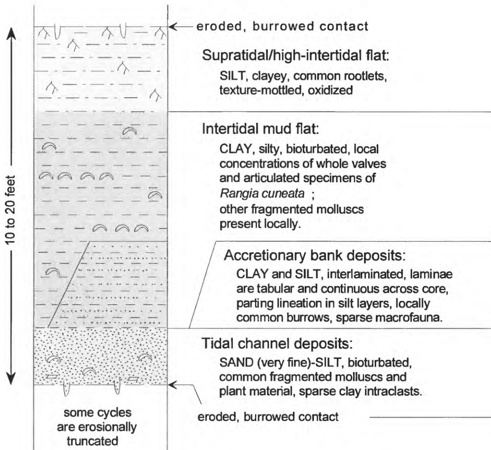
Figure 3. Generalized sediment cycle found in the estuarine deposits of unit 1 (modeled on figure 20 of Clifton, 1982). Accretionary bank deposits are rare in the upper two-thirds of unit 1.
