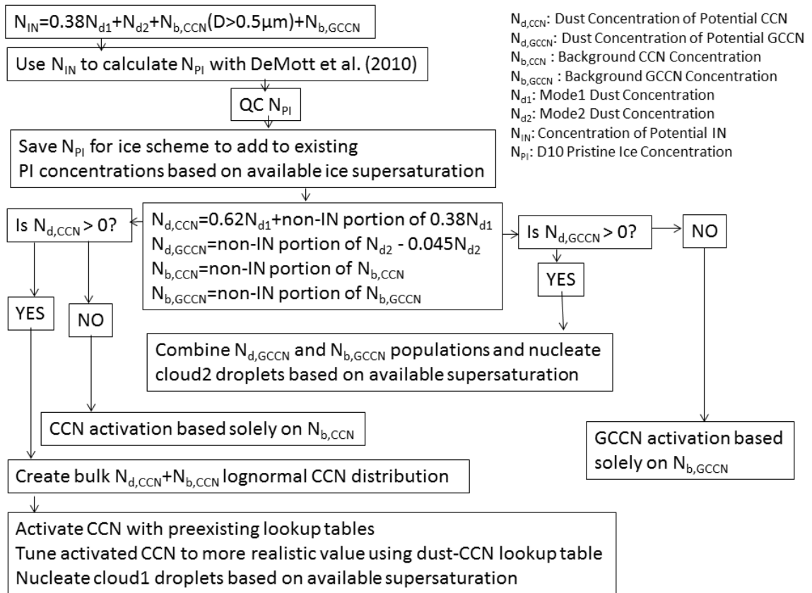
Figure 3.14: Flowchart outlining the dust microphysics scheme implemented in RAMS.
