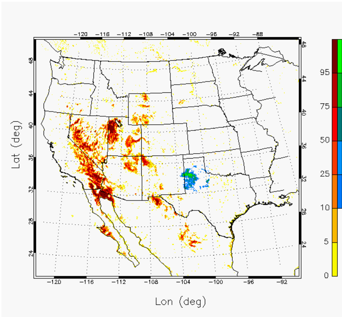
Figure 3.6: MODIS-based fractions (percentages) of barren land, or desert, category (yellow-orange-red colorbar) and croplands within the Texas panhandle (blue-green colorbar). Fractions are given in units of percent.
