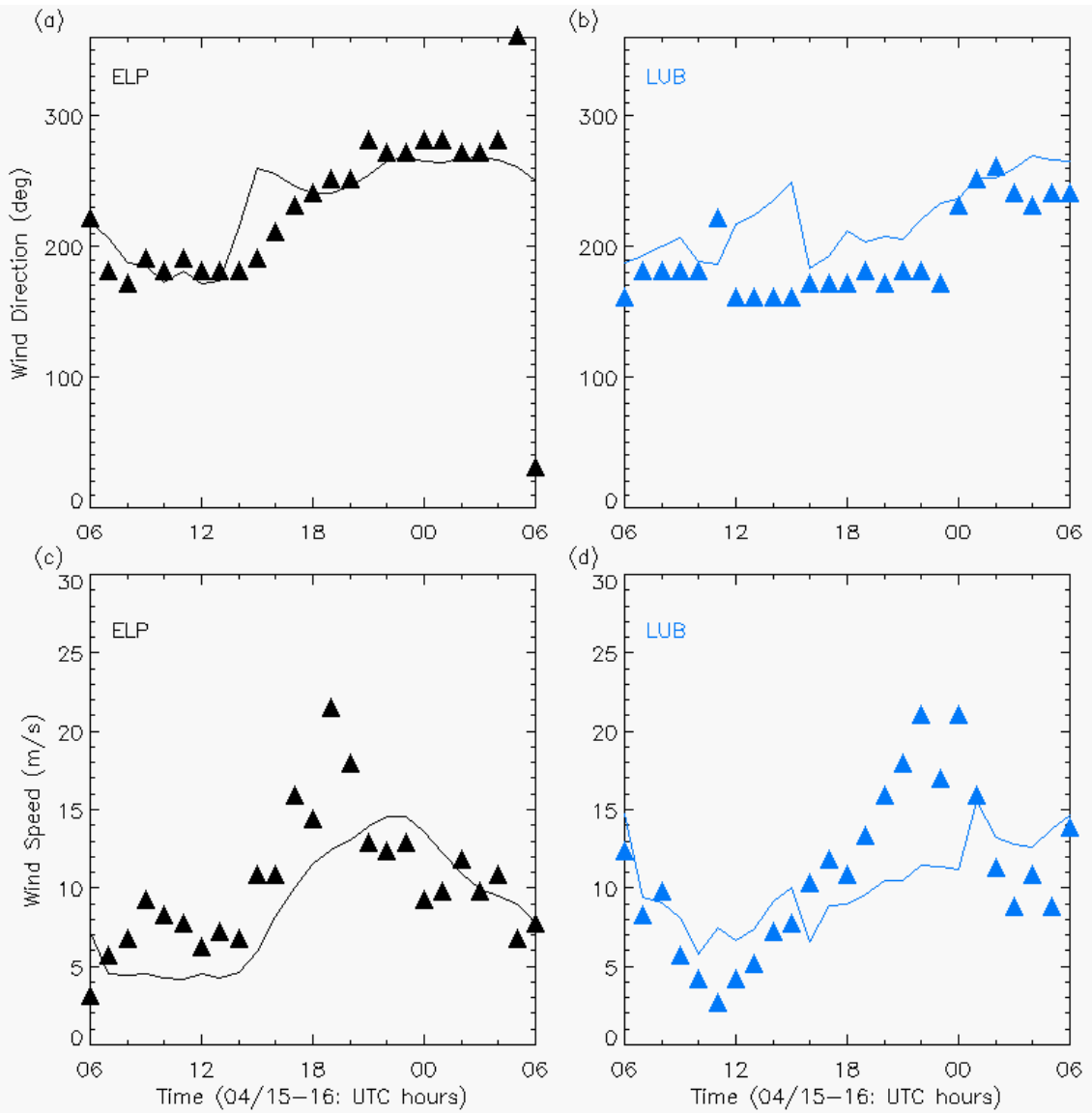
Figure 7.6: Time series of simulated near-surface winds on Grid 2 from the DST experiment (solid curves) and associated hourly METAR reported winds (filled triangles); (a) El Paso (ELP) wind direction, (b) Lubbock (LUB) wind direction, (c) El Paso wind speed, and (d) Lubbock wind speed.
