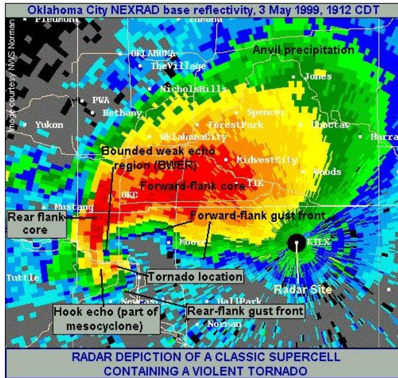
Figure 2.5: NEXRAD radar depiction of a classical type supercell that contains a violent F-5 tornado from Oklahoma City, OK on 3 May 1999 at 1912 CDT ( http://www.spc.noaa.gov/faq/tornado/radscl.htm ).
