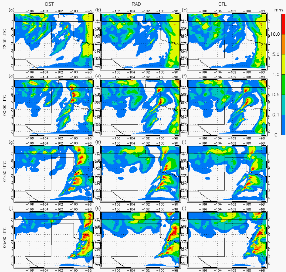
Figure 7.8: Grid 2 VIC for the DST (column 1), RAD (column 2), and CTL (column 3) simulations at 2230 UTC on 15 April (row 1) and 16 April at 0000 (row 2), 0130 (row 3), and 0300 UTC (row 4).
