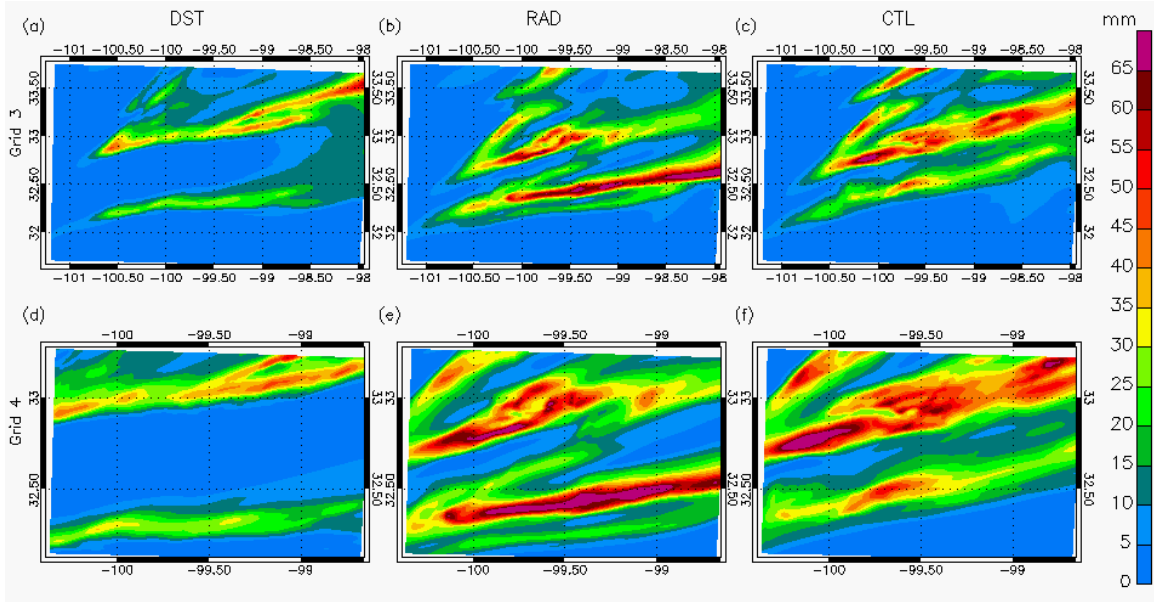
Figure 7.14: Accumulated precipitation on Grid 3 (row 1) and Grid 4 (row 2) at 5 UTC on 16 April from the DST (column 1), RAD (column 2), and CTL (column 3) simulations.
