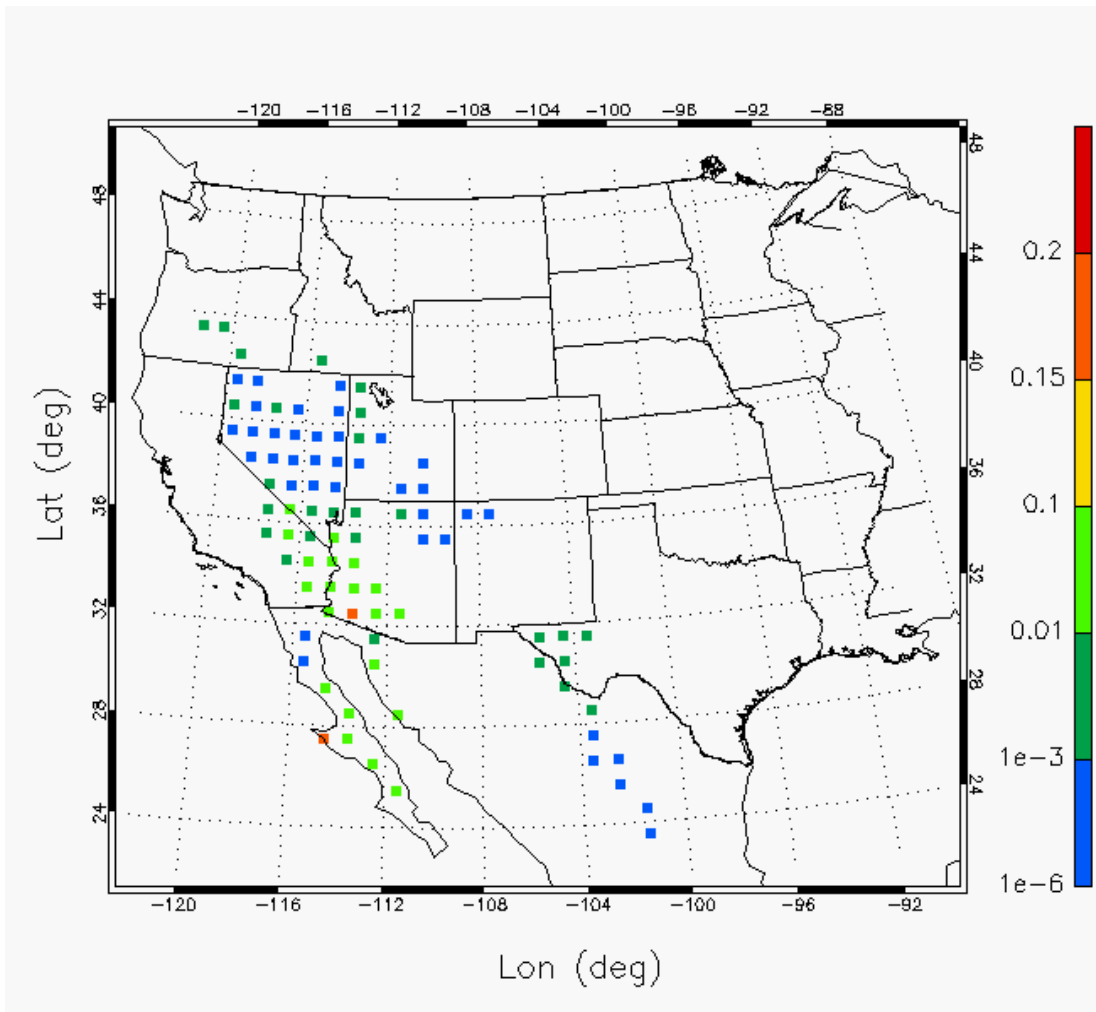
Figure 3.1: The Ginoux et al. (2001) dust source function, S , over the western U.S. and Mexico. The colorbar denotes nondimensional values of S .
