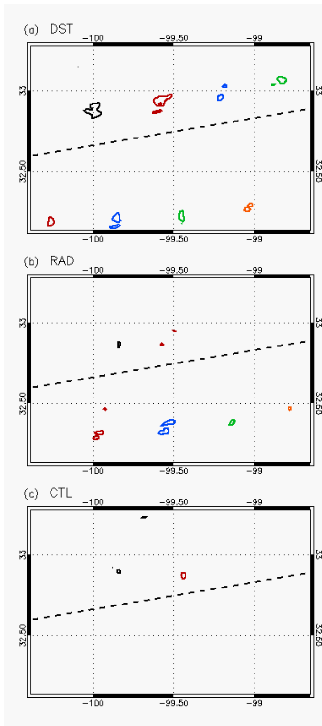
Figure 7.10: Evolution of vertical relative vorticity on Grid 4 in the (a) DST, (b) RAD, and (c) CTL simulations. Smoothed maximum vertical relative vorticity between 2 and 6 km is contoured at 0130 (black), 0200 (red), 0230 (blue), 0300 (green), and 0330 (orange) UTC for each simulation at 0.025 and 0.05 \text{ s}^{-1} . The dashed line delineates the northern storm track of the grid (NR1) from the southern storm track region (SR2).
