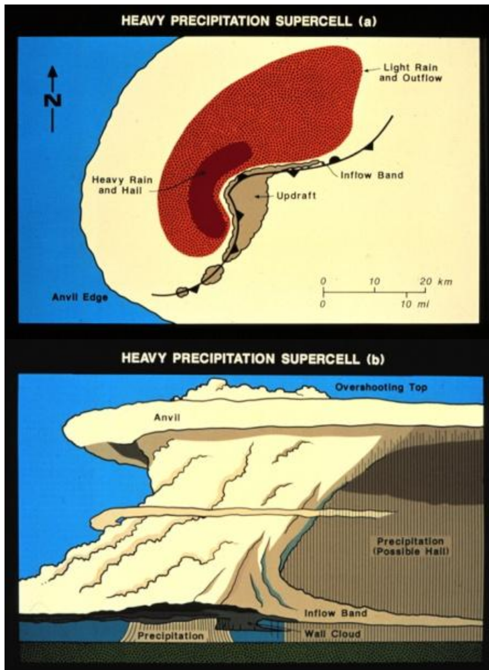
Figure 2.7: A conceptual model of a high-precipitation supercell, showing (a) the low-level precipitation structure and cloud features looking down from above and (b) visual structures from an observer's point of view to the east of the storm (from Doswell and Burgess 1993).
