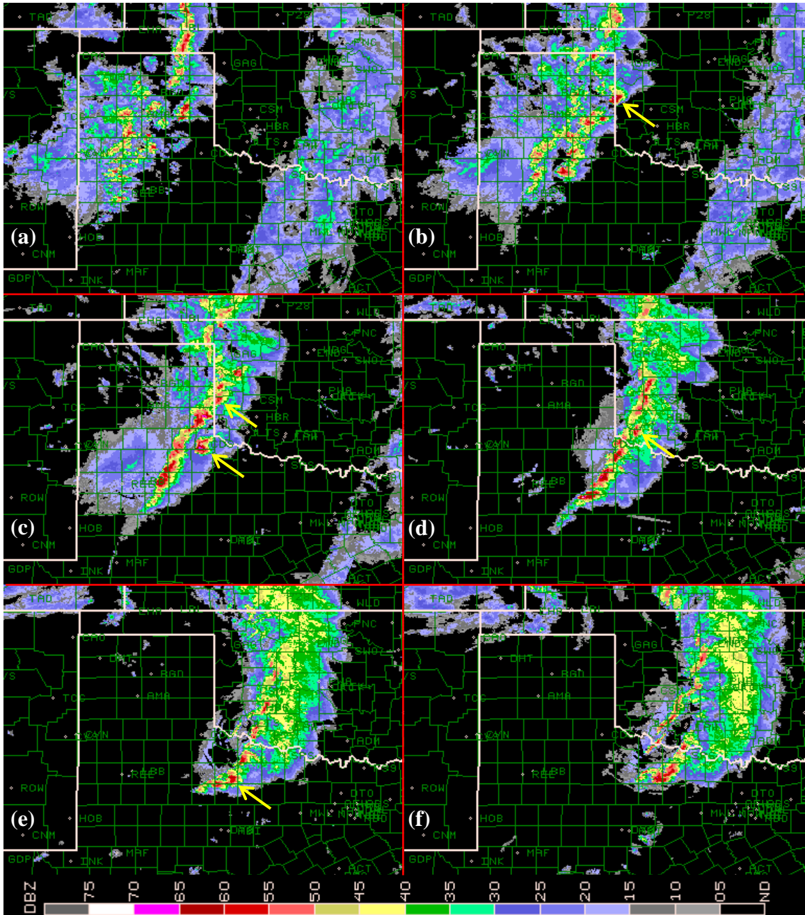
Figure 6.9: WSR-88D radar images of composite reflectivity over eastern New Mexico, northern Texas, and Oklahoma at (a) 22 and (b) 23 UTC on 15 April 2003 and (c) 00, (d) 01, (e) 02, and (f) 03 UTC on 16 April 2003. Yellow arrows point to individual supercells that are tornadic near the time of the image.
