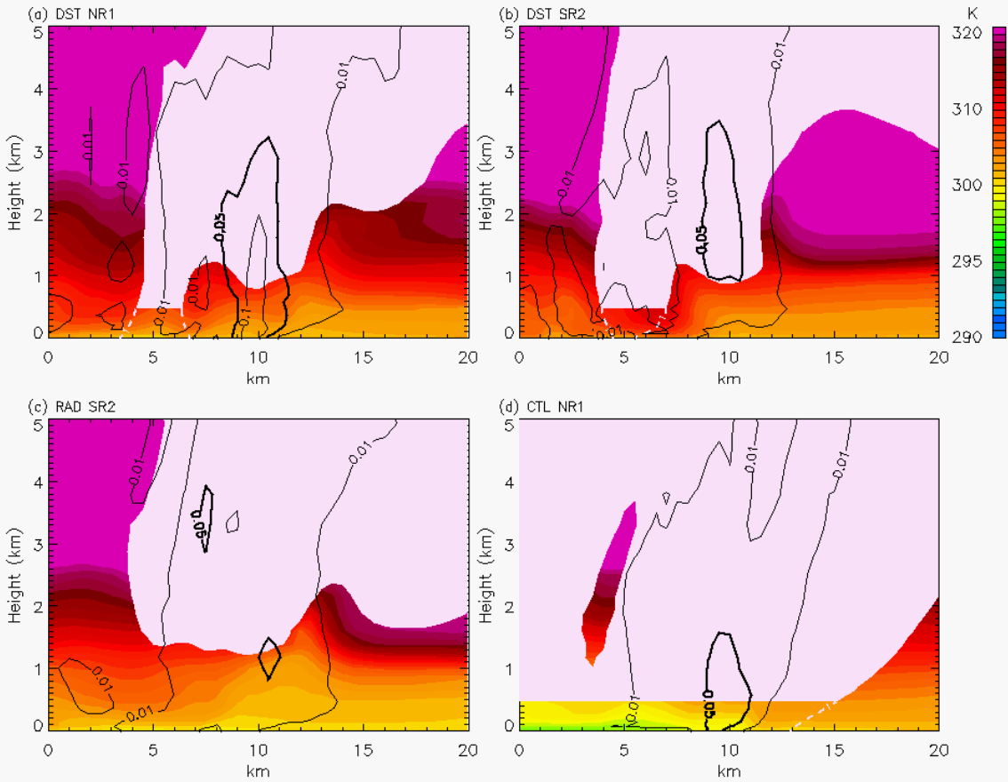
Figure 7.28: Vertical cross-sections of mean potential temperature overlaid with mean total condensate greater than 1 \text{ g kg}^{-1} (filled pink contoured above 477 m; dashed pink contour lines below 477 m) and maximum relative vertical vorticity contoured at 0.01, 0.05 (thick), and 0.1 \text{ s}^{-1} on Grid 4 for the (a) DST NR1 supercell at 0200 UTC, (b) DST SR2 supercell at 0220 UTC, (c) RAD SR2 supercell at 0230 UTC, and (d) CTL NR1 supercell at 0150 UTC. The domains are centered over the location of maximum relative vertical vorticity below 6 km (same as Fig. 7.27). Maximum values of vorticity and mean values of total condensate and \theta are based on the latitude of maximum vorticity (below 6 km) \pm 2.5 \text{ km} in the latitudinal direction.
