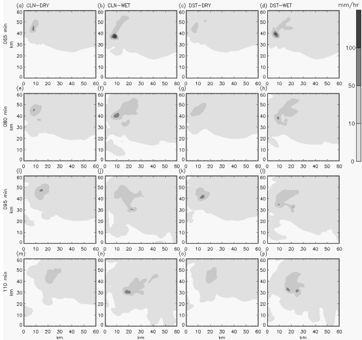
Figure 5.5: Same as Fig. 5.2 but for precipitation rates on Grid 2.
