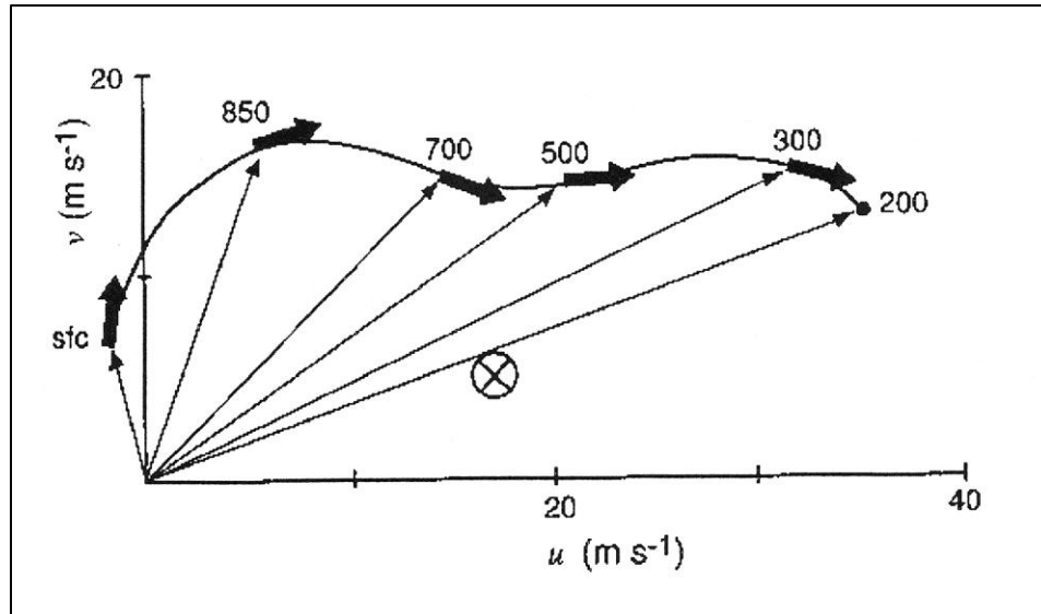
Figure 2.1: Mean hodograph for 62 tornado outbreak cases. The soundings are composited by computing the winds at each level relative to the estimated storm motion. Heavy arrows indicate the direction of the shear vector at each level (labeled in mb). The estimated storm motion is denoted by the encircled 'X' (from Maddox 1976).
