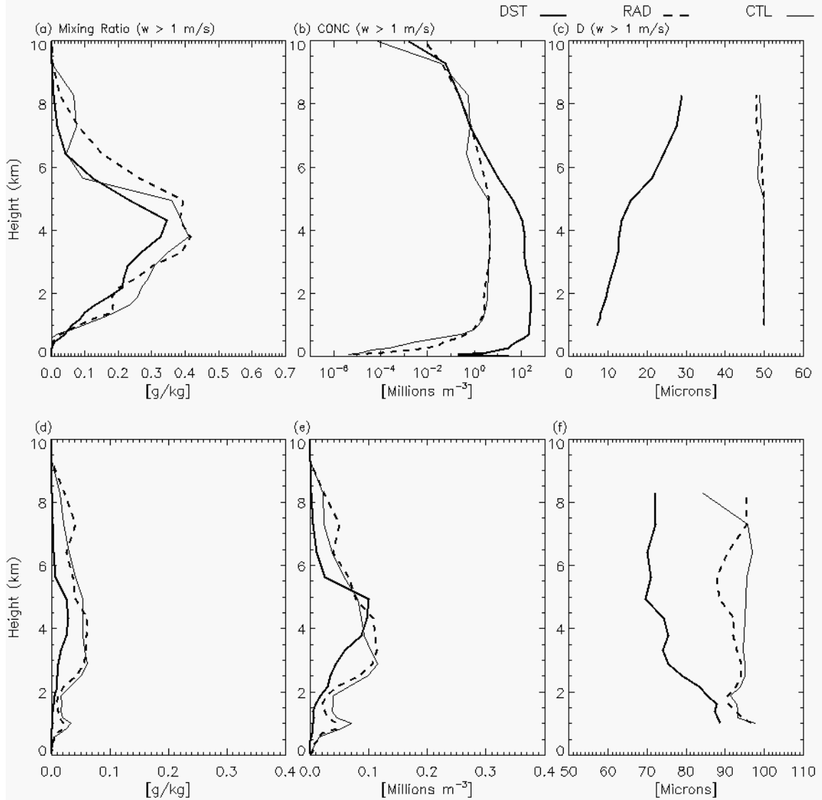
Figure 7.19: Mean profiles of cloud1 (row 1) and cloud2 (row 2) droplet mixing ratio (column 1), number concentration (column 2), and median diameter (column 3) within updrafts greater than 1 \text{ m s}^{-1} on Grid 4 within the NR1 region for the DST (thick solid), RAD (thick dashed), and CTL (thin solid) simulations at 0200 UTC. Values are based on the location of maximum vertical relative vorticity and the surrounding 25 \times 25 \text{ km} region.
