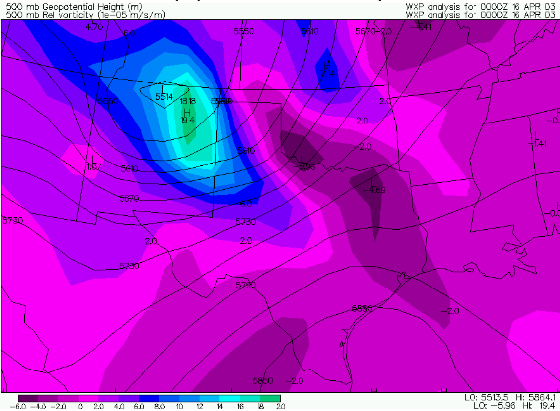
Figure 6.4: Vertical relative vorticity at 500 mb on 16 April 2003 at 0 UTC from Plymouth State University online archives. 500-mb geopotential height contours (m) are overlaid ( http://vortex.plymouth.edu ).
