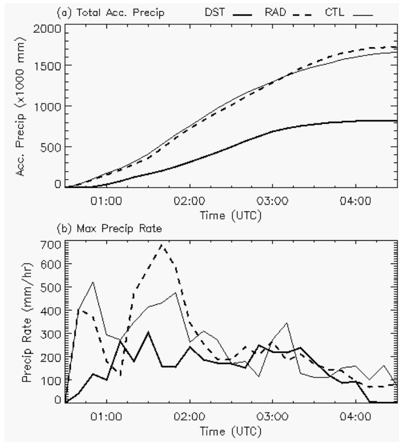
Figure 7.16: Time series of (a) grid-cumulative accumulated precipitation and (b) maximum precipitation rates on Grid 4 for the DST (thick solid), RAD (thick dashed), and CTL (thin solid) simulations.
