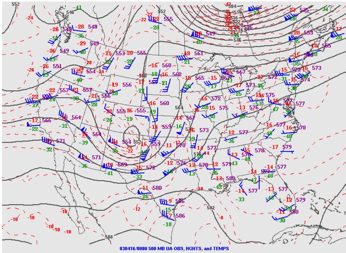
Figure 6.3: 500-mb analyses from SPC for 16 April 2003 at 0 UTC. Isoheights are overlaid in black, and isotherms are plotted with red dashed curves. Wind barbs (kt) are overlaid in blue. Temperature, dew point temperature, and 500-mb heights are plotted at various sounding stations in red, green, and purple, respectively.
