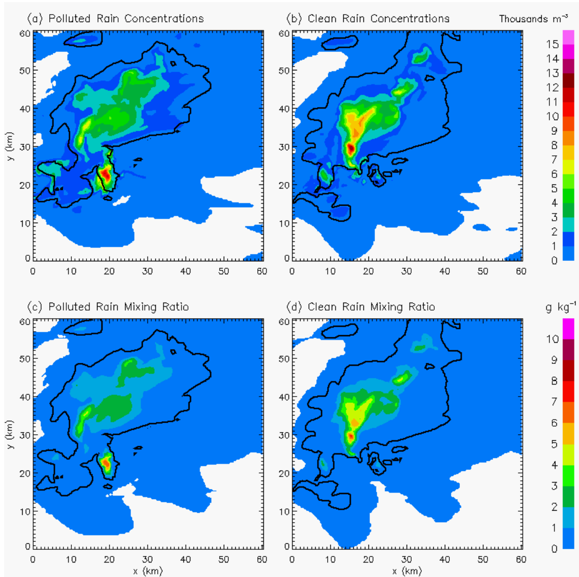
Figure 4.7: Rain concentrations at 1 km for the POL (a) and CLN (b) simulations (top panels) and rain mixing ratios at 1 km for the POL (c) and CLN (d) simulations (bottom panels) at 90 minutes on Grid 2. Plots are overlaid with 30-dBZ model reflectivity boundaries at 1 km for reference.
