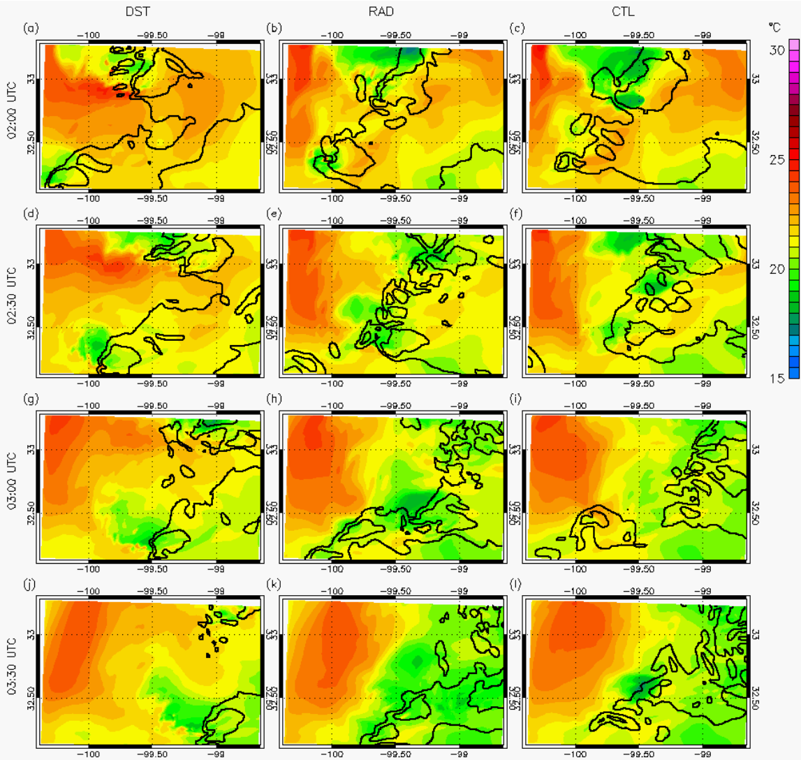
Figure 7.18: Near-surface temperature on Grid 4 for the DST (column 1), RAD (column 2), and CTL (column 3) simulations at 0200 (row 1), 0230 (row 2), 0300 (row 3), and 0330 (row 4) UTC on 16 April. Panels are overlaid with VIC at 0.5 and 5 mm.
