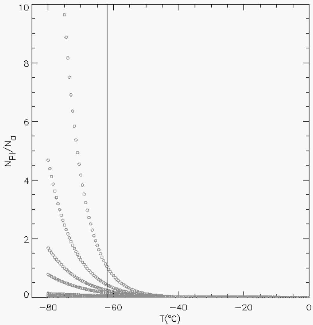
Figure 3.15: IN activation fractions as a function of temperature according to the DeMott et al. (2010) activation scheme. Gray open circles denote individual data points at increments of 0.5^{\circ}\text{C} for initial aerosol concentrations of 0.005, 0.01, 0.05, 0.1, 0.5, 1.0, 5.0, 10.0, 25.0, and 100\text{ cm}^{-3} . The line representing a temperature of -62^{\circ}\text{C} is also plotted.
