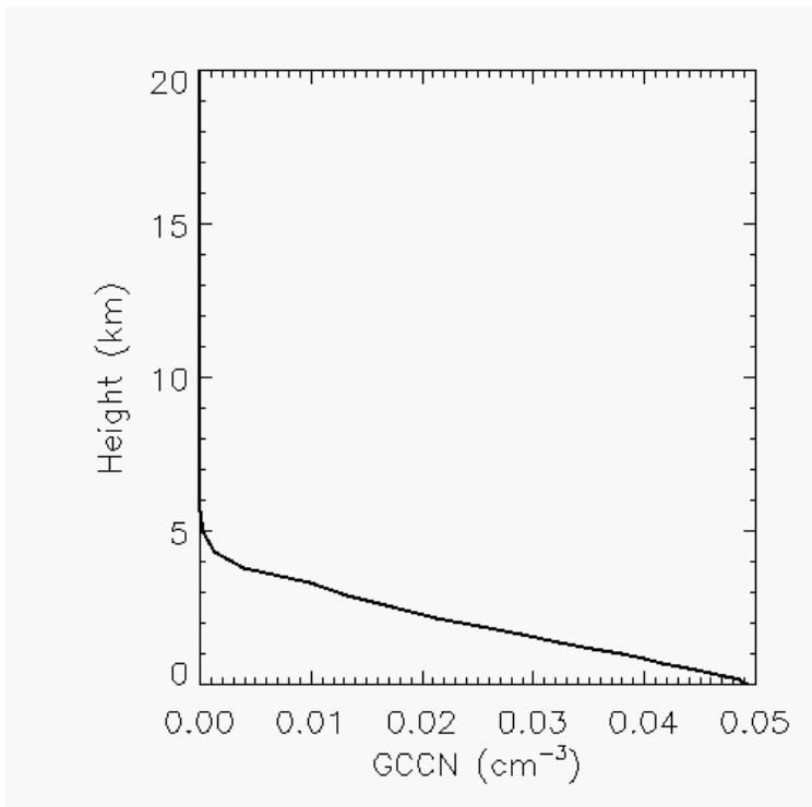
Figure 7.3: Initial profile of GCCN number concentrations for the 15-16 April 2003 case simulations.
