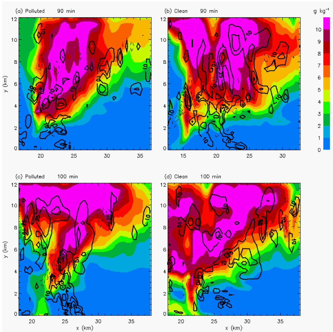
Figure 4.9: Constant ‘y’ vertical cross-sections of total mixing ratio overlaid with vertical vorticity ( -25, -10, 10, 25, 50 \times 10^{-3} \text{ s}^{-1} ) at 90 (top) and 100 minutes (bottom) on Grid 2 through the main updraft for the POL (left) and CLN (right) simulations. Cross-section regions are denoted in Figs. 4.2 and 4.3 as lines ‘AB’.
