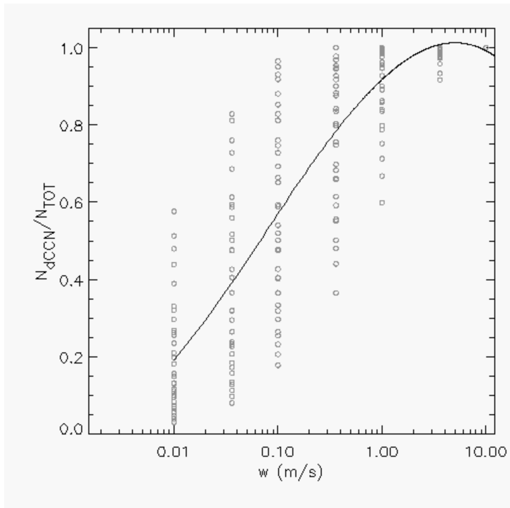
Figure 3.12: Dust GCCN activation fractions plotted as a function of vertical velocity for each parcel simulation. The black curve represents the 3 rd order polynomial best-fit curve to the dataset.
