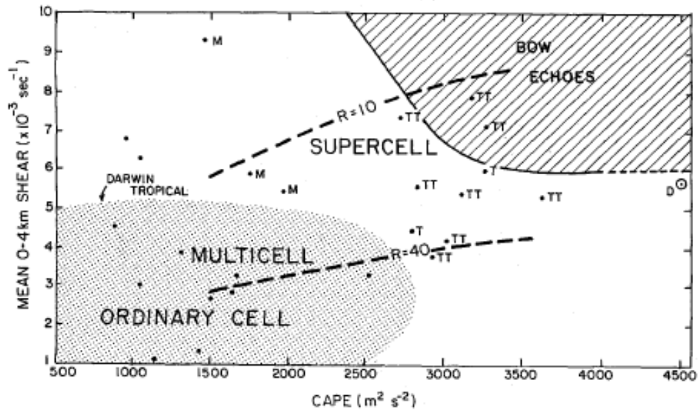
Figure 2.2: Types of convective elements as a function of mean vertical wind shear in the lowest 4 km and CAPE (from Rasmussen and Wilhelmson 1983). 'M' represents a storm with a mesocyclone but no tornado, 'T' a storm with one tornado, 'TT' a storm with more than one tornado, and an unmarked dot denotes a storm without a mesocyclone. 'D' represents mean conditions for derechos. The heavy dashed lines indicate bulk Richardson number values of 10 and 40. The shaded region indicates the approximate range of conditions found near Darwin, Australia, during the active and break monsoon periods. The hatched region indicates the range of conditions for bow echoes.
