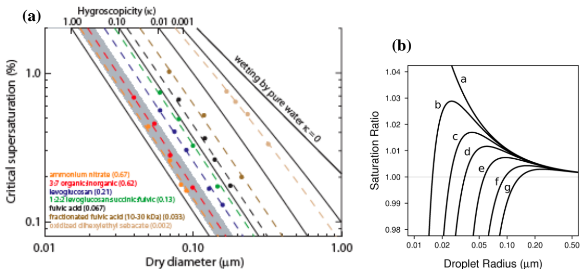
Figure 2.17: (a) s_c - D_d data for pure compounds, organic mixtures and organic-inorganic mixtures. Dashed lines indicate best-fit \kappa values for each particle type, as shown in the legend. Shaded area indicates reported range of values for ammonium sulfate. Kappa values were computed for where \sigma_{s/a} = 0.072 \text{ Jm}^{-2} and T = 298.15 \text{ K} (from Petters and Kreidenweis 2007); (b) Plots of the equilibrium vapor pressure for solution droplets with the following characteristic dissolved nuclei: a) r=10\text{nm} , \kappa=0 , b) r=10\text{nm} , \kappa=0.2 , c) r=10\text{nm} , \kappa=0.6 , d) r=10\text{nm} , \kappa=1.28 , e) r=25\text{nm} , \kappa=0.2 , f) r=25\text{nm} , \kappa=0.6 , g) r=25\text{nm} , \kappa=1.28 (provided by Dan Ward; produced with code created by Markus Petters, 2007).
