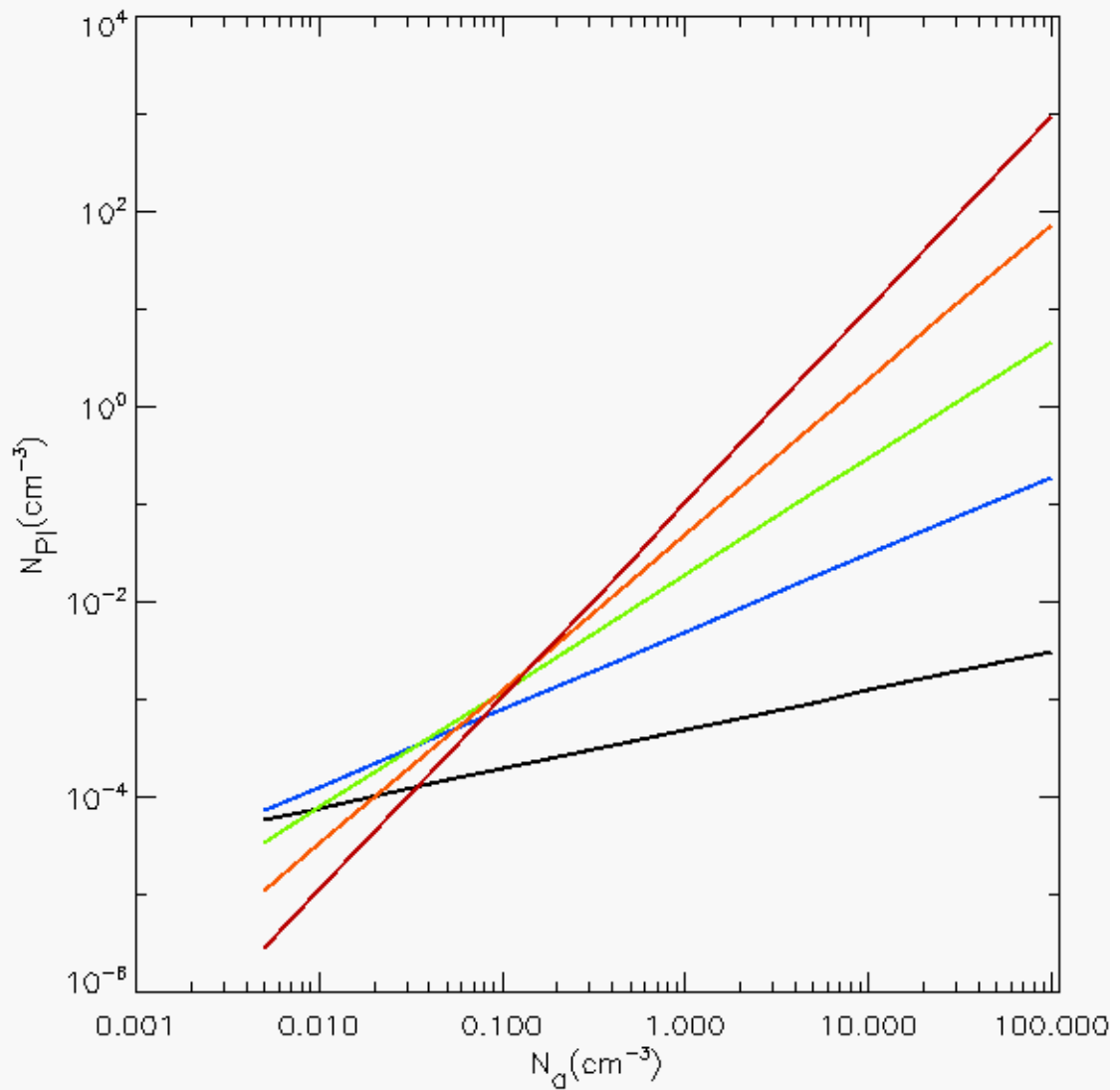
Figure 3.13: Activated IN concentrations in \text{cm}^{-3} , or pristine ice concentrations ( N_{PI} ), plotted as a function of initial potential IN concentrations in \text{cm}^{-3} (aerosol concentrations of particles with the potential to serve as IN with diameters greater than 0.5 \mu\text{m} , or N_a ) according to the DeMott et al. (2010) scheme, based on measurements at STP. The black line denotes IN activation at a temperature of -15^\circ\text{C} , blue -30^\circ\text{C} , green -45^\circ\text{C} , orange, -60^\circ\text{C} , and red -75^\circ\text{C} .
