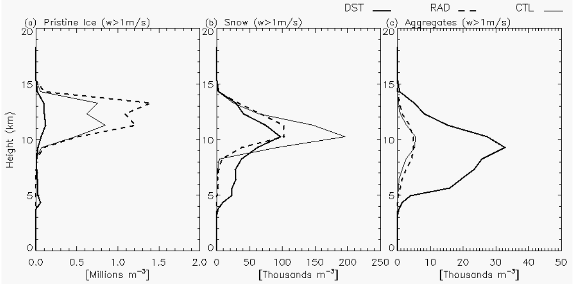
Figure 7.24: Mean profiles of (a) pristine ice, (b) snow, and (c) aggregate number concentrations within updrafts greater than 1 \text{ m s}^{-1} for the DST (thick solid), RAD (thick dashed), and CTL (thin solid) simulations at 0210 UTC in the SR2 region.
