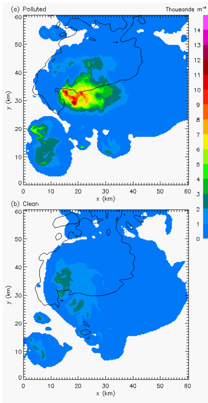
Figure 4.6: Hail number concentrations at 8.381 km on Grid 2 at 80 min for the (a) POL and (b) CLN simulations. The 30-dBZ model reflectivity boundaries at 1 km are overlaid for reference.
