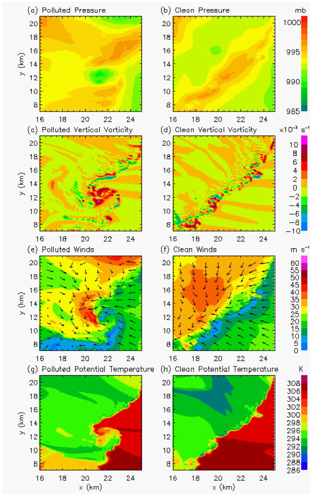
Figure 4.5: Grid 3 near-surface (24 m) pressure, vertical vorticity, horizontal winds overlaid with directional wind barbs, and potential temperature for the POL (left) and CLN (right) simulations at 100 minutes (from Lerach et al. 2008).
