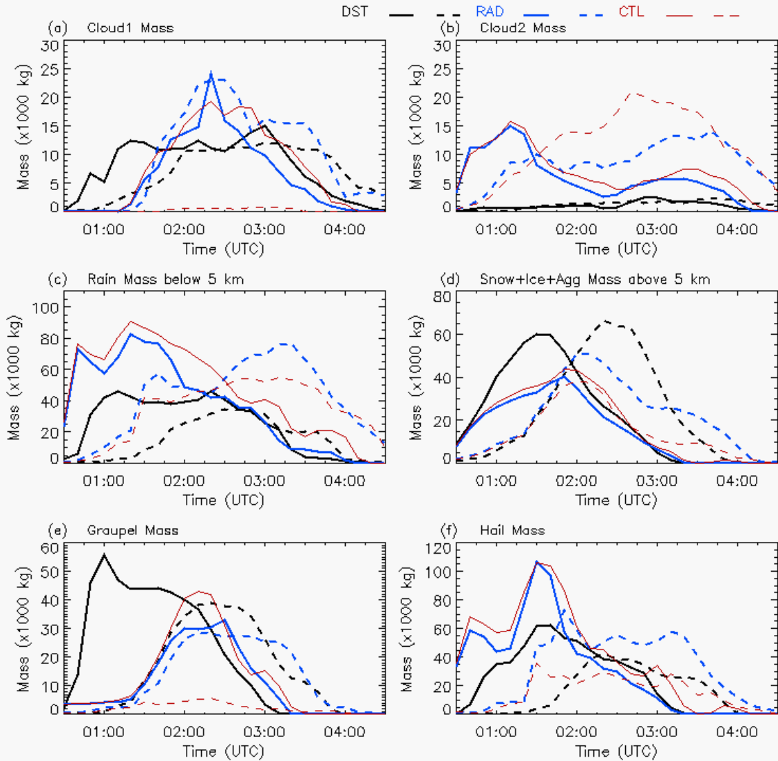
Figure 7.23: Time series of grid-cumulative (a) cloud1 mass, (b) cloud2 mass, (c) rain mass below 5 km, (d) pristine ice+snow+aggregate mass above 5 km, (e) graupel mass, and (f) hail mass on Grid 4 for the DST (black), RAD (blue), and CTL (red) simulations in the NR1 (solid) and SR2 (dashed) regions of the grid.
