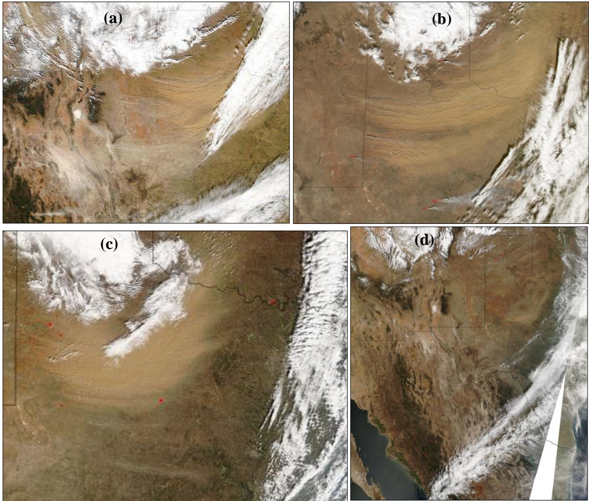
Figure 3.4: MODIS images of dust plumes originating over northwestern Texas and eastern New Mexico on (a) 15 December 2003, (b) 1 January 2006, (c) 24 February 2007, and (d) 6 April 2006 (Figs 3.4a-c from http://earthobservatory.nasa.gov ; Fig. 3.4d from http://visibleearth.nasa.gov )
