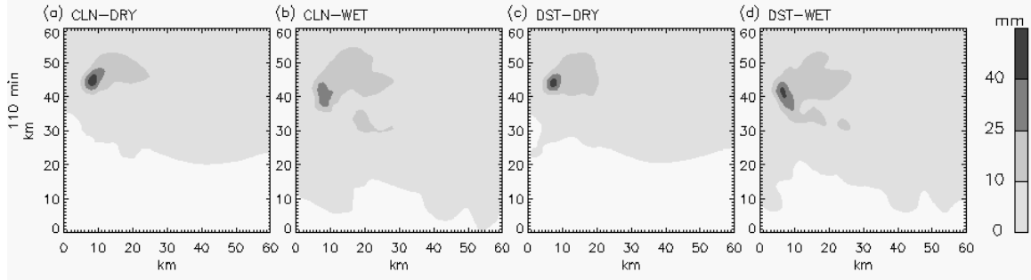
Figure 5.8: Accumulated precipitation on Grid 2 at 110 min for the (a) CLN-DRY, (b) CLN-WET, (c) DST-DRY, and (d) DST-WET simulations.
