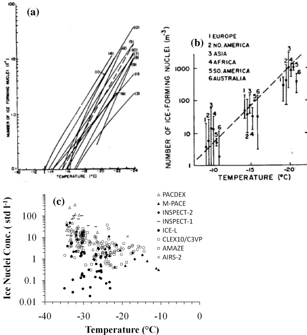
Figure 2.19: (a) Variation of mean or median IN number concentration with temperature and geographic location. (1) Bracknell, England; (2) Clermont-Ferrand, France; (3) Corvallis, Oregon; (4) Tokyo, Japan; (5) Tuscon, Arizona; (6) Jerusalem, Israel; (7) Palm beach, Florida; (8) Hawaii; (9) Swakopmund, South Africa; (10) Sindy, Australia; (11) Tasmania, Australia; (12) Antarctica. The dashed line represents N_{IN} = 10^{-5} \exp(0.6\Delta T) ; (b) Range of median IN number concentration as a function of temperature for various geographic locations, based on 44 stations. The dashed line represents N_{IN} = 10^{-5} \exp(0.6\Delta T) ; (c) IN number concentration (at STP) active at water saturation or above as a function of temperature for various experiments (adapted from DeMott et al. 2010).
