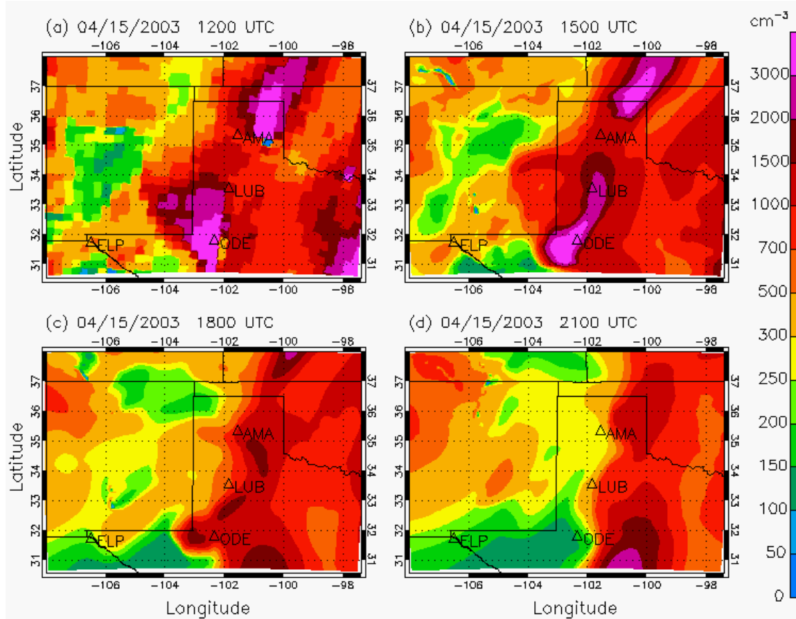
Figure 7.2: Near-surface CCN on Grid 2 at (a) 12 UTC, (b) 15 UTC, (c) 18 UTC, and (d) 21 UTC on 15 April 2003.
