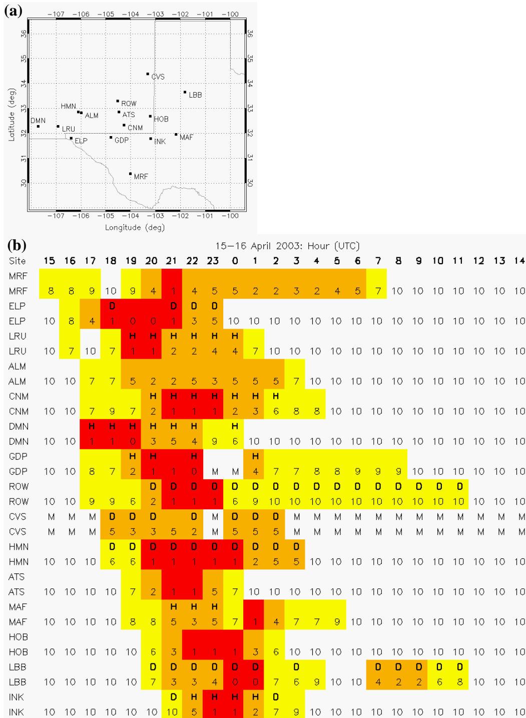
Figure 6.10: (a) METAR site locations that reported dust, haze and/or reduced visibility during 15-16 April 2003, (b) Dust, haze, and visibility METAR observations for 15-16 April 2003 as a function of time (hourly reports) and surface station (three letter identifiers). Dust and haze reports are denoted by ‘D’ and ‘H’, respectively. Visibility is represented numerically with units of statute miles. Yellow highlighting denotes a report of visibility < 10 statute miles and/or a direct report of dust. Orange (red) denotes visibility \leq 5 ( \leq 1 ) statute miles. ‘M’ indicates missing data.
