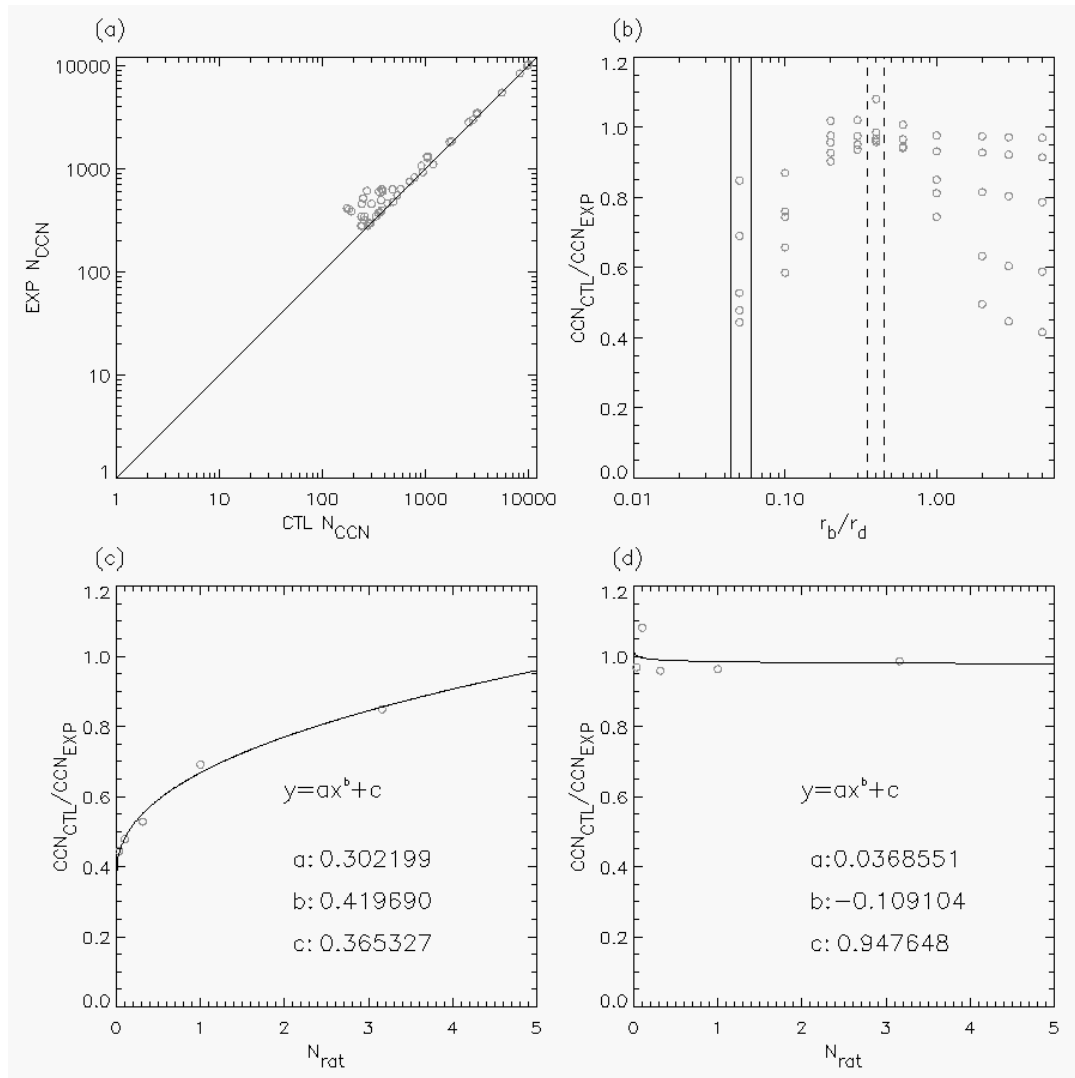
Figure 3.8: Plots of (a) CTL vs. EXP activated CCN ( \text{cm}^{-3} ) and (b) median aerosol size ratio vs. CCN activation ratio for w=0.361\text{ms}^{-1} , \kappa_b=0.6 , T=10^\circ\text{C} , and N_d=316 ; (c) aerosol number concentration ratio vs. CCN activation ratio for an aerosol size ratio 0.05, shown as the data points surrounded by the two solid vertical lines in Fig. 3.8b; (d) same as (c) but for an aerosol size ratio of 0.4, shown as the data points in between the two dashed vertical lines in Fig. 2b. The black line in Fig. 3.8a represents the one-to-one line. The curves overlaid on Fig. 3.8c-d represent the best-fit geometric curves to the plotted data, represented by the parameters a , b , and c .
