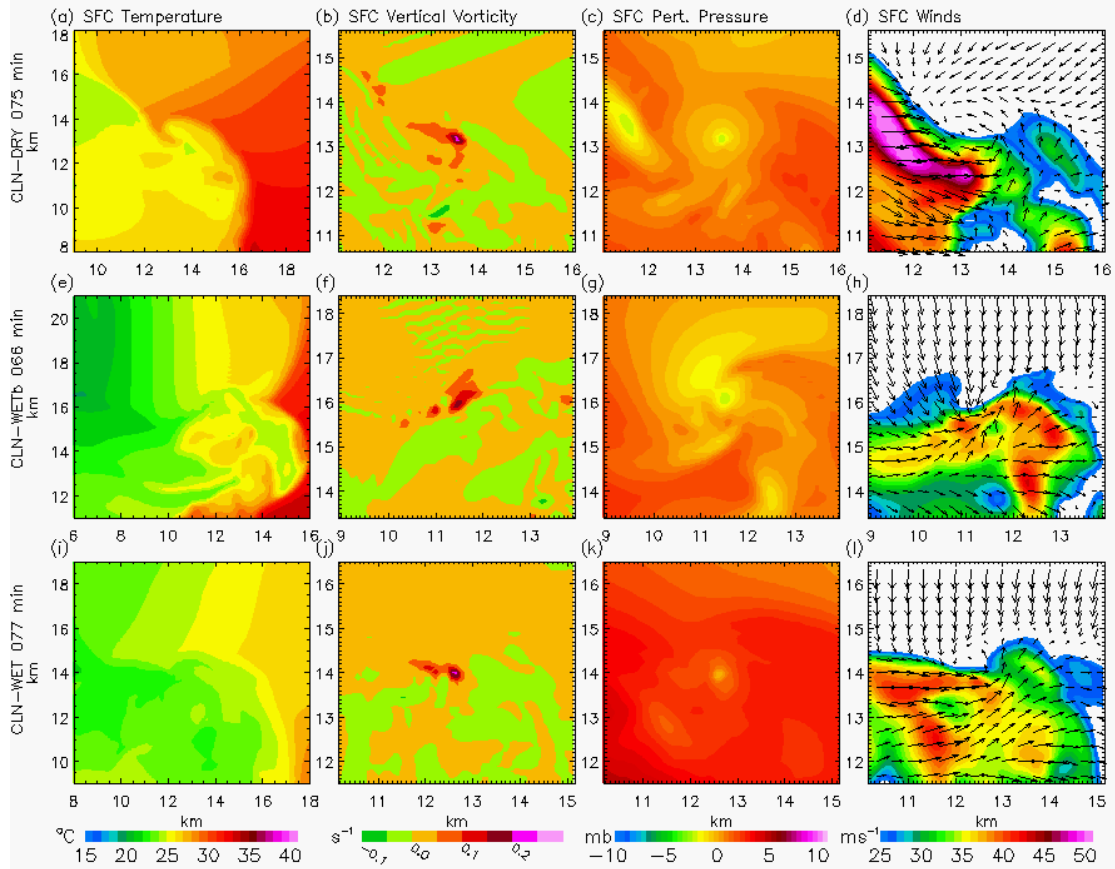
Figure 5.14: Same as Fig. 9 but for the CLN-DRY simulation at 75 min (row 1), the CLN-WETb (row 2) simulation at 66 min, and the CLN-WET (row 3) simulation at 77 min.
