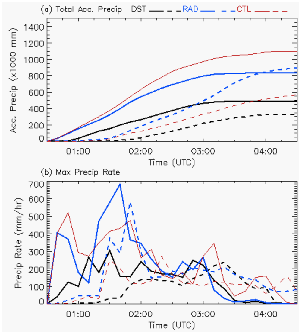
Figure 7.15: Time series of (a) grid-cumulative accumulated precipitation and (b) maximum precipitation rates on Grid 4 for the DST (black), RAD (blue), and CTL (red) simulations in the NR1 (solid) and SR2 (dashed) regions of the grid.
