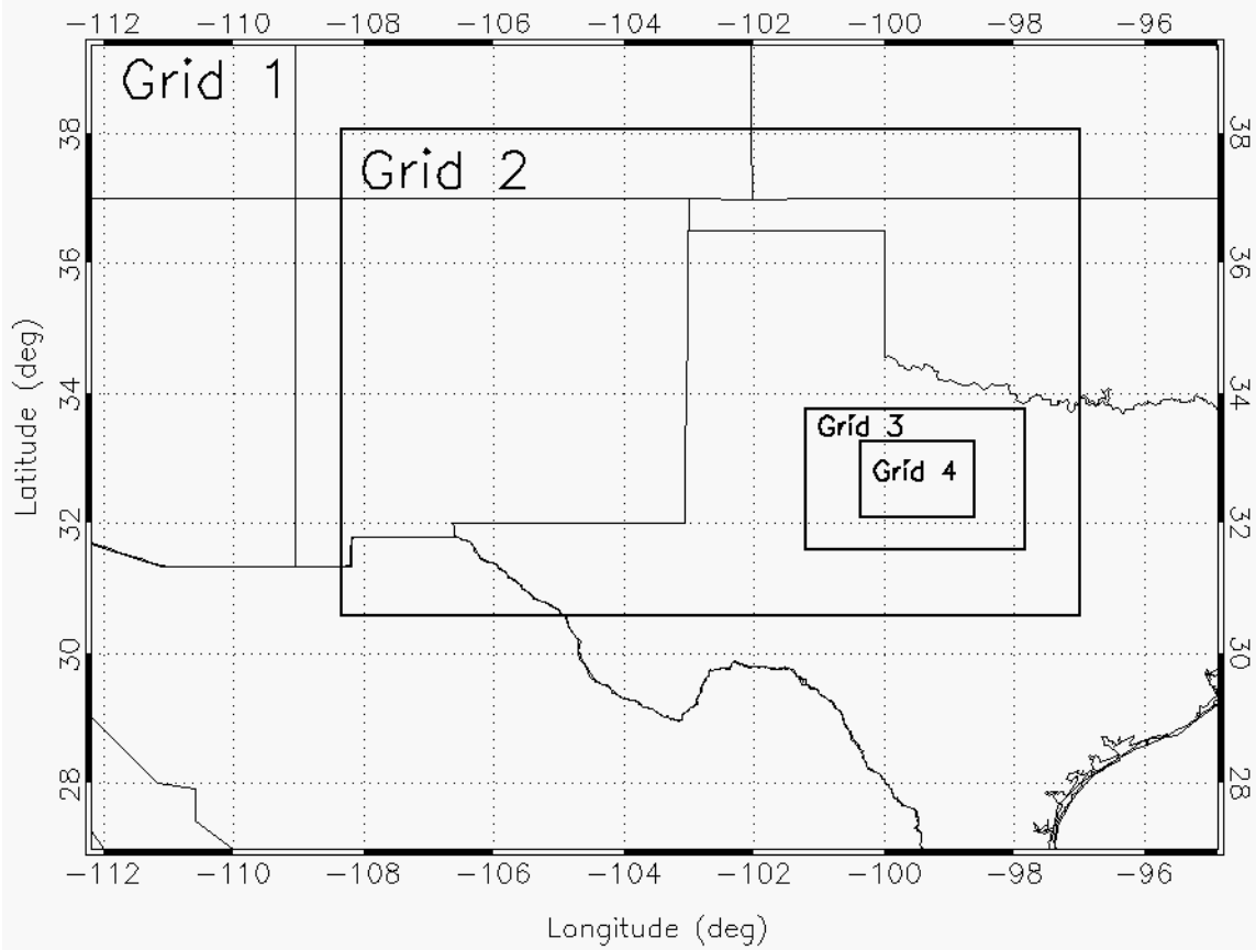
Figure 7.1: The four nested model grid configuration used for the 15-16 April 2003 case simulations.
