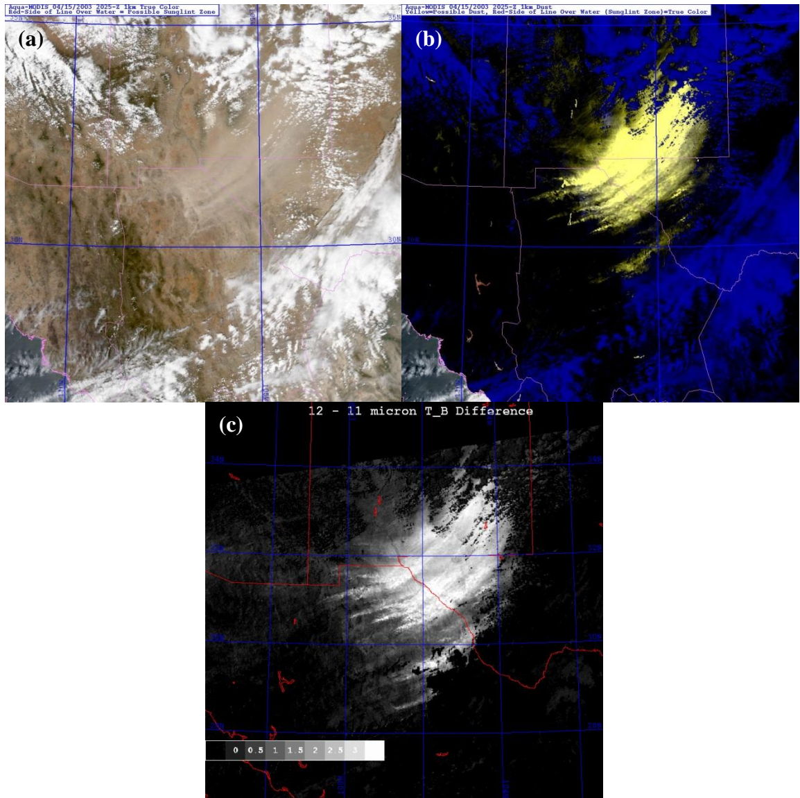
Figure 6.11: Images of a major dust plume centered over the southwestern U.S. and the Chihuahuan Desert region of Mexico on 15 April 2003 at 2020 UTC: (a) MODIS visible composite, (b) application of a sophisticated dust detection algorithm supplied by Steven Miller of CIRA, and (c) application of the “split window” technique.
