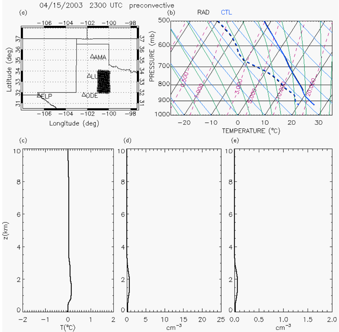
Figure 7.26: Mean sounding comparisons on Grid 2 between the RAD and CTL simulations at 2300 UTC on 15 April within the pre-storm environment between 32 and 34° latitude and between -101 and -100° longitude, where VIC was less than 0.01 mm: (a) grid cells used for mean calculations; (b) Skew-T log p diagrams of the mean RAD (black) and CTL (blue) thermodynamic profiles below 500 mb; (c) mean temperature differences between the RAD and CTL simulations (RAD-CTL); (d) mean profile of mode 1 dust number concentrations; (e) mean profile of mode 2 dust number concentrations.
