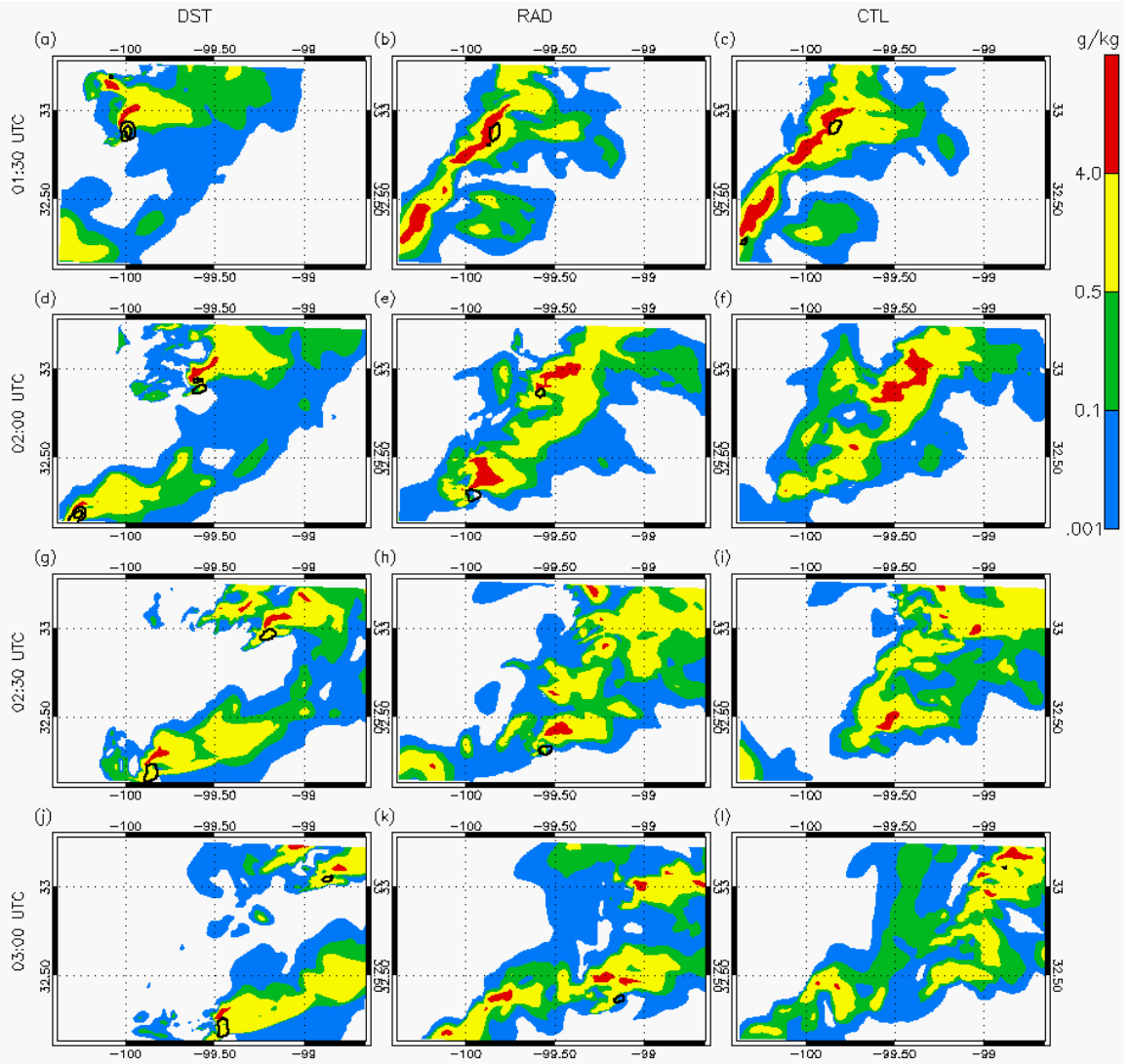
Figure 7.9: Total condensate at 1 km on Grid 4 for the DST (column 1), RAD (column 2), and CTL (column 3) simulations on 16 April at 0130 (row 1), 0200 (row 2), 0230 (row 3), and 0300 UTC (row 4). 3.5-km vertical velocity is overlaid at 10 and 20 \text{m s}^{-1} .
