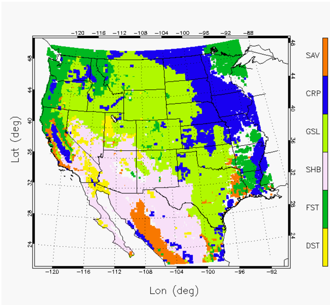
Figure 3.5: Dominant vegetation classifications derived from the MODIS land cover product for April 2003, generalized and grouped in six primary land type classifications: savannas (SAV), croplands (CRP), grasslands (GSL), shrub lands (SHB), forest (FST), and desert or barren land (DST).
