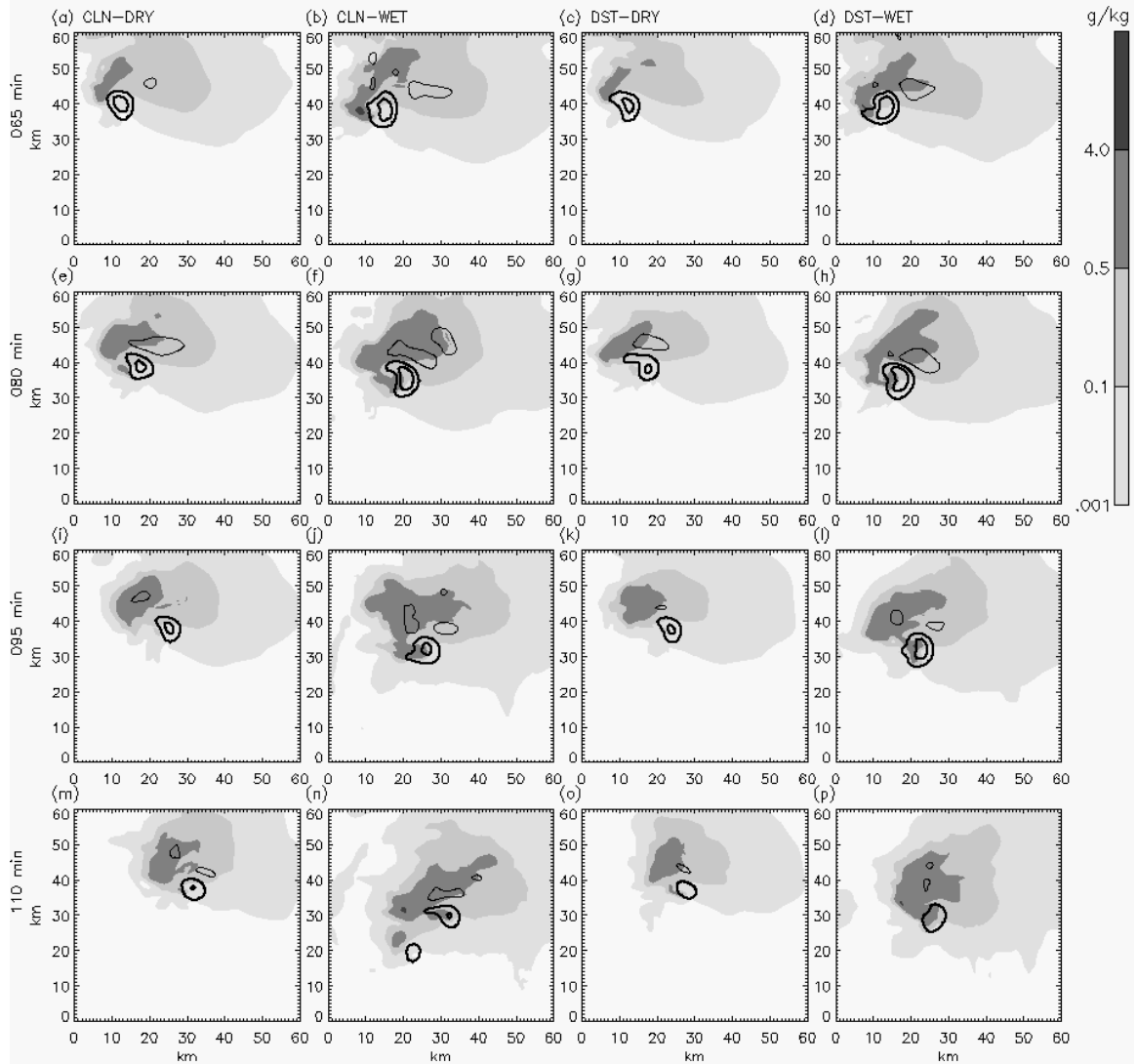
Figure 5.2: Total condensate at 1 km on Grid 2 at 65, 80, 95, and 110 min (rows 1-4, respectively) for the CLN-DRY, CLN-WET, DST-DRY, and DST-WET (columns 1-4, respectively) simulations. Vertical velocities of -5 , 10 , and 20 \text{ m s}^{-1} at 3.5 km are overlaid with thick (thin) contours for updrafts (downdrafts).
