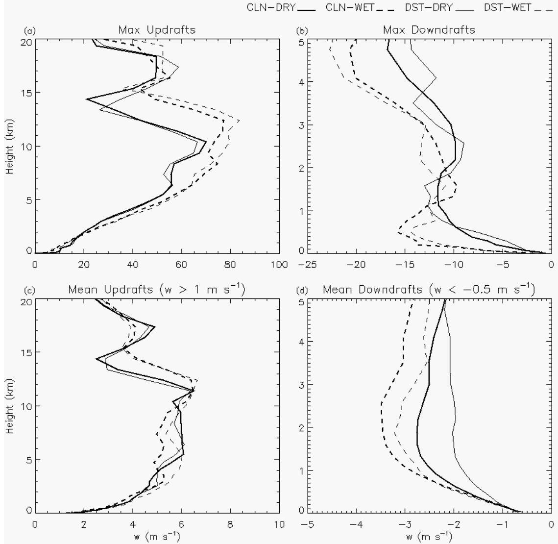
Figure 5.3: Profiles of (a) peak updrafts, (b) peak downdrafts, (c) mean updrafts for all updrafts greater than 1 \text{ m s}^{-1} , and (d) mean downdrafts for all downdrafts stronger than 0.5 \text{ m s}^{-1} on Grid 2. Updraft profiles are shown up to 20 km; low-level downdrafts are shown up to 5 km.
