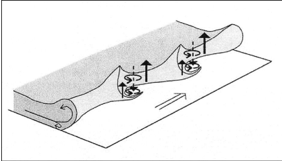
Figure 2.11: Schematic diagram describing the mature misocyclone structure along a north-south boundary (from Lee and Wilhelmson 1997a).
