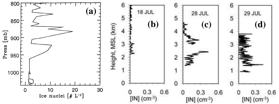
Figure 2.20: Vertical profiles of IN concentrations from (a) over the Arctic ice sheet during the 1998 FIRE/SHEBA field campaign (from Jiang et al. 2000) and within the Saharan Air Layer (SAL) observed during CRYSTAL-FACE on (b) 18 July, (c) 28 July, and (d) 29 July 2002 (from DeMott et al. 2009).
