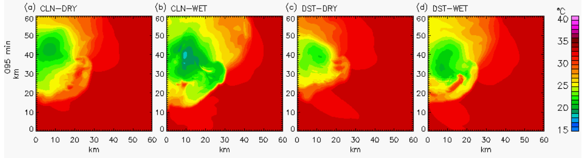
Figure 5.4: Near-surface (24 m) temperature on Grid 2 at 95 min for the (a) CLN-DRY, (b) CLN-WET, (c) DST-DRY, and (d) DST-WET simulations.
