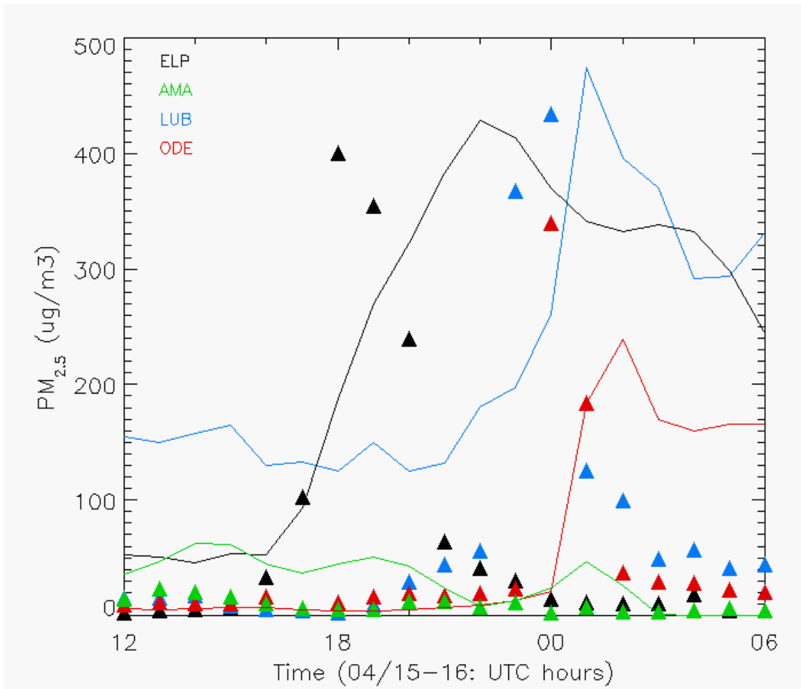
Figure 7.5: Time series of simulated total dust mass concentrations on Grid 2 from the DST experiment (solid curves) and observed PM 2.5 mass concentrations (filled triangles) at El Paso (ELP; black), Amarillo (AMA; green), Lubbock (LUB; blue), and Odessa (ODE; red).
