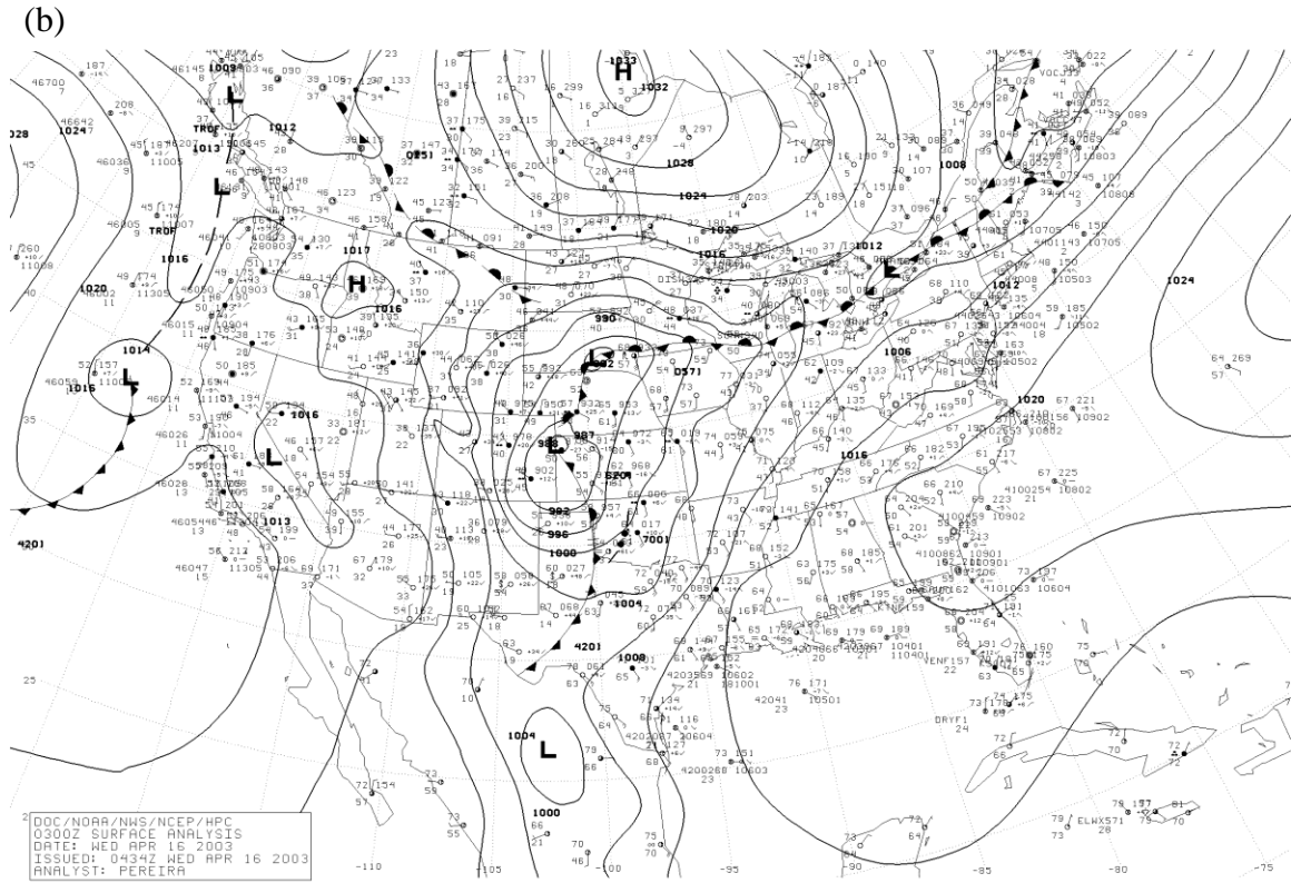
Figure 6.7: National Oceanic and Atmospheric Administration (NOAA) surface analyses from (a) 15 April 2003 at 15 UTC and (b) 16 April 2003 at 3 UTC.
