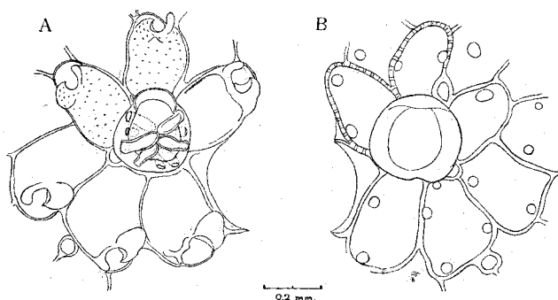
Fig. 13. Schizoporella kiiensis Okada and Mawatari
