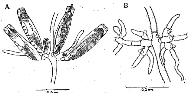
Fig. 1. Valkeria uva (Linnaeus) A Several functional zooecia. B A Stolon showing the mode of branching.
