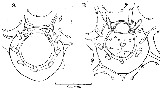
Fig. 14. Fenestulina malusii (Audouin) A Usual type of ancestrula B Ancestrula with orifice and ascopore.
