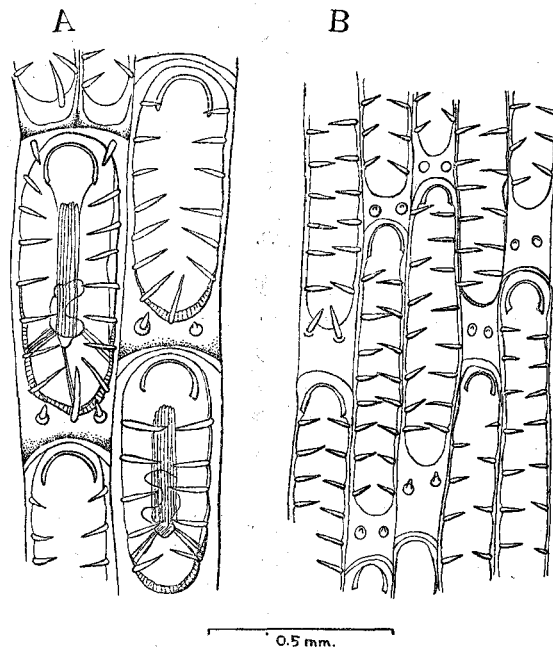
Fig. 2. Electra tenella (Hincks) A normal type of zoecia with narrow proximal cryptocyst. B Unusual elongate form.
