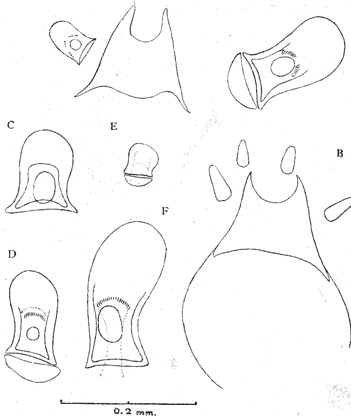
Fig. 17. Escharoides sauroglossa Levinsen A Normal position of operculum and mandibles. B Normal position of operculum and compensatrix C-F Spatulate mandibles
