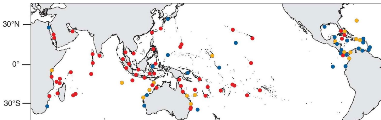
Figure 6 The global extent of mass bleaching of corals in 2015 and 2016. Symbols show 100 reef locations that were assessed: red circles, severe bleaching affecting >30% of corals; orange circles, moderate bleaching affecting <30% of corals; and blue circles, no substantial bleaching recorded (Source: Hughes et al. 2018).
