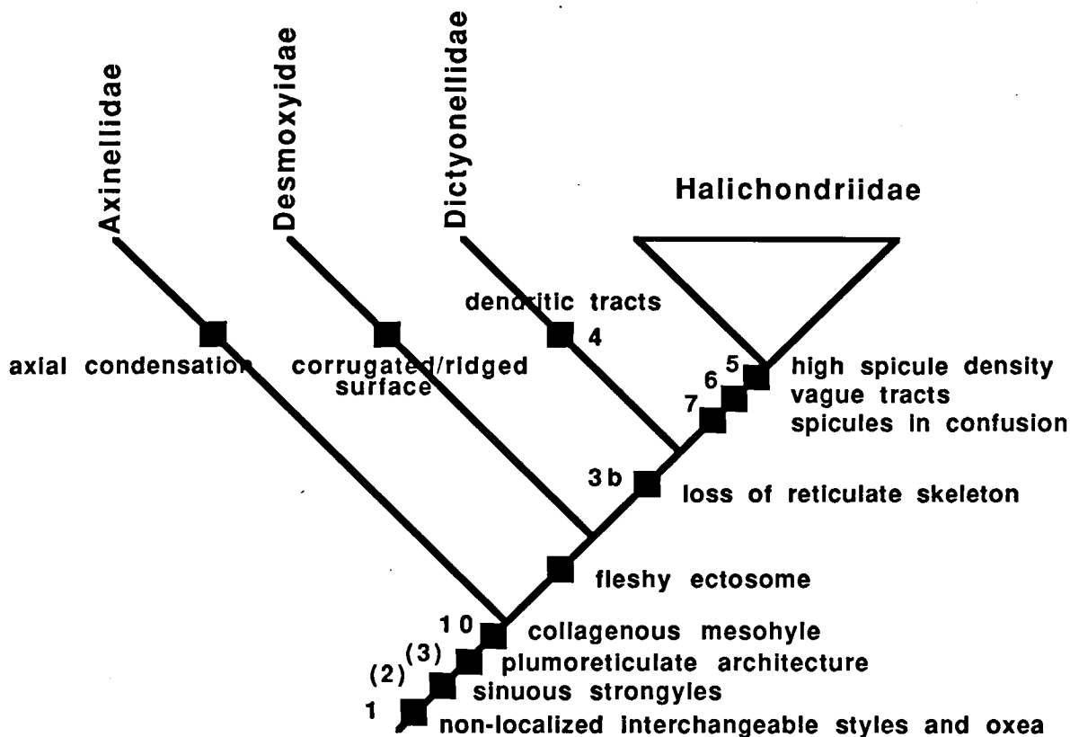
Fig. 12. Phylogenetic relationships of newly defined Halichondrid families (further explanations see text).
