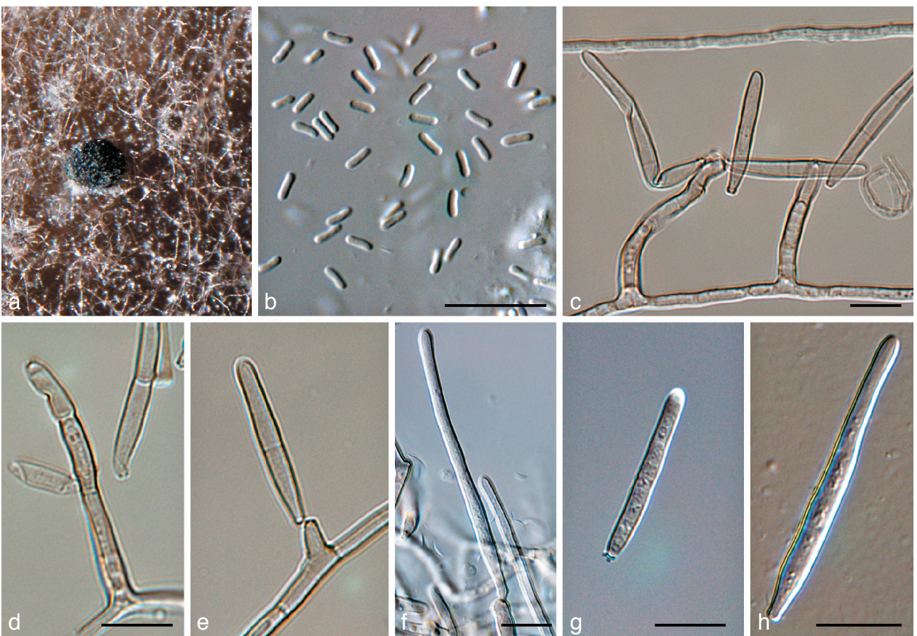
Fig. 4 Passalora intermedia (CPC 15745). a. Spermatogonium forming on OA; b. spermatia; c–f. conidiophores giving rise to conidia; g, h. conidia. — Scale bars = 10 µm.
