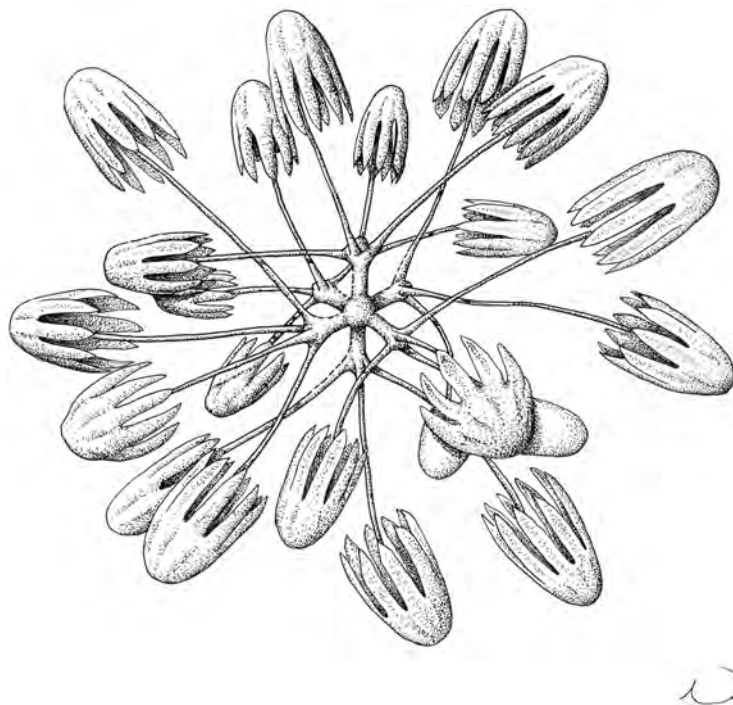
Figure 7 Schematic illustration of Bolosoma perezii sp. nov. codonhexaster (Illustration by Nicholas Bezio). Full-size DOI: 10.7717/peerj.9431/fig-7
