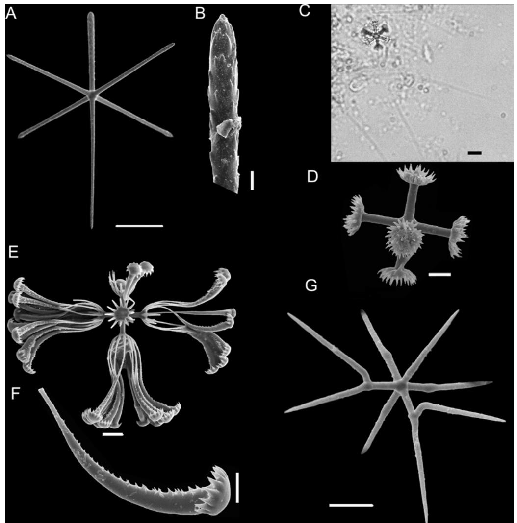
Figure 5 Euplectella sanctipauli sp. nov. scicules. (A) Dermal/atrial hexactin with sword-shaped distal ray; (B) Detail of hexactin sword-shaped distal ray; (C) Graphiome and secondary rays; (D) Graphiome without secondary rays; (E) Floricome; (F) Detail of apical portion of floricome secondary ray; (G) Hemioxyhexaster. Scales: (A) 100 \mu\text{m} ; (B and C) 10 \mu\text{m} ; (D and F) 5 \mu\text{m} ; (E and G) 10 \mu\text{m} .
