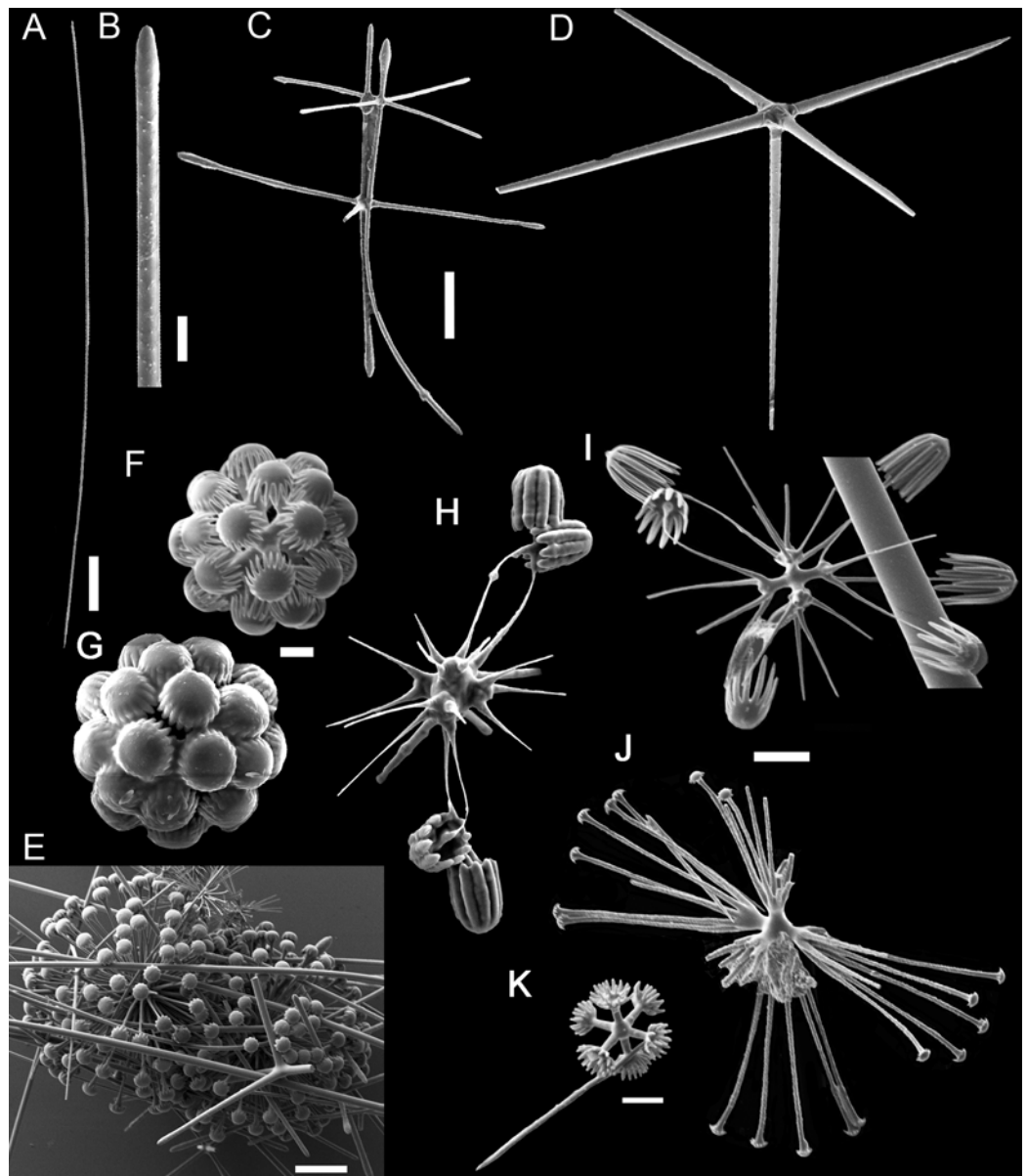
Figure 9 Advhena magnifica sp. nov. (A) diactin; (B) detail of hexactin extremity; (C and D) pentactins; (E) discasters (discohexaster); (F and G) discohexaster; (H and I) codonhexasters (J) calydiscohexasters (partially broken); (K) graphiocomes (primary rays with one of the secondary rays). Scales: (A) 250 \mu\text{m} ; (B, H, I and J) 20 \mu\text{m} ; (C–E) 100 \mu\text{m} ; (F, G, J and K) 10 \mu\text{m} .
