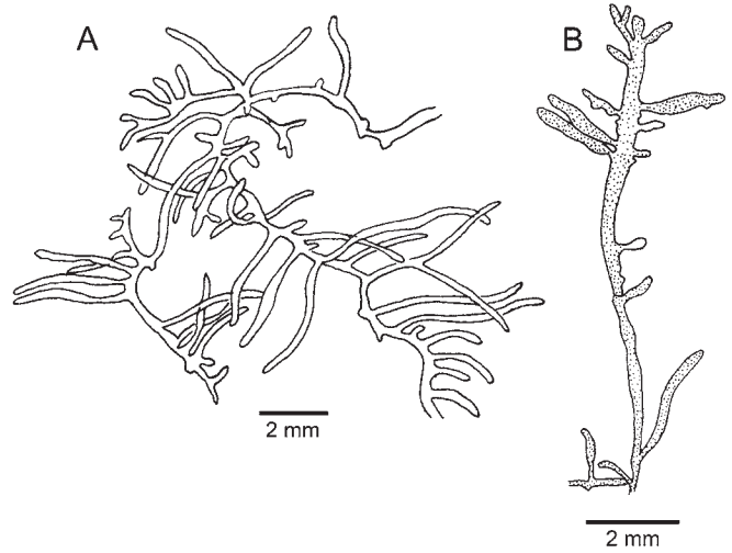
FIGURE 155. Species of Gelidiella and Pterocliadiella . A. Gelidiella hancockii : Habit (after Dawson, 1944a: pl. 43: fig. 1). B. Pterocliadiella caloglossoides : A small, suberect branch from the type collection (after Dawson, 1953a: pl. 6: fig. 2, as Pterocliadia parva ).
