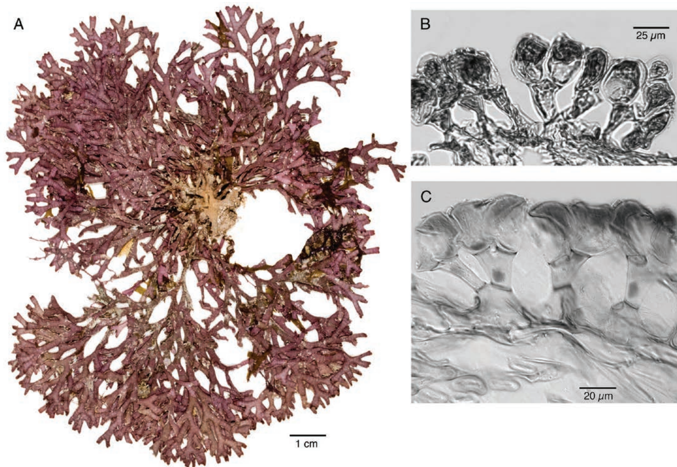
FIGURE 25. Dichotomaria spathulata : A. Habit, tetrasporophyte (JN-5859, US Alg. Coll.-159150). B, C. Portion of transverse sections through sporophyte cortex showing loosely arranged stalk-like cells bearing 1–2 subspherical, nonapiculate ultimate cortical cells (B, JN-4891b, US Alg. Coll. microscope slide 8708; C, JN-2941, US Alg. Coll. microscope slide 5366).
