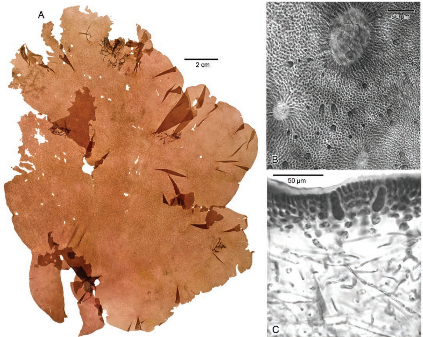
FIGURE 218. Schizymenia pacifica : A. Habit (female gametophyte) (JN-5759, US Alg. Coll.-160898). B. Surface view showing gland cells in cortex and several carpostomes of cystocarps, the largest with carposporangia visible within (JN-5747c, US Alg. Coll. microscope slide 4524). C. Portion of transection showing elongate gland cells terminating cortical filaments (JN-5747, US Alg. Coll. microscope slide 4526).
