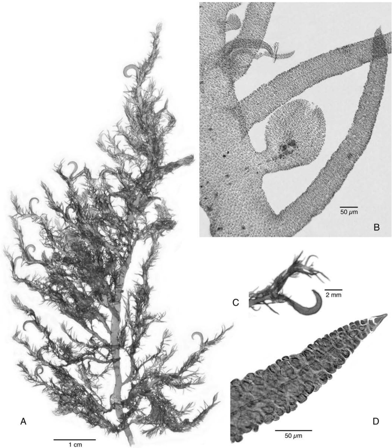
FIGURE 65. Bonnemaisonia hamifera : A. Habit (gametophyte) with hook-shaped branchlets for entangling attachment ( JN-5438 , US Alg. Coll.-158653). B. Branch with developing and young cystocarps terminating short branches ( JN-2989 , US Alg. Coll. microscope slide 4277). C. Close-up of a hook branchlet (from A; JN-5438 ). D. Ultimate branchlet showing central axial filament surrounded by cortical cells, tapering to acute apex ( JN-2989 , US Alg. Coll. microscope slide 4277).
