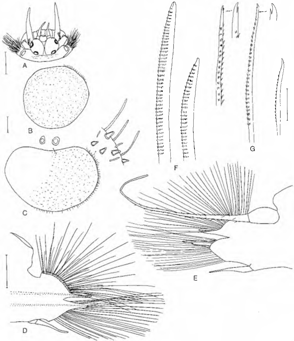
Fig. 3. Harmothoe craigsmiti , holotype (USNM 157590): A, Dorsal view of anterior end, styles of median antenna and tentacular cirri missing; B, Right 1st elytron; C, Right middle elytron, with detail of microtubercles and papillae; D, Left elytrigerous parapodium, anterior view, acicula dotted; E, Left middle cirriferous parapodium, posterior view; F, Long and short notosetae from same; G, Upper, middle and lower neuroseta from same, with detail of parts. Scales = 0.1 mm for A; 0.5 mm for B, C; 0.5 mm for D, E; 0.1 mm for F, G.
