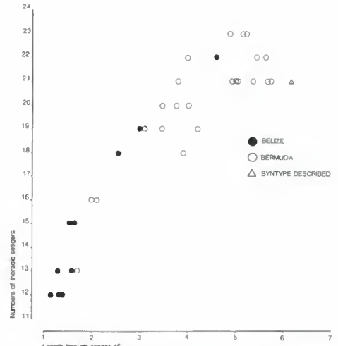
Fig. 3. Relationship between length through setiger 15 and number of thoracic setigers in N. setosa from Belize and Bermuda.
