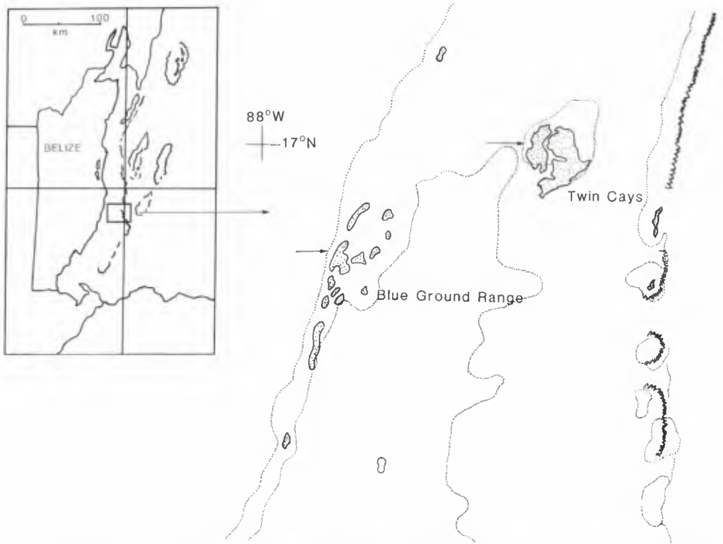
Fig. 1. Study area in Belize. The box to the left indicates the position of the study areas in relation to Belize; the study area is enlarged on the right. The two arrows in the enlargement indicates West Bay, Twin Cays and the un-named cay in the Blue Ground Range at which the collections were made.
