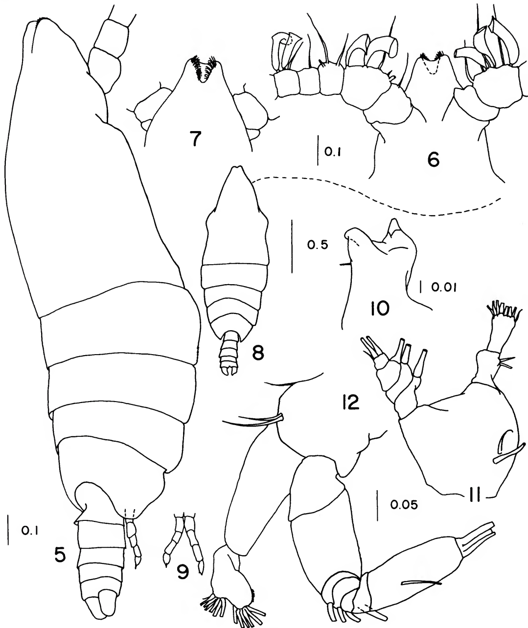
FIGURES 5-12.— Mimocalanus sulcifrons , new species, male: 5, adult, lateral view; 6, anterior end of head, ventral view; 7, anterior end of head, dorsal view; 8, adult, dorsal view; 9, male fifth legs; 10, gnathal lobe of mandible; 11, mandibular palp; 12, second antenna.
