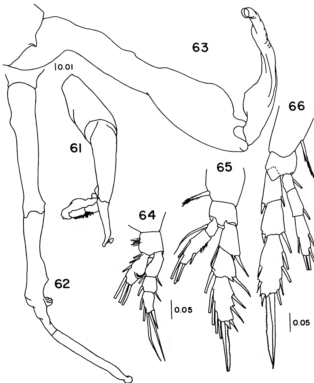
FIGURES 61-66.— Undinella gricea , new species, male: 61, exopod of left fifth leg; 62, endopod of left fifth leg; 63, right fifth leg; 64, first leg; 65, second leg; 66, fourth leg.
