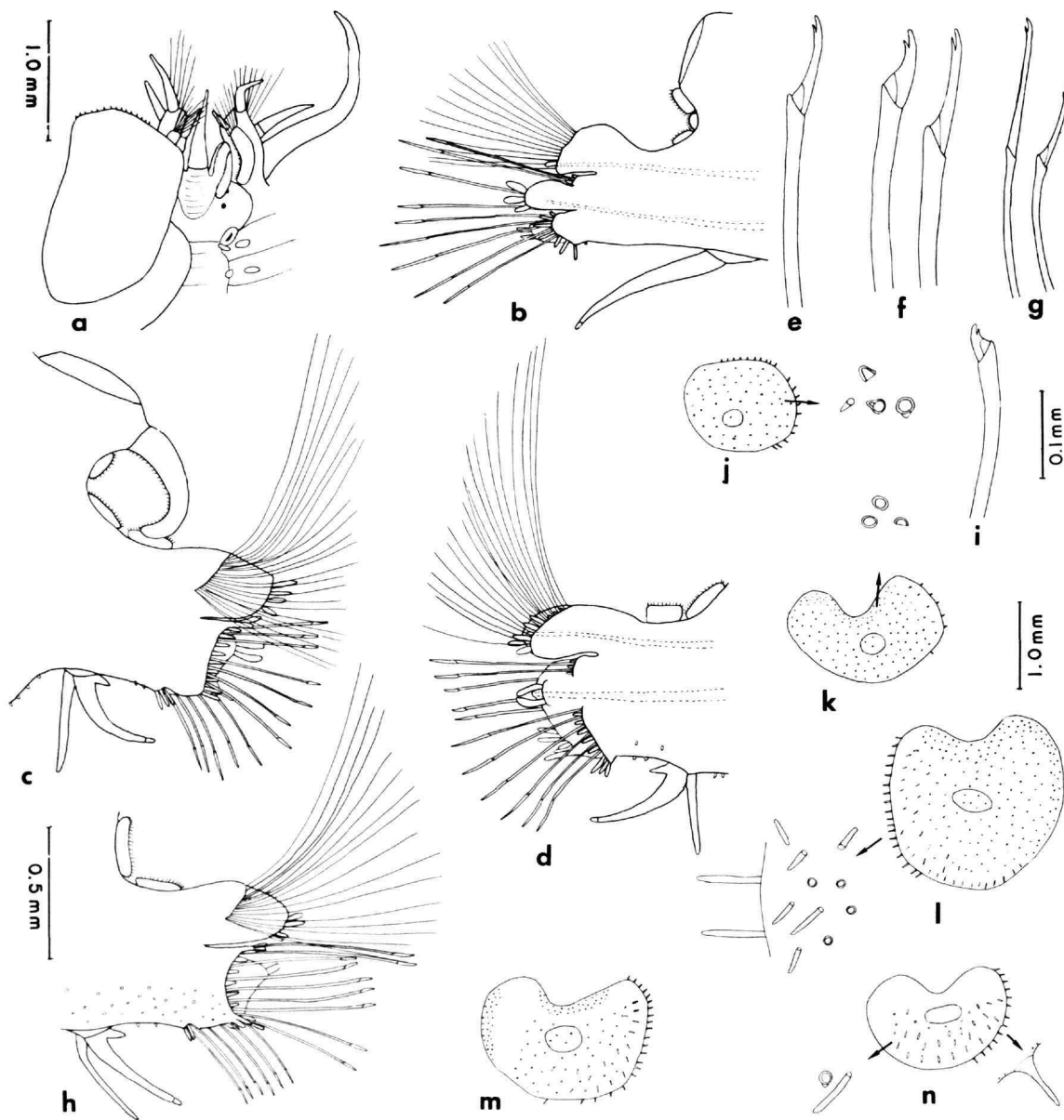
FIGURE 13.— Willeysthenelais suezensis new species (holotype, BMNH 1926: 11: 12: 20–22): a , Anterior end, dorsal view; b , second parapodium, anterior view; c , parapodium from anterior region, posterior view; d , same, anterior view; e , upper neuroseta from same; f , middle neurosetae from same; g , lower neurosetae from same; h , parapodium from middle region, posterior view; i , middle neuroseta from same; j , first elytron; k , second elytron; l , elytron from anterior region; m , elytron from middle region; n , elytron from posterior region.
