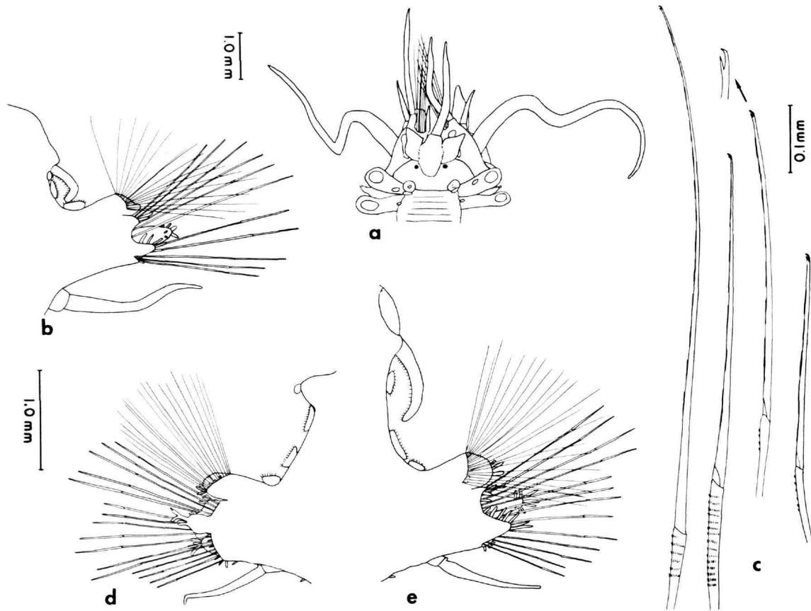
FIGURE 9.— Willeythenelais horsti , new species (holotype, ZMA 1387.5): a , Anterior end, dorsal view, pharynx everted, causing prostomium to appear much wider than long; parapodia of segments II–IV not shown; b , second parapodium, posterior view; c , upper, middle and lower neurosetae from same; d , third parapodium, anterior view, e , fourth parapodium, posterior view.
