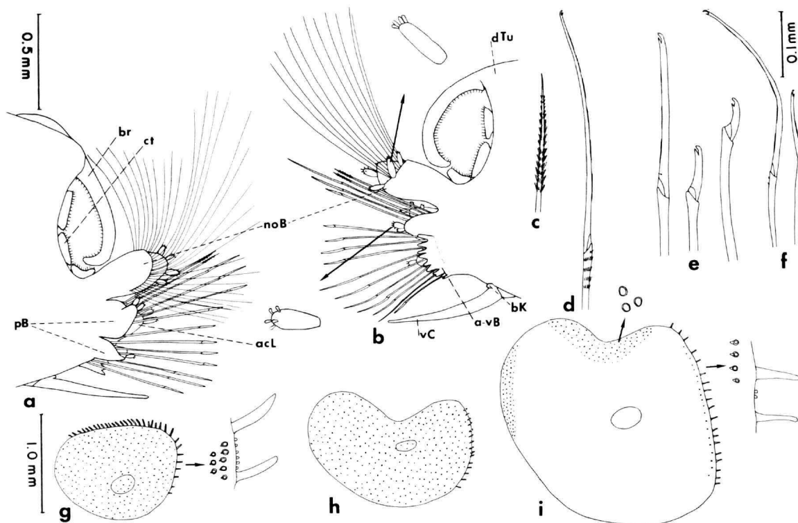
FIGURE 16.— Fimbristhenelais longipinnis (syntype of Sthenelais dubiosa , ZMA 1388): a , Parapodium from anterior region (about segment 25), posterior view; b , same, anterior view; c , upper simple neuroseta from same; d , upper compound falcigerous neuroseta from same; e , middle neurosetae from same; f , lower neurosetae from same; g , right first elytron; h , right third elytron; i , right 13th elytron.
