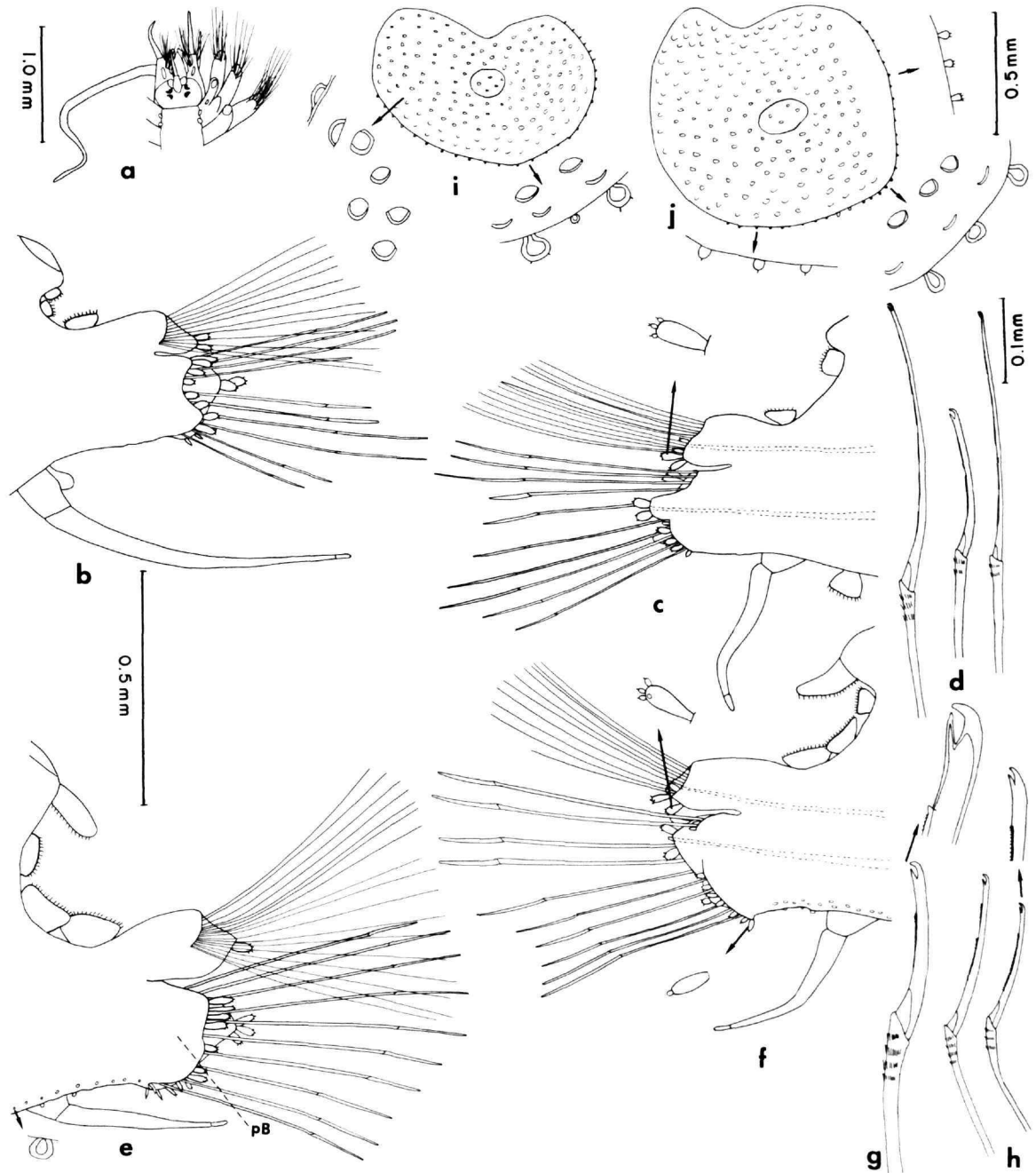
FIGURE 21.— Fimbriosthenelais zetlandica (holotype of Sthenelais vachoni , MNHNP): a , Anterior end, dorsal view; b , second parapodium, posterior view; c , third parapodium, anterior view; d , upper, middle, and lower neurosetae from same; e , parapodium from anterior region, posterior view; f , same, anterior view; g , middle neuroseta from same; h , lower neurosetae from same; i , right third elytron; j , elytron from anterior region.
