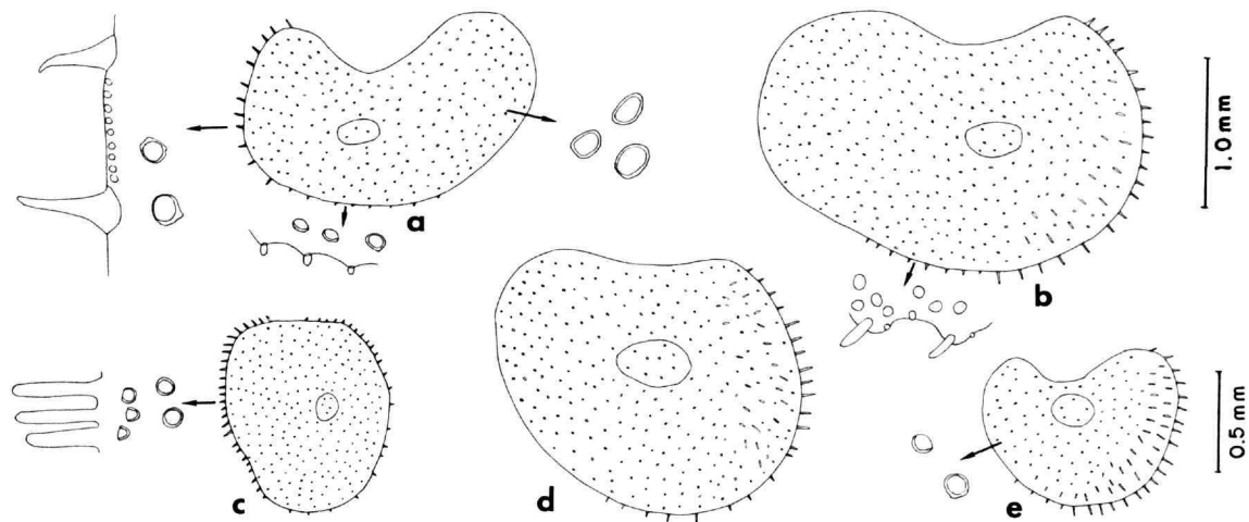
FIGURE 19.— Fimbristhenelais hirsuta (a,b, holotype of Sthenelais calcarea , BMNH 1924: 3: 1: 92; c-e, holotype of Sthenelais dahli , ZMB 6551): a, Left second elytron; b, right elytron from anterior region; c, left first elytron; d, right elytron from anterior region; e, right elytron from middle region.
