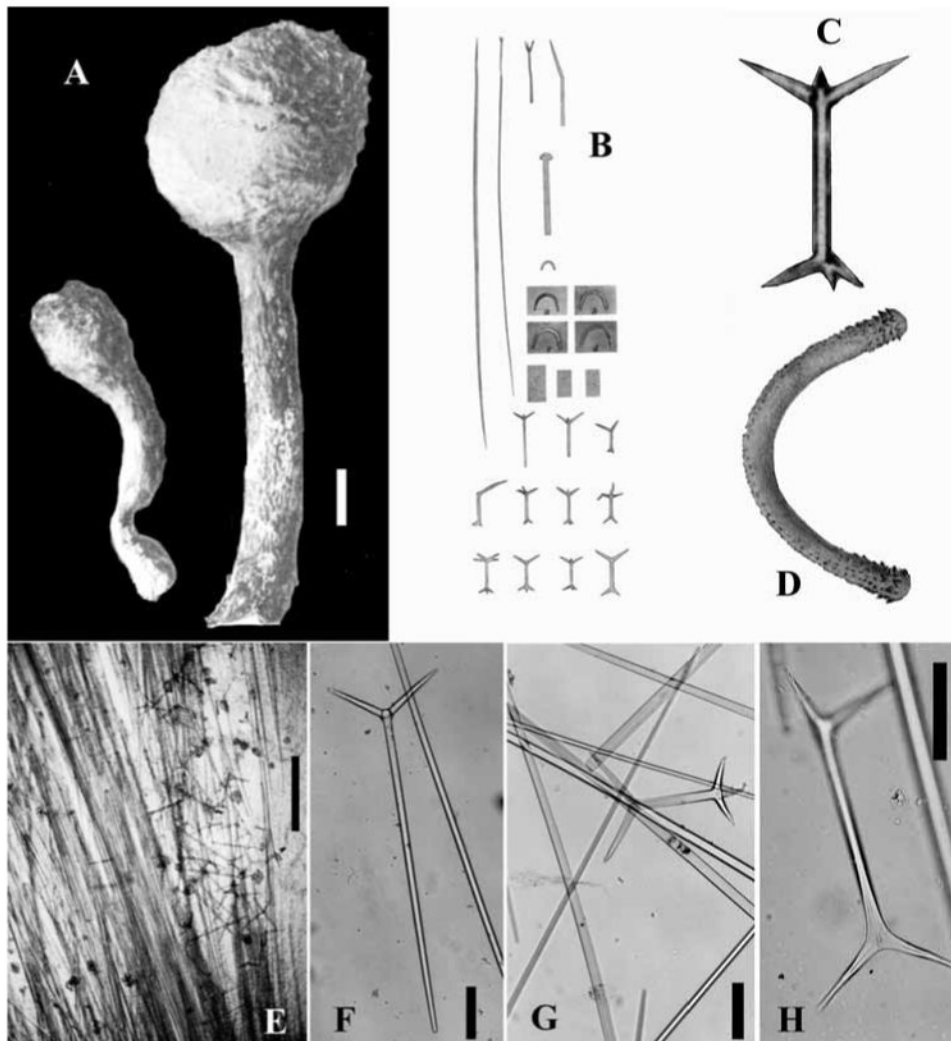
Fig. 2. Amphitethya microsigma Lendenfeld, 1907. A–D, habit and spicules reproduced from Lendenfeld, pl. XV fig. 19–3. A, habit (scale 1 cm). B, spicules. C, detail of amphitriaene. D, detail of sigmaspire (sizes see text). E–H, photos of spicules made from slides of one of the types kept in BMNH. E, cross section of peripheral region of peduncle (scale 500 \mu\text{m} ). F, plagiotriaene (scale 100 \mu\text{m} ). G–H, amphitriaenes (scale 100 \mu\text{m} ).
