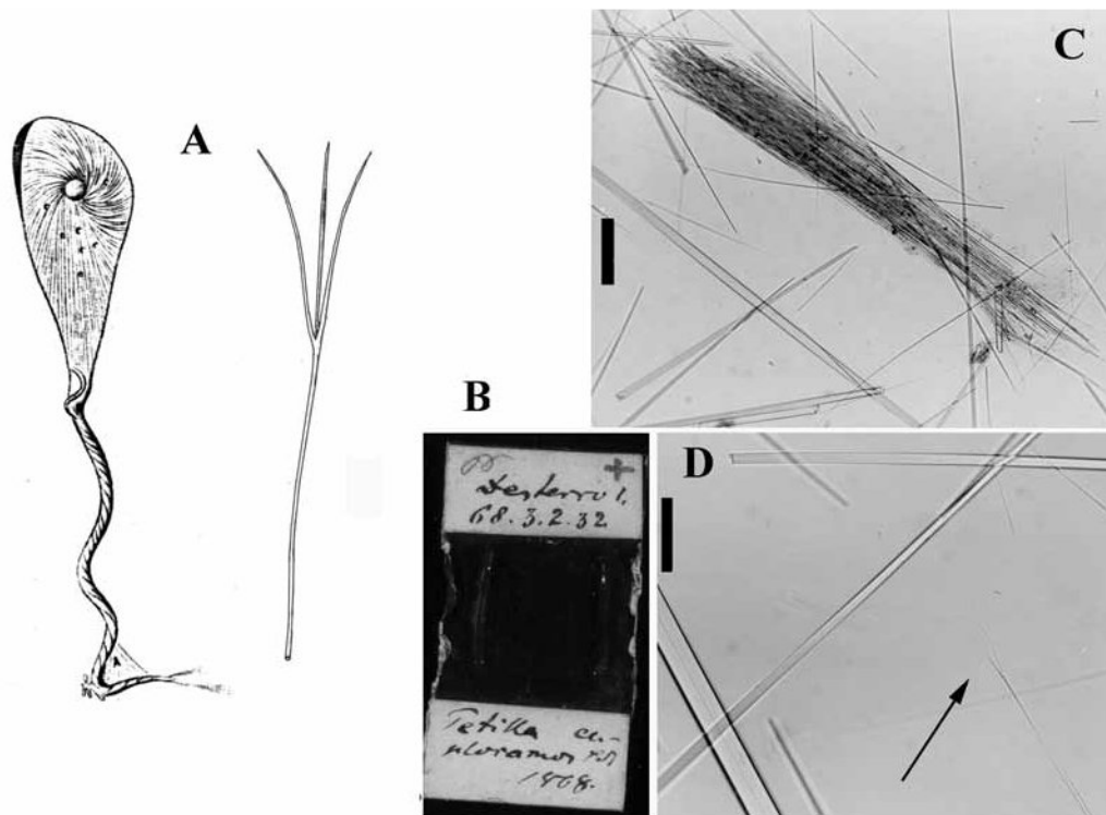
Fig. 9. Tetilla euplocamos Schmidt, 1868. A, drawing of type and protriaene reproduced from Schmidt, 1868: pl. V fig. 10 (sizes see text). B, BMNH slide of type. C–D, photos of spicules from BMNH slide. C, oxeads and bundle of small? protriaenes (scale 100 \mu m). D, protriaene (arrow) (scale 100 \mu m).
