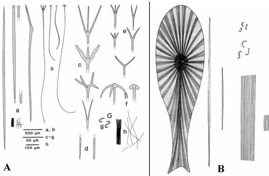
Fig. 5. A, Cinachyrella apion (Uliczka, 1929), drawing of spicules, reproduced from Rützler & Smith (1992: fig. 7). B, Cinachyrella enigmatica (Burton, 1934a as Raphidotethya ), drawing of cross section and spicules reproduced from Burton's fig. 2 (scales see text).
