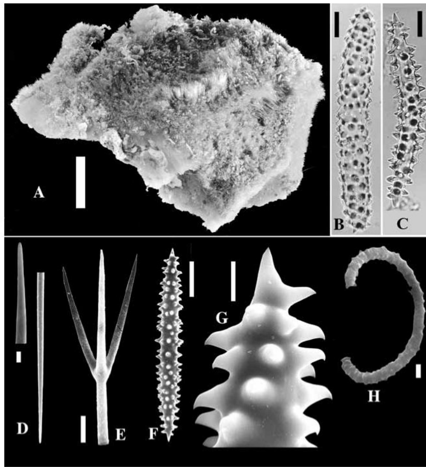
Fig. 1. Acanthotetilla spp. A–B, Acanthotetilla hemisphaerica Burton, 1959a. A, holotype BMNH 1936.3.4.530 (scale 1 cm). B, megacanthoxea of holotype (scale 50 \mu\text{m} ). C, Acanthotetilla enigmatica (Lévi, 1964b as Acanthocinachyra ), megacanthoxea (scale 50 \mu\text{m} ). D–H, Acanthotetilla gorgonosclera Van Soest, 1977b. D, oxea (scale 10 \mu\text{m} ). E, protriaene (scale 10 \mu\text{m} ). F, megacanthoxea (scale 50 \mu\text{m} ). G, detail of same (scale 10 \mu\text{m} ). H, sigmaspire (scale 1 \mu\text{m} ).
