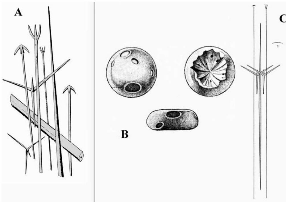
Fig. 8. Paratetilla bacca (Selenka, 1880) (scales see text). A, drawing of spicules reproduced from Selenka, 1867: fig. 15, as Stelletta . B–C, drawing of habit (B) and spicules (C) of Tetilla merguensis Carter, 1883a: pl. XV figs 6–8, considered a junior synonym.
