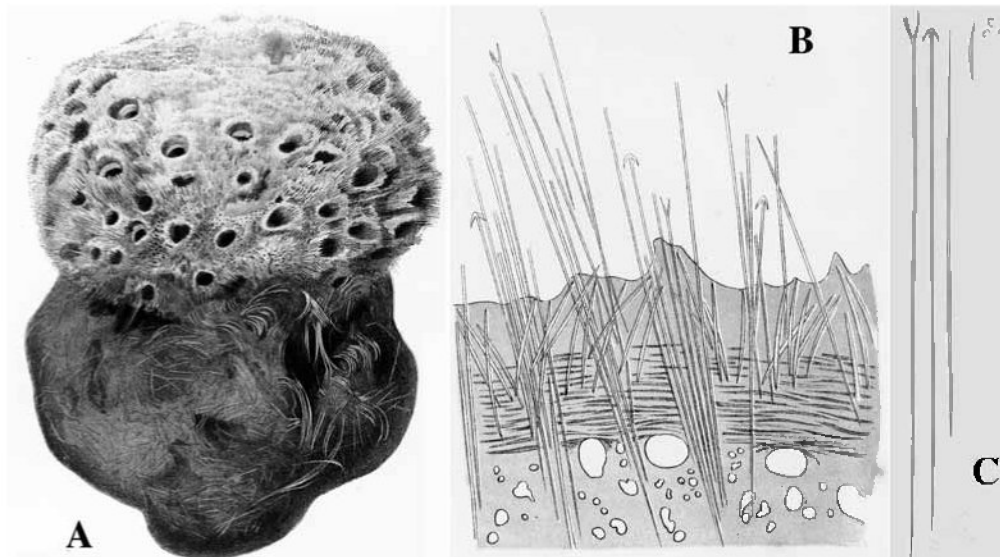
Fig. 3. Cinachyra barbata Sollas, 1888, drawing of habit (A), peripheral skeleton in cross section (B), and spicules (C), reproduced from Sollas' pl. III (scales see text).
