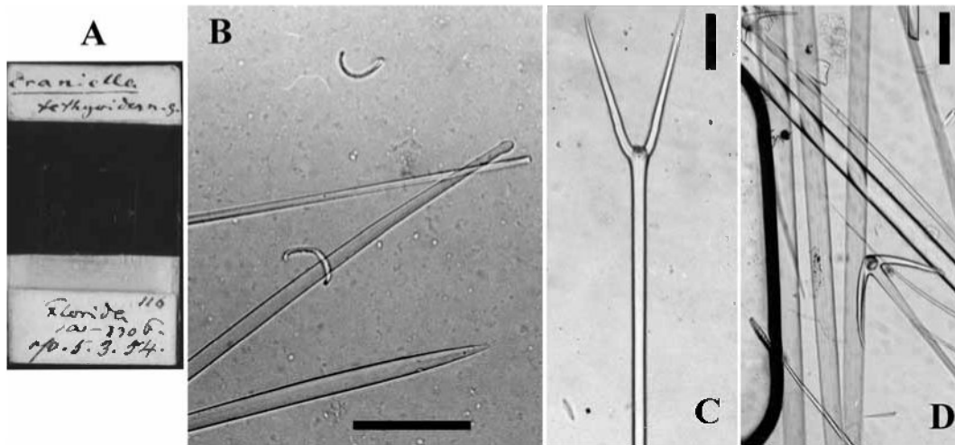
Fig. 6. Craniella tethyoides Schmidt, 1870. A, BMNH slide of lectotype. B–D, photos of spicules from lectotype (scales 50µm). B, sigmaspires. C, protriaene. D, anatriaenes.
