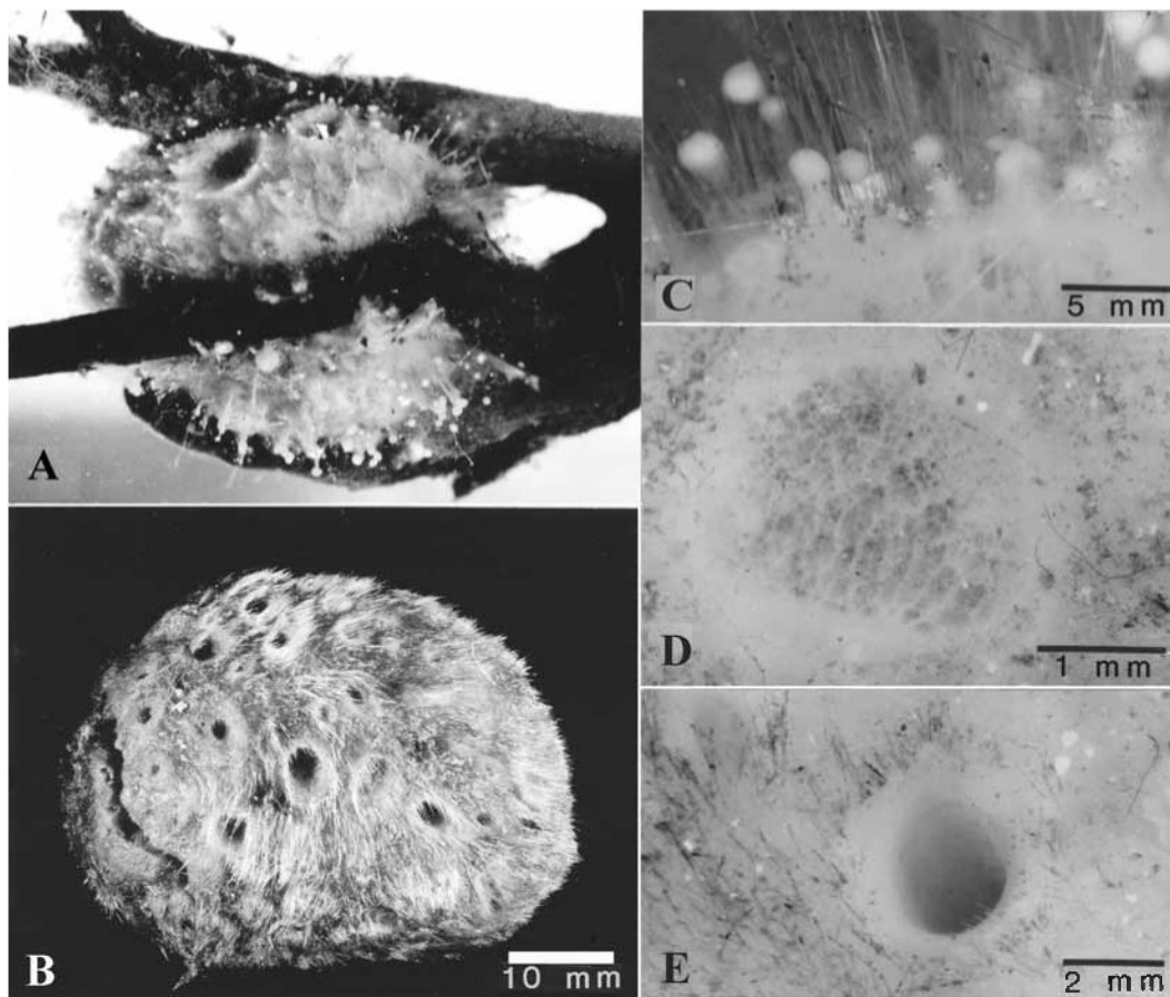
Fig. 4. Cinachyrella apion (Uliczka, 1929), habit and surface characteristics, reproduced from Rützler & Smith (1992: fig. 6). A, specimen in situ attached to alga, showing numerous buds. B, alcohol-preserved specimen. C, close-up of buds. D, close-up of porocalyx. E, close-up of oscule.
