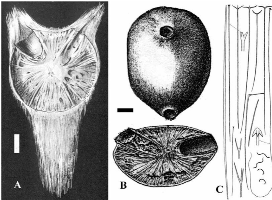
Fig. 7. Fangophilina species. A, Fangophilina submersa Schmidt, 1880b, drawing of cross section of holotype reproduced from Schmidt's pl. X fig. 3 (scale 1 cm). B–C, Fangophilina gilchristi (Kirkpatrick, 1902 as Spongocardium ). B, lectotype and cross section, reproduced from Kirkpatrick's pl. II fig. 1 (scale 1 cm). C, drawing of spicules from Kirkpatrick's pl. III fig. 1 (scale see text).
