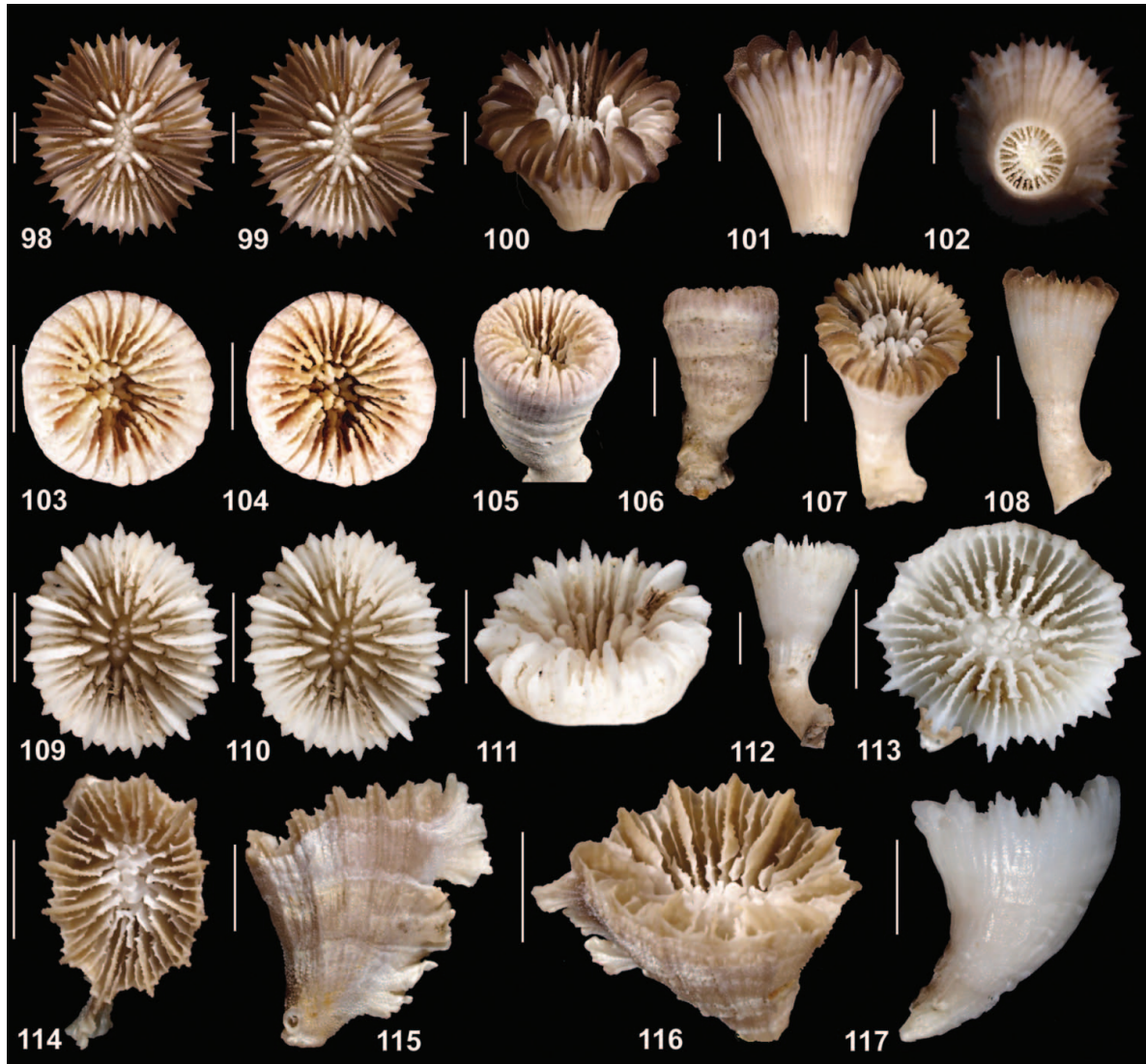
Figs 98–117. Caryophyllia sp. A (MNHN-IC.2009–0087): 98 and 99, stereo pair of calicular view; 100, oblique calicular view; 101, lateral view; 102, broken base view. Caryophyllia tangaroae sp. nov. (AM-G.17618–Holotype): 103 and 104, stereo pair calicular view; 105, oblique calicular view; 106, lateral view. Caryophyllia versicolorata sp. nov. (MNHN-IC.2009–0045–Holotype): 107, oblique calicular view; 108, lateral view. (MNHN-IC.2009–0053–Paratype): 109 and 110, stereo pair of calicular view; 111, oblique calicular view; 112, lateral view. Caryophyllia scobinosa (MNHN-IC.2009–0089): 113, calicular view; 117, lateral view. Caryophyllia unicristata (MNHN-IC.2009–0094): 114, calicular view; 115, lateral view; 116, oblique calicular view. Scale bars represent 5 mm.
